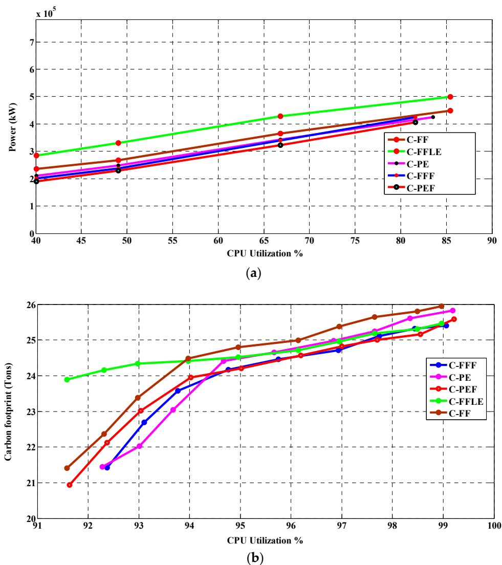
Figure 8. (a) Power consumption values with low utilization. (b) Carbon footprint values with high utilization. C-PEF and C-FFF are compared with other algorithms in terms of CPU utilization.
