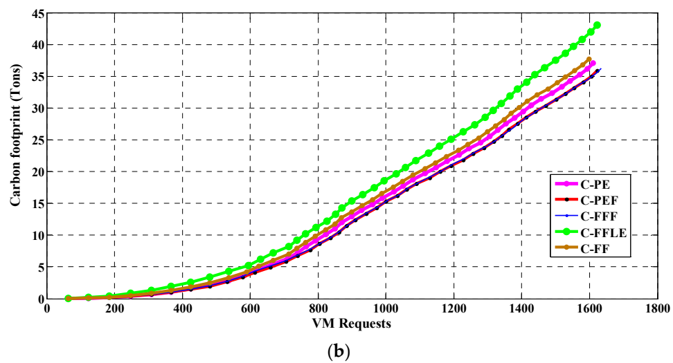
Figure 7. (a)Power consumption and (b) carbon footprint comparisons of all algorithms.
