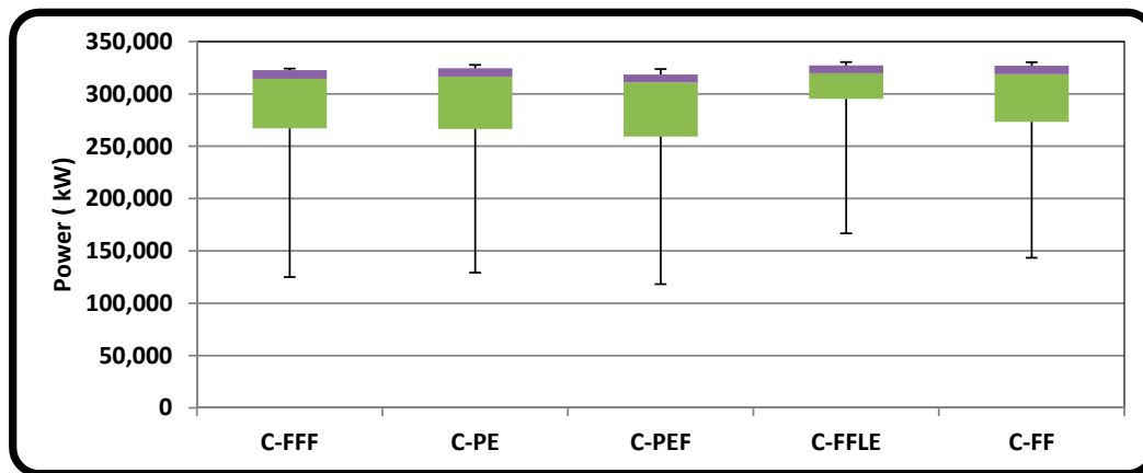
Figure 10. Power consumption.
