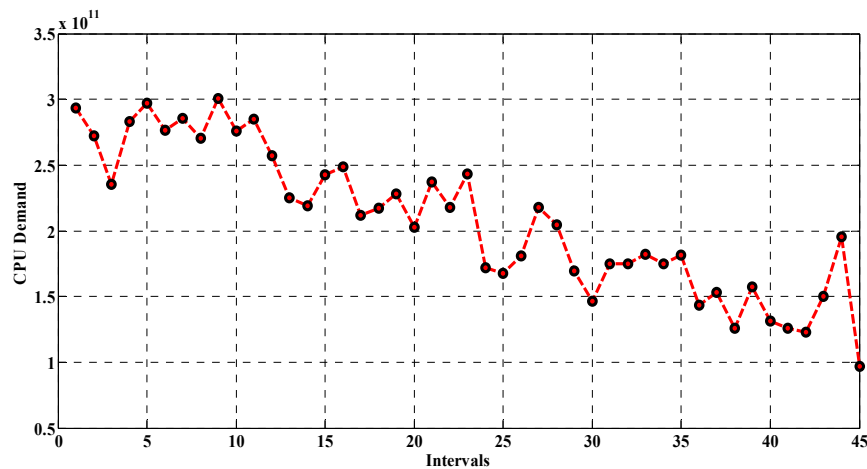
Figure 4. Processor demand at different intervals
