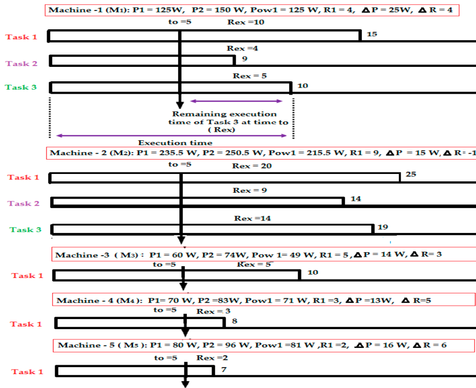
Figure 2. Host selection policy for carbon- and power-efficient optimal frequency (C-PEF).
