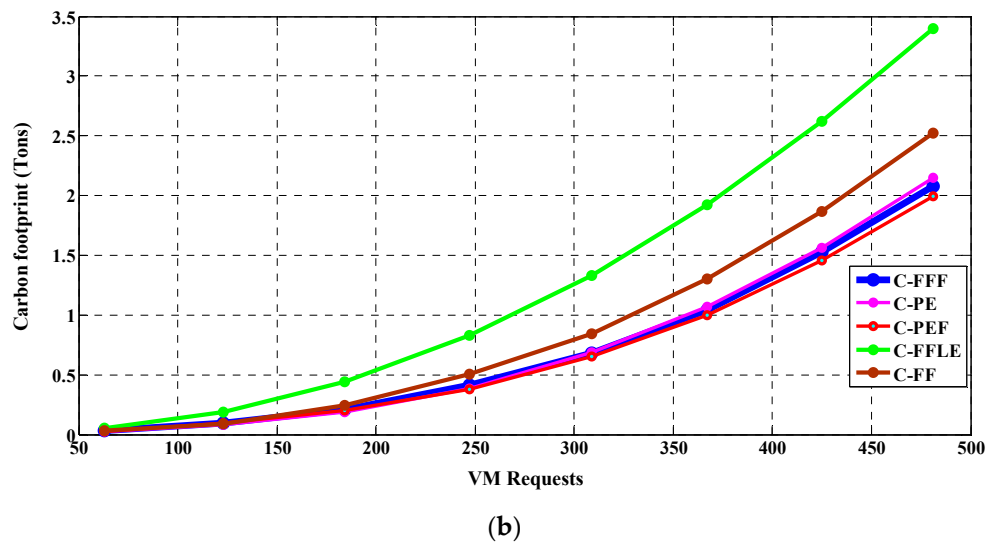
Figure 6. (a)Power consumption and (b) carbon footprint of all algorithms with 100% RVA.
