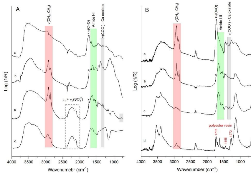
Figure S1. IR bands vibrational modes of the spectra acquired on different sampled paint fragments (see figure 8).
