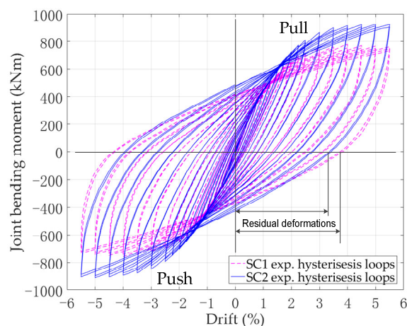
Figure 9. Hysteresis moment–drift response of specimens.
