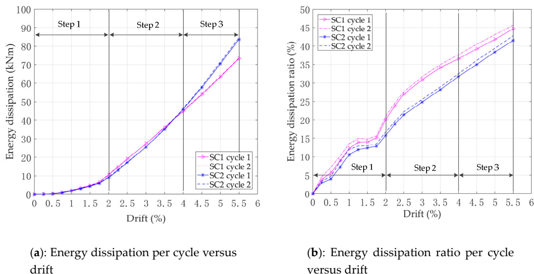
Figure 14. Energy dissipation for each cycle.
