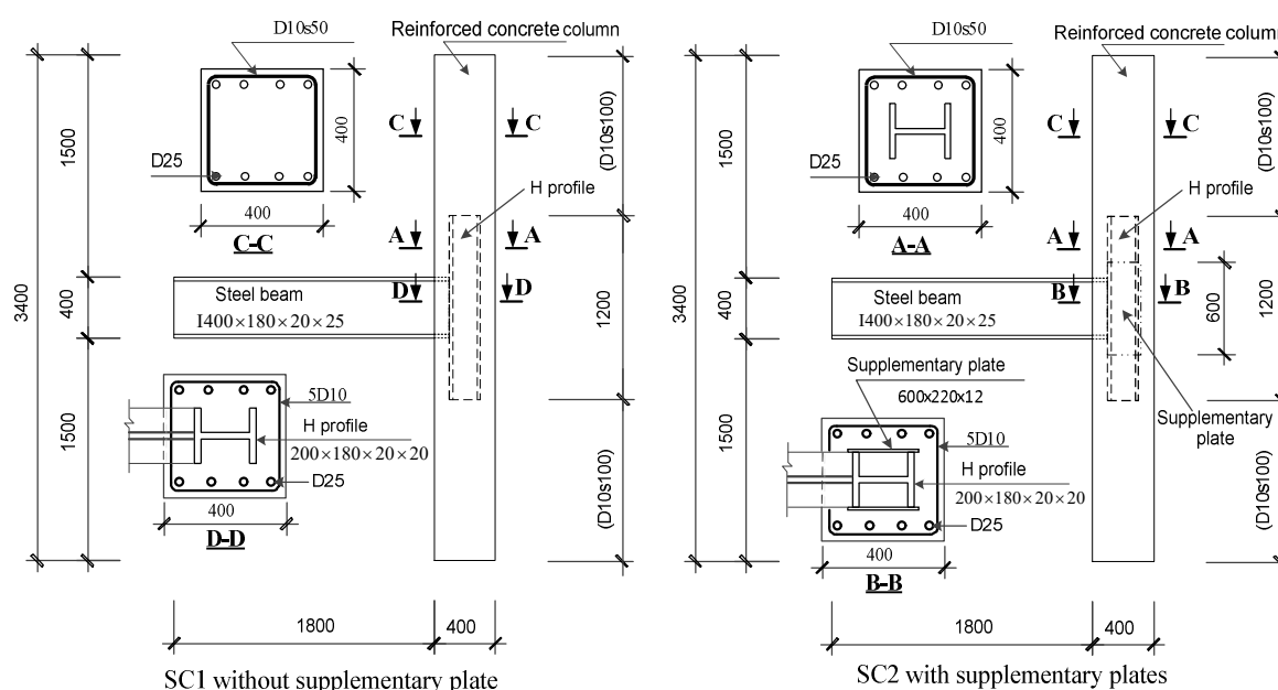
Figure 2. Description of the test specimens.
