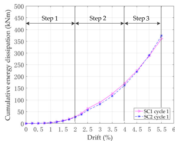
Figure 15. Cumulative energy dissipation versus drift.
