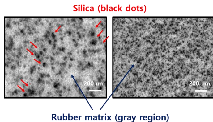
Figure S1. (left) TEM images of rubber composites with HCR. (right) TEM images of rubber composites with TPR.
