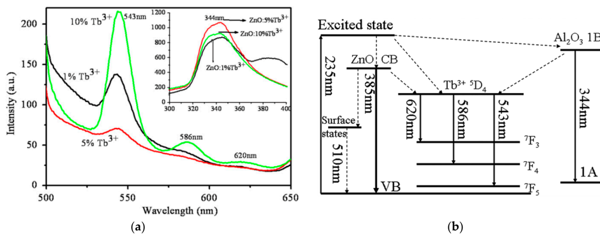
Figure 2. Photoluminescence properties of Tb-doped ZnO nanotubes. (a) Emission spectra of ZnO with different dopant levels excited by a 235 nm radiation; (b) energy-levels schematic with the electron transition processes in Tb-doped ZnO nanotubes grown onto alumina. Adapted from [114].
