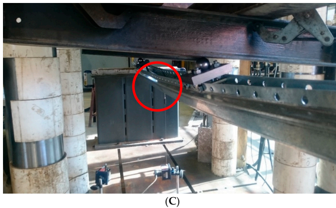
Figure 17. The observed failure mode for unreinforced specimens during the minor axis test: (A) SMIM-test1; (B) SMIM-test2; (C) SMIM-test3.
