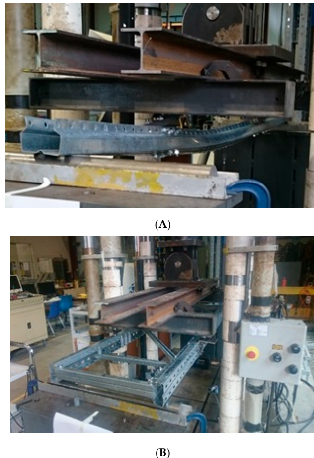
Figure 9. Test set-up: (A) minor axis test, (B) major axis test.
