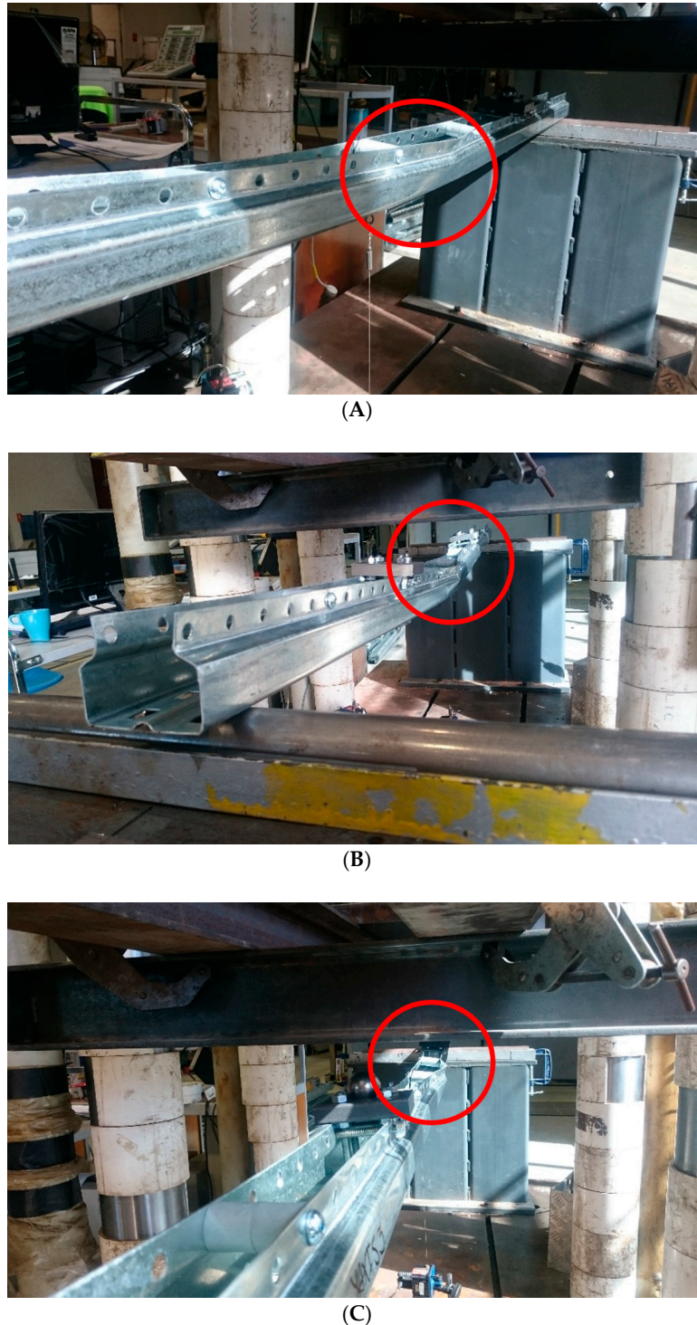
Figure 19. The observed failure mode for reinforced specimens with 300 mm reinforcing pitch during the minor axis test: (A) 300RMIM-test1; (B) 300RMIM-test2; (C) 300RMIM-test3.
