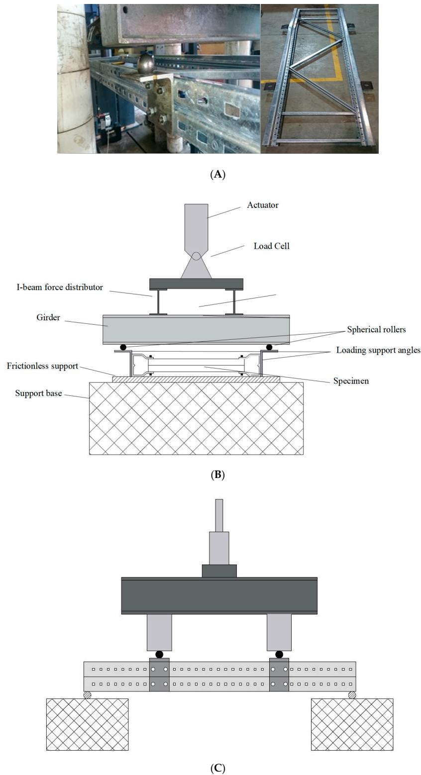
Figure 7. Major axis test set-up details: (A) Test specimen; (B) schematic front view; (C) schematic side view.
