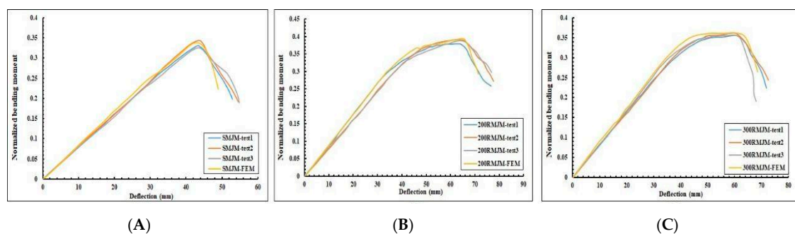
Figure 28. Finite element model and experimental curves for major axis test set-up: (A) non-reinforced frame types; (B) 200 mm reinforced frame types; (C) 300 mm reinforced frame types.
