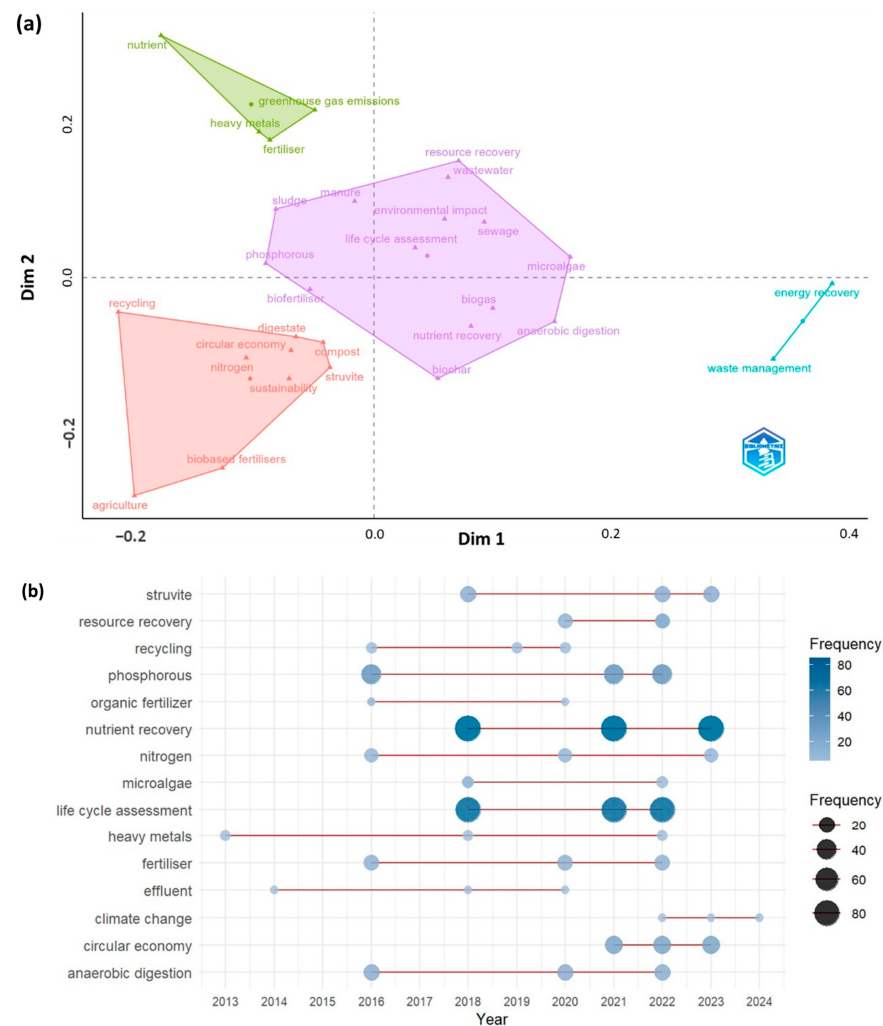
Figure 6. (a) Two-dimensional conceptual structure map based on multivariate analysis. The axes (Dim 1 and Dim 2) represent principal components capturing the highest variance in term co-occurrence.. Triangles represent keywords; proximity indicates co-occurrence. Colours show thematic clusters, and points mark central terms in each group. Dominant themes include nutrient recovery, recycling, circular economy, and waste valorisation. (b) Timeline of trend topics from 2013 to 2024. Circle size and color intensity represent the frequency of each term per year, revealing the evolution and prominence of key research topics over time.
