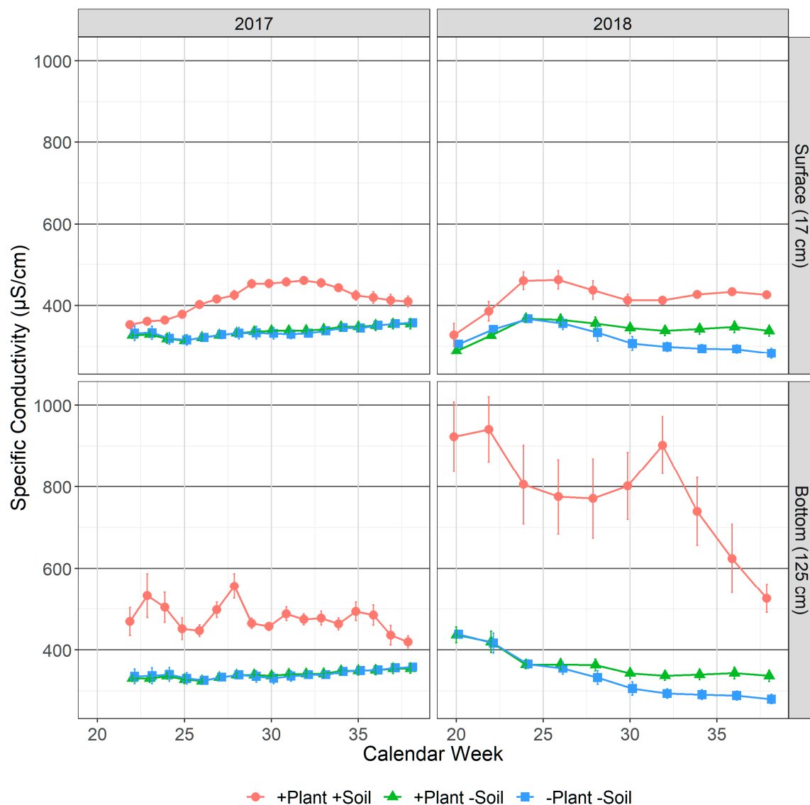
Figure 6. Mean specific conductivity readings from data sonde across depth and time in different groups (+Plant +Soil, n = 6 ; +Plant −Soil, n = 6 ; −Plant −Soil, n = 3 ). Error bars represent standard error.
