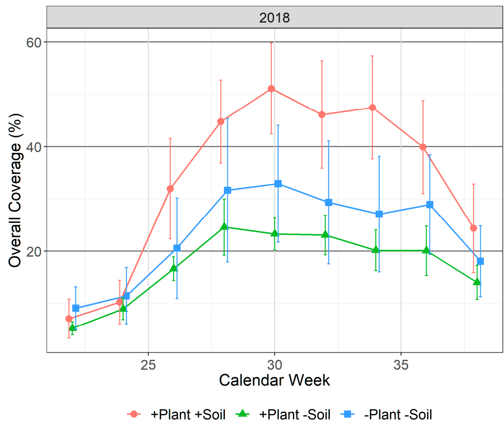
Figure 9. Mean estimated cover of phytoplankton/metaphyton over time with (+Plant +Soil, n = 6 ) or without soil (+Plant –Soil, n = 6 ; –Plant –Soil, n = 3 ) during 2018. Error bars represent standard error.
