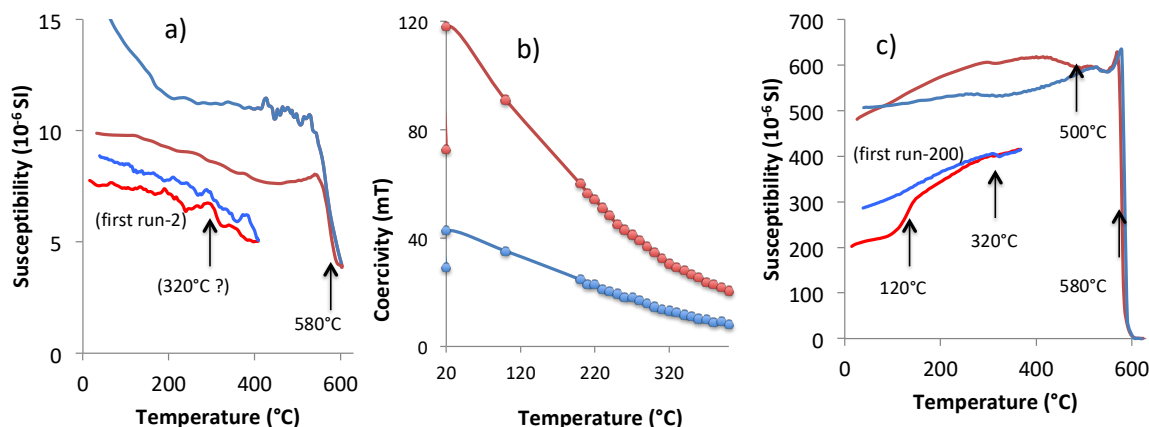
Figure 5. High temperature data for Popigai glasses: (a) sample PO-7 susceptibility versus temperature; (b) sample PO-7, B_{CR} (red), B_C (blue) as a function of temperature during heating; second lower value at room temperature (RT) corresponds to remeasure after heating cycle; (c) sample PO-23 susceptibility versus temperature. Heating and cooling curves in a) and (c) are indicated in red and blue, respectively.
