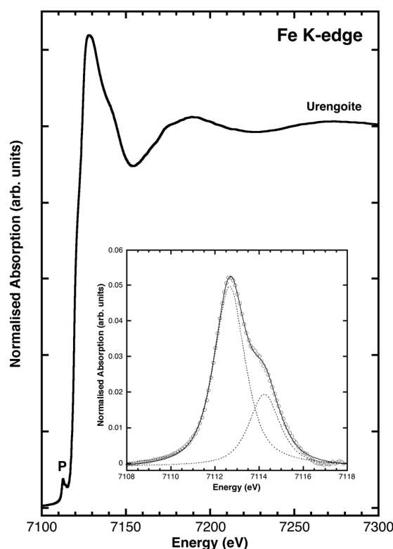
Figure 8. Fe K-edge XANES spectra of urengoite U1; background subtracted pre-edge peak (labeled P in the XANES spectrum) shown in the inset.
