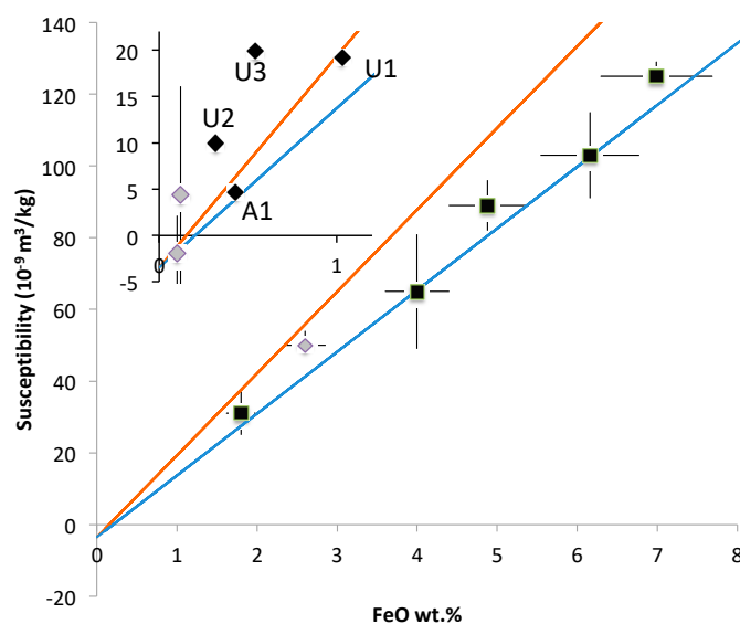
Figure 2. Magnetic susceptibility versus iron amount for tektite (black) and Darwin glass (grey), with theoretical curve for paramagnetic \text{Fe}^{2+} and \text{Fe}^{3+} (in blue and red, respectively), updated after [9]. Inset: iron poor glasses: LDG (grey), urengoite (U1, U2, U3), South-Ural glass (A1).
