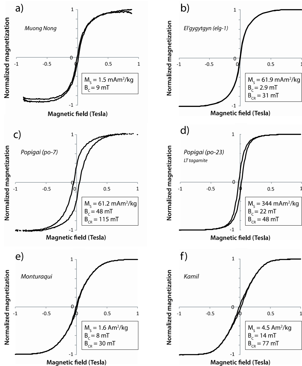
Figure 4. Examples of hysteresis loops, corrected for paramagnetism, obtained on impact glasses: (a) a titanomagnetite-rich Muong Nong tektite (note that strong paramagnetism prevented to obtain a well defined closed loop); (b) titanomagnetite-dominated El'gygytgyn glass; (c,d) pyrrhotite or magnetite-dominated Popigai glasses PO-7 and PO-23, respectively; (e,f) metal-bearing Monturaqui and Kamil glasses, respectively. LT tagamite is low-temperature tagamite (see Section 4.2.2).
