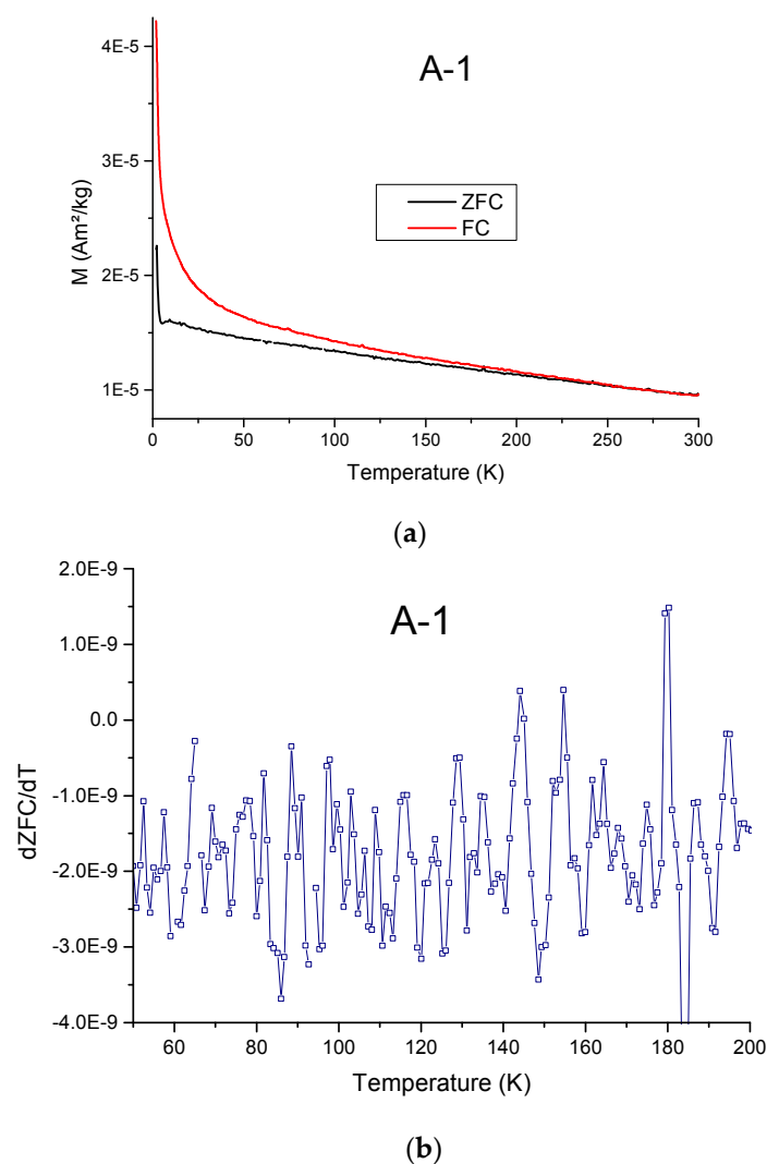
Figure 11. (a) Low temperature remanence data for South-Ural glass; (b) remanence derivative from (a) showing lack of transition.
