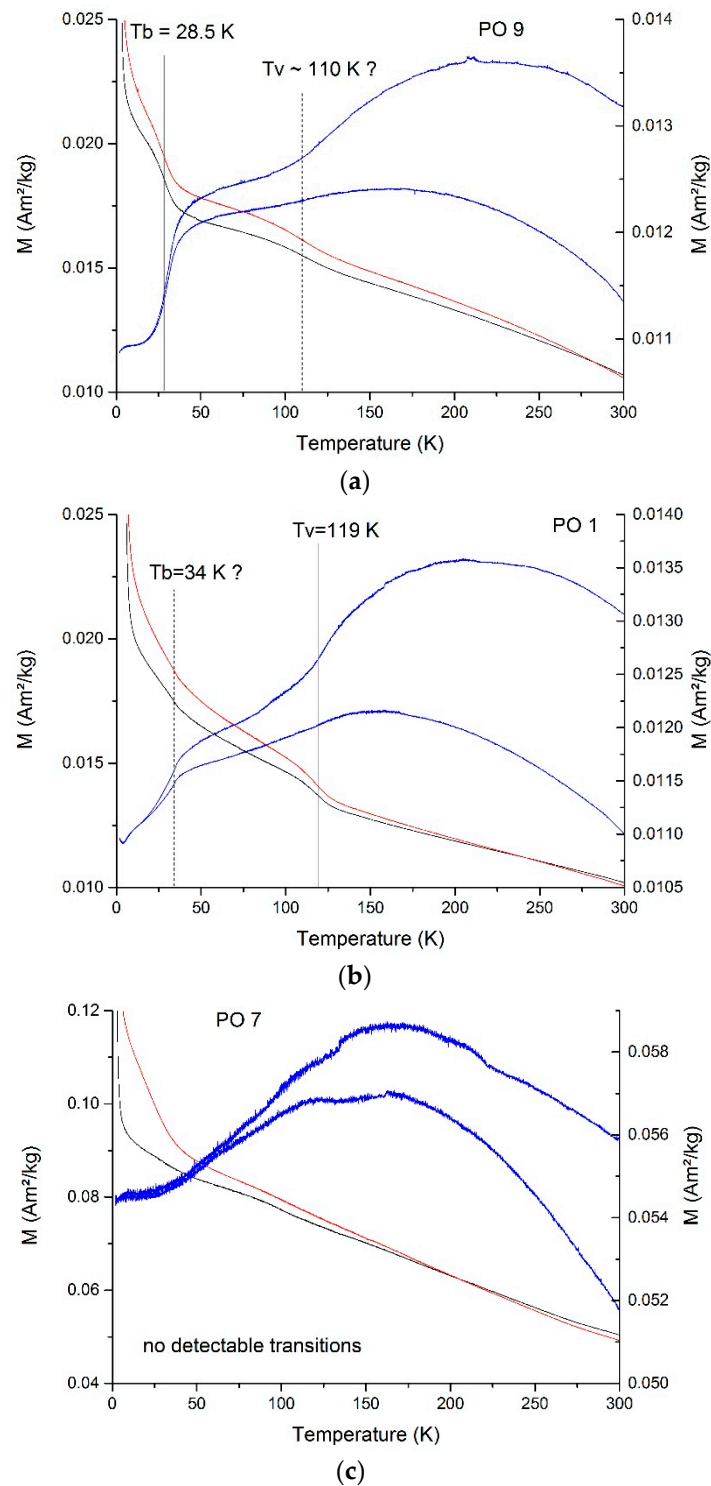
Figure 6. (a–c) Low-temperature properties of Popigai samples PO9, PO1, PO7. ZFC curves are shown in black, FC in red, room temperature SIRM cycle to 1.8 K in blue. ZFC and FC curves are shown above 10 K to emphasize Besnus and Verwey phase transitions. (a) and (b) show the samples with both Verwey and Besnus transitions, in variable proportion, (c) shows a sample with no detectable transitions. Where appropriate, transition temperatures are marked by vertical lines.
