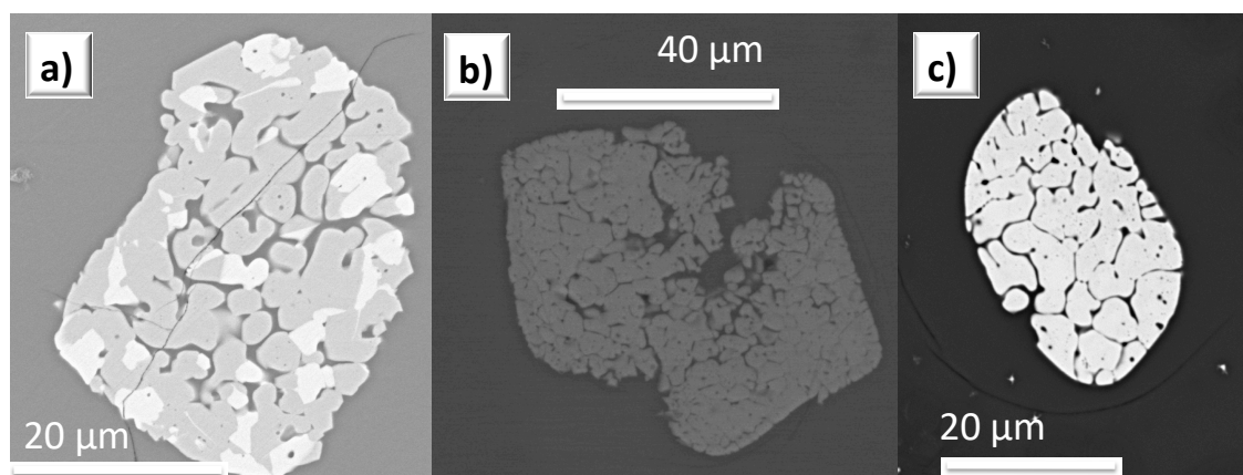
Figure 13. SEM back-scattered images of granular titanomagnetite in: (a) El'gygytgyn glass after [38]. Note that the darker phase is \text{TiO}_2 -rich; (b) irghizite from [12]; (c) Pantasma glass from [11].
