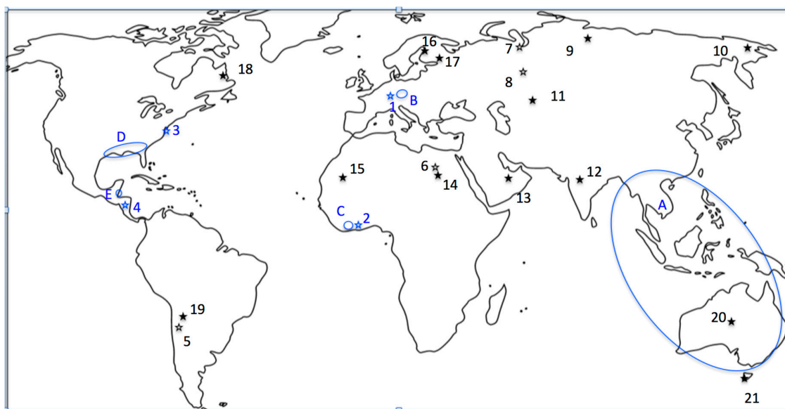
Figure 1. Map of tektite fields (blue contours: A—australasites; B—moldavites; C—ivoirites; D—bediasite-georgiites; E—belizites), craters of possible origin for tektites (blue star: 1—Ries; 2—Bosumtwi; 3—Chesapeake Bay; 4—Pantasma), other impact glasses without known source crater (black open star: 5—atacamaites; 6—LDG; 7—urengoites; 8—Ural glass) or with known source crater (black filled star: 9—Popigai; 10—El’gygytgyn; 11—irghizites; 12—Lunar; 13—Wabar; 14—Kamil; 15—Aouelloul; 16—Lapajarvi; 17—Janisjarvi; 18—Mistastin; 19—Monturaqui; 20—Henbury; 21—Darwin glass).
