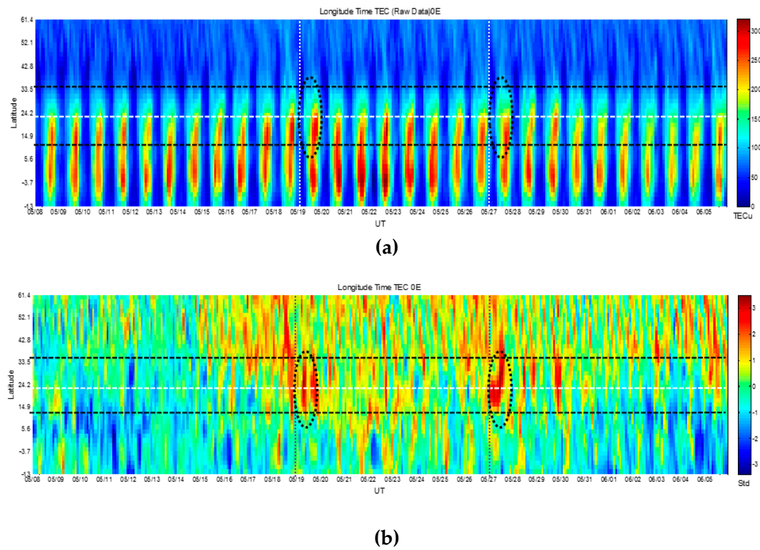
Figure 14. (a) Longitude–time–TEC (LTT) plots extracted from the global ionosphere map (GIM) along the 0° E longitude; (b) standardized plot. The mean is computed at each location and each time point for the observation period of 8 May–6 June 2008.
