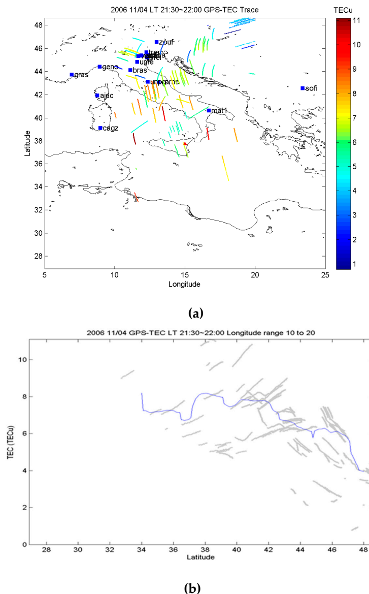
Figure 8. (a) Locations of 17 ground-based Global Positioning System (GPS) receivers (SOPAC, http://sopac.ucsd.edu/ ) and their GPS total electron content (TEC) ground traces during 9:30–10:00 p.m. on 4 November 2006. Blue squares and color curves in the top panel stand for the ground-based GPS receivers and the TEC at its associated ionospheric point, respectively. (b) GPS TEC variations along the volcano longitude during 9:30–10:00 p.m. LT on 4 November 2006. Grey and blue curves in the bottom panel denote the GPS TEC in the network and their median within 10–20 longitude (with a 0.1-deg latitudinal grid), respectively.
