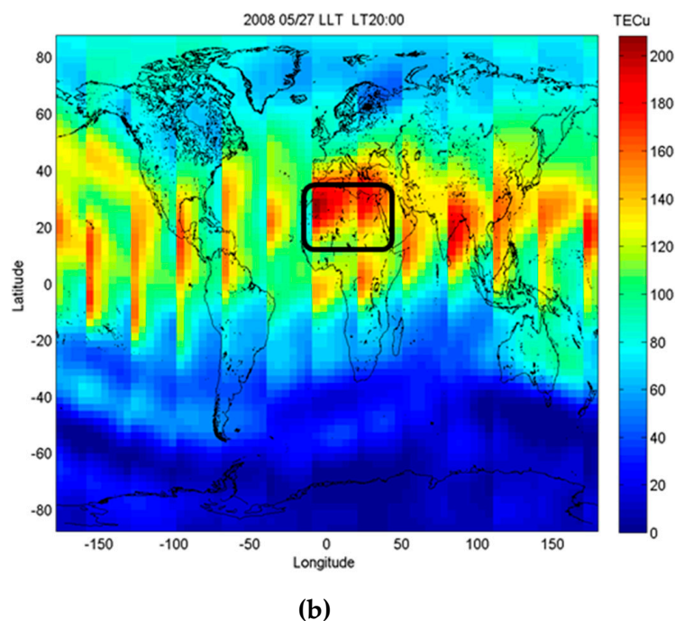
Figure 15. Latitude–longitude (LLT) maps at global fixed local time 8:00 p.m. LT extracted from the GIMs along various longitudes in reference to: (a) 19 May 2008; (b) 27 May 2008.
