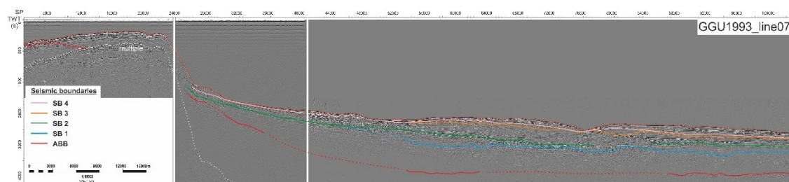
Figure S6. Seismic across slope profile. Its location is shown in Supplementary Figure S2.
