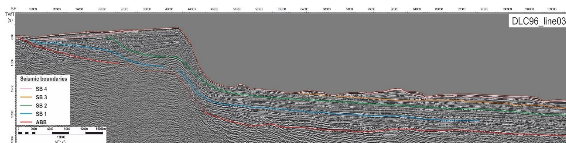
Figure S5. Seismic across slope profile. Its location is shown in Supplementary Figure S2.
