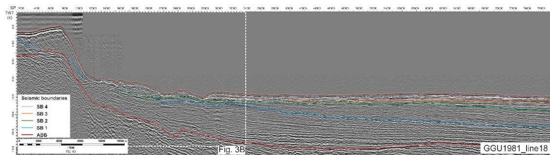
Figure S7. Seismic across slope profile. Its location is shown in Supplementary Figure S2.
