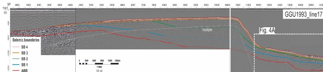
Figure S4. Seismic across slope profile. Its location is shown in Supplementary Figure S2.
