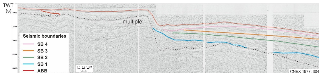
Figure S9. Seismic across slope profile. Its location is shown in Supplementary Figure S2.
