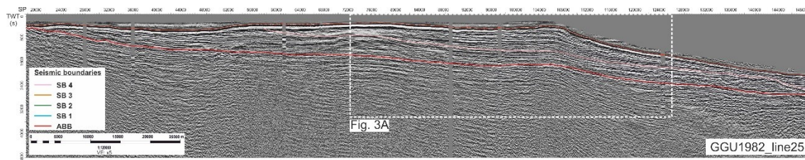
Figure S3. Seismic across slope profile. Its location is shown in Supplementary Figure S2.
