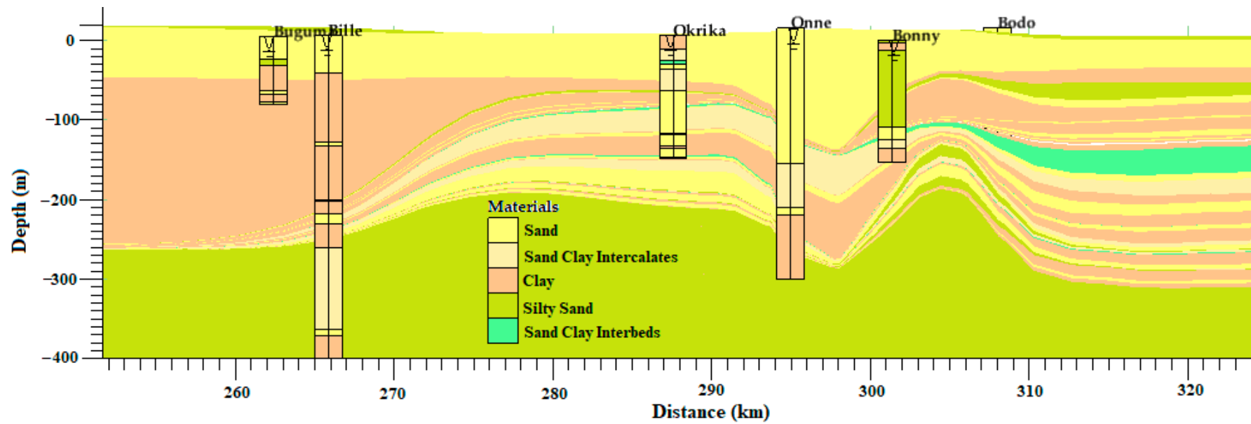
Figure 6. Hydrostratigraphic section along profile line DD I at various zones within the Niger Delta basin.
