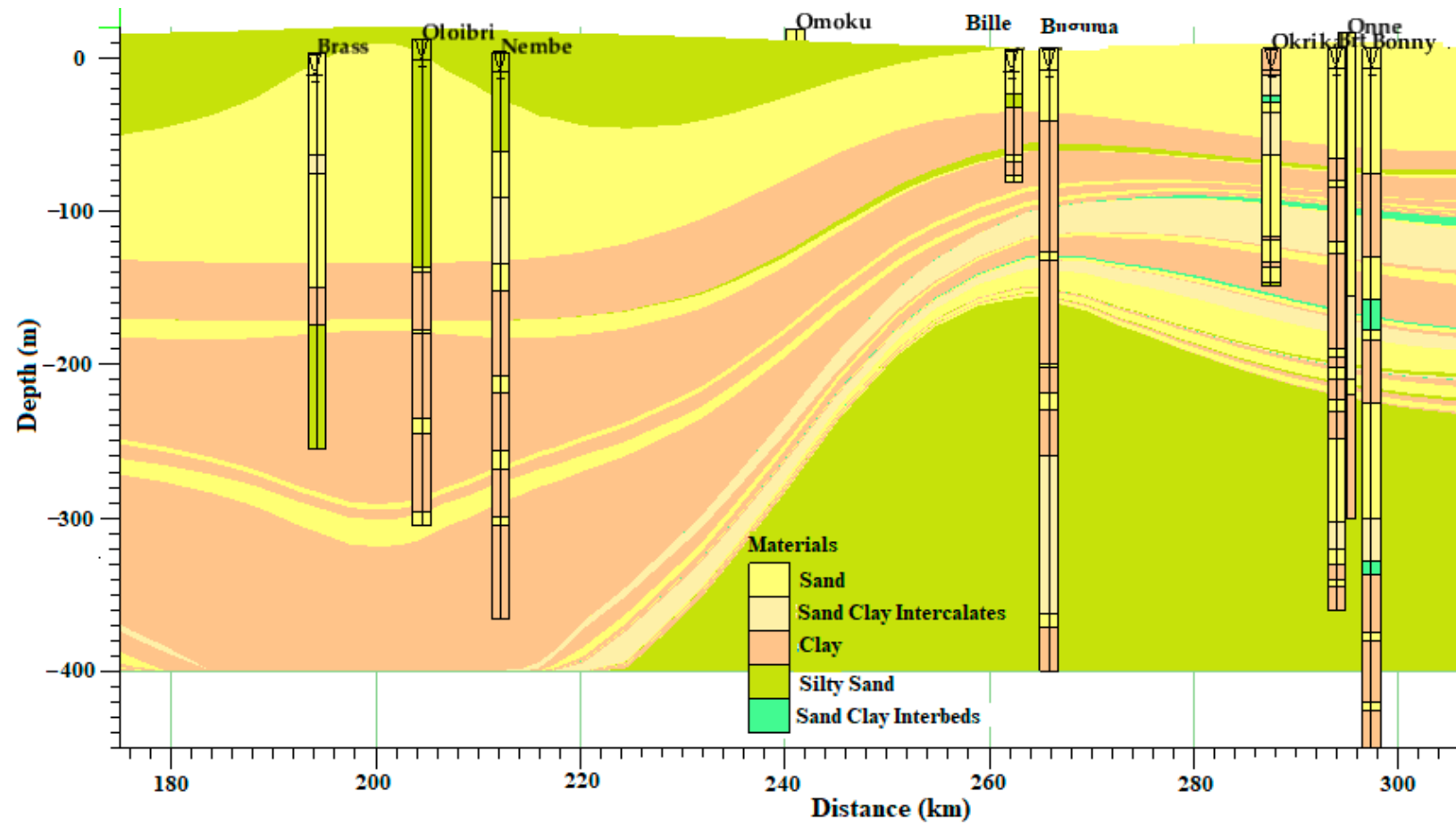
Figure 4. Hydrostratigraphic section along profile line BB I at various zones within the Niger Delta basin.
