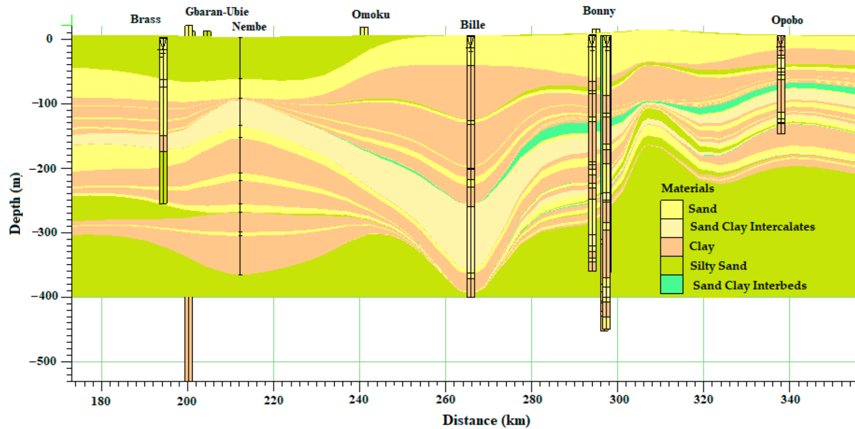
Figure 3. Hydrostratigraphic section along profile line AA I at various zones within the Niger Delta basin.
