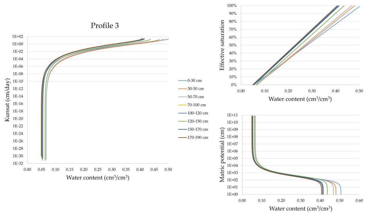
Figure 5. SWRCs, effective saturations, and unsaturated hydraulic conductivities in soil profile 3.
