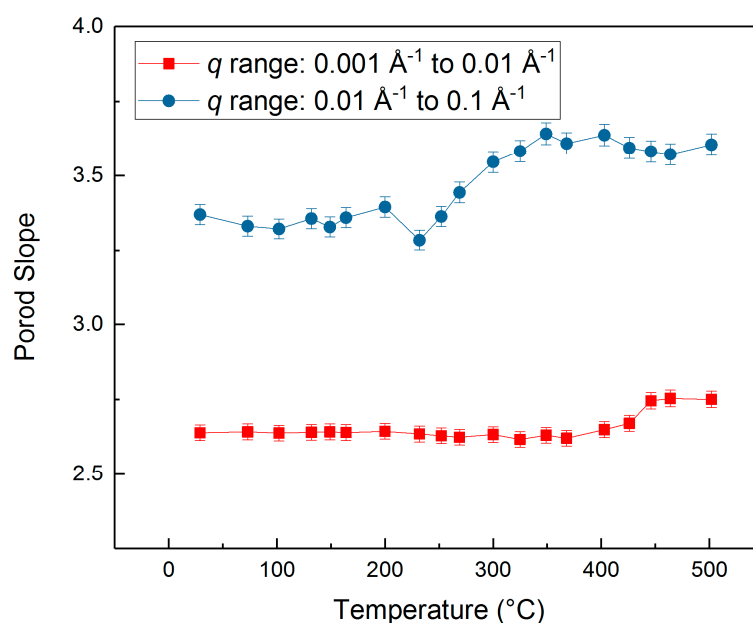
Figure 6. Porod slopes as calcium hydroxide is reacted with calcium carbonate are represented. Low q and high q ranges represent 0.001 to 0.01 \text{ \AA}^{-1} and 0.01 to 0.1 \text{ \AA}^{-1} , respectively. The data was obtained after desmearing the USAXS/SAXS data shown in Figure 5. Porod slope of 1 and 4 indicated scattering from rigid rods and smooth surfaces, respectively. Porod slopes in the range of 2 to 3 and 3 to 4 are indicative of branched systems or networks also known as mass fractals and rough interfaces with a fractal dimension, D where n = 6 - D represents a surface fractal.
