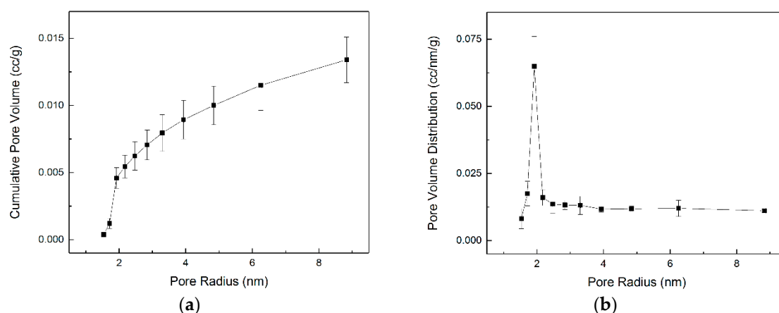
Figure 1. The cumulative pore volume (a) and pore volume distribution (b) of unreacted calcium hydroxide using Brunauer–Emmett–Taylor (BET) measurements.
