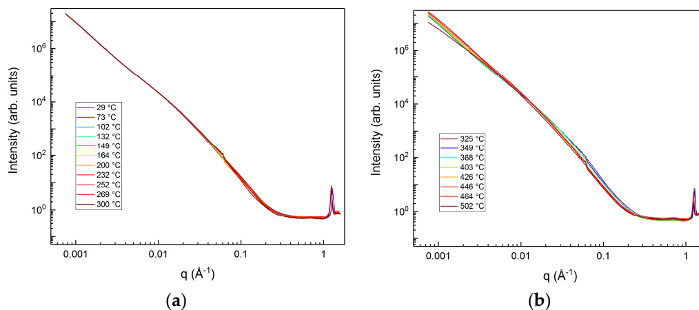
Figure 5. Changes in the combined slit-smear USAXS/SAXS data as calcium hydroxide is reacted with CO 2 where (a) and (b) represent temperatures in the range of 29 to 300 °C and 325 to 502 °C, respectively.
