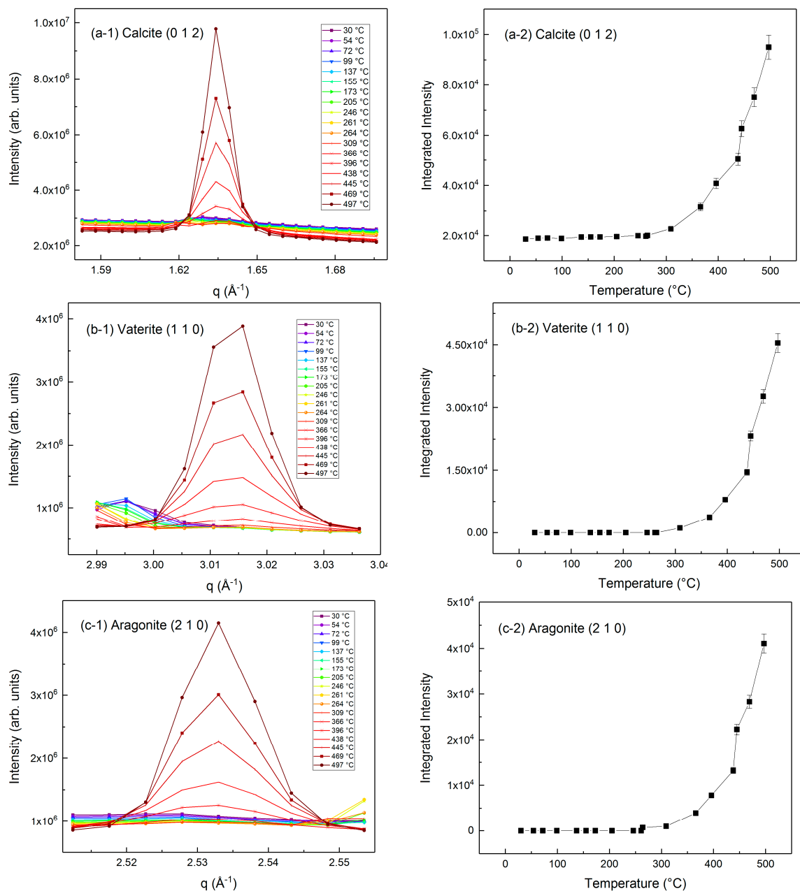
Figure 3. Changes in the characteristic carbonates peaks: calcite ( d = 3.85 Å, q = 1.63 Å -1 , h k l: (0 1 2)) [46] in (a-1), vaterite ( d = 2.08 Å, q = 3.02 Å -1 , h k l: (1 1 0)) [44] in (b-1), and aragonite ( d = 2.48 Å, q = 2.53 Å -1 , h k l: (2 1 0)) [45] in (c-1) as calcium hydroxide is reacted with CO 2 at reaction temperatures in the range of 30 °C to 500 °C. The integrated peak intensities of calcite, vaterite, and aragonite are shown in Figure 3 (a-2,b-2 and c-2) respectively. Vertical bars represent estimated 5% standard deviation uncertainties in Figure 3 (a-2,b-2 and c-2).
