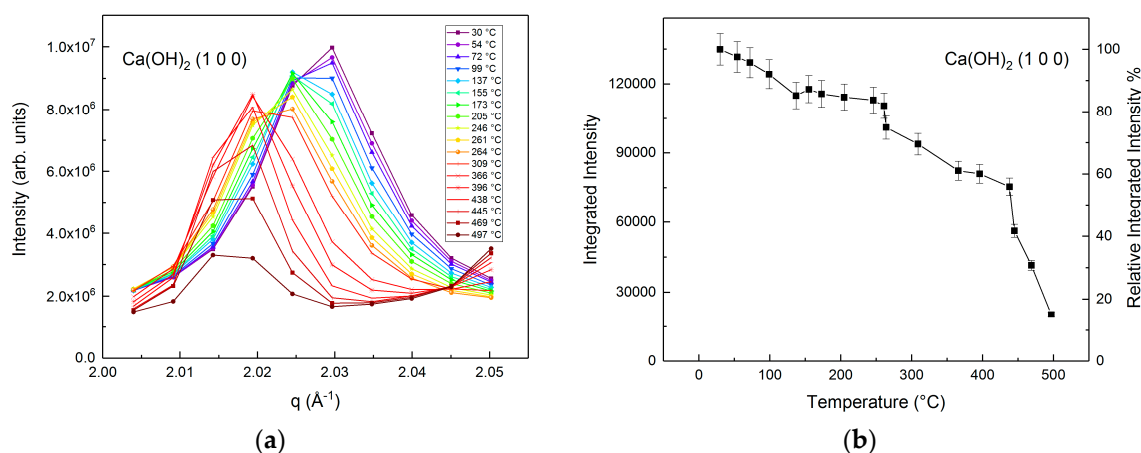
Figure 2. Changes in the characteristic peak of calcium hydroxide ( d = 3.105 Å, q = 2.024 Å -1 , h k l : (1 0 0)) and the integrated peak intensity are represented in (a) and (b), respectively [40]. The relative integrated intensity of calcium hydroxide represented in (b) is the integrated intensity of the characteristic peak at a given temperature normalized to the integrated intensity at 30 °C. Vertical bars in (b) represent estimated 5% standard deviation uncertainties.
