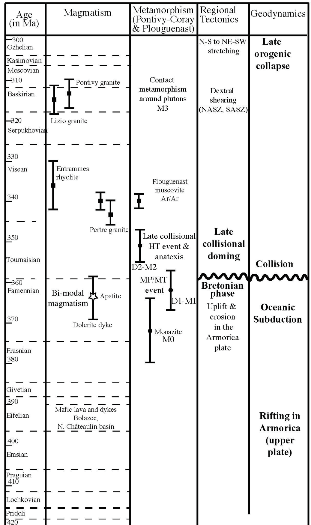
Figure 14. Synoptic chart of the metamorphic, magmatic, and tectonic events experienced in Armorica with radiometric ages provided in [59,60,78,82,102,104].
