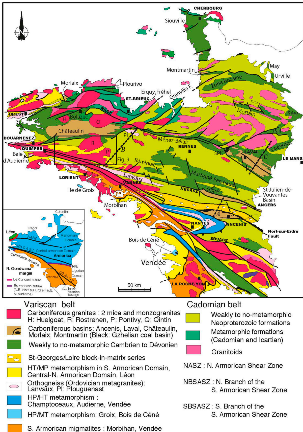
Figure 2. Structural map of the Armorican Massif with location of the study area (Figure 3) and trace of the three segments A, B, and C used to construct the synthetic general cross-section shown in Figure 13. Inset shows the subdivision of the Armorican Massif in three geodynamic domains, namely from north to south, the Léon, Armorica, and Northern Gondwana margin.
