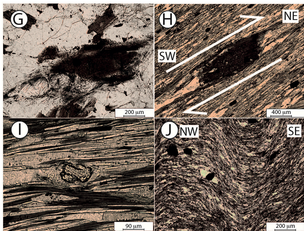
Figure 7. Thin section pictures. (A–F) images come from biotite–staurolite \pm garnet micaschists sampled within a few tenths of meters in the Evel valley (N47°53'16", W2°58'15.7"). (A): Staurolite with random quartz inclusions and asymmetric biotite pressure shadows indicating a top-to-the-NW shearing; (B): Same sample as A but cut perpendicular to the lineation showing a staurolite porphyroblast at high angle to the regional foliation; (C): Staurolite with quartz inclusion and biotite pressure shadows indicating a top-to-the NW sense of shear; (D): Staurolite with quartz inclusion defining a folded internal foliation unrelated with the regional one, suggesting the existence of an earlier foliation. Note the sharp boundary in the bottom of the staurolite grain; (E): Small-sized staurolite grain parallel to the regional foliation; (F): Garnet porphyroblast with randomly arranged quartz inclusion without internal foliation. (G): Biotite–muscovite–fibrolitic sillimanite micaschist (S. of St-Caradec, N48°1'35", W3°20'48"); (H): Sigmoidal biotite showing a dextral sense of shear consistent with the Armorican shear zone (N48°51'35", W3°38'21"); (I): Kyanite relict indicative of an earlier metamorphic event of higher pressure conditions than the main barrowian one. The grain is surrounded by a sericite halo elongated in the NS-SW direction (N47°53'16.5", W2°58'16"); (J): Crenulated biotite–chlorite micaschist, observed in XZ section. The folded foliation contains opaque minerals fringed by quartz pressure shadows (Cléguerrec, N48°7'6", W3°5'13"; see also Figure 7).
