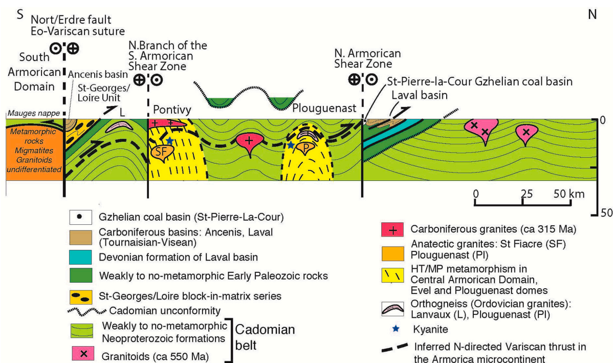
Figure 13. Interpretative crustal-scale cross-section of Central Brittany with emphasis on the Late Devonian N-directed thrusting coeval with kyanite crystallization and subsequent HT metamorphism and crustal melting.
