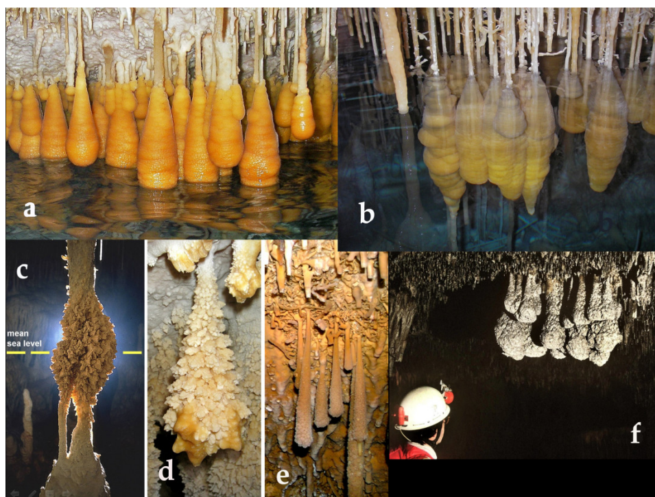
Figure 4. Photos of phreatic overgrowth on a speleothem (POS) in Mallorca. (a,b) : Modern aragonite POS at Cova des Pas de Vallgornera (Llucmajor, Mallorca). Photos by Tony Merino and Bogdan P. Onac. (c) POS at +2.6 m in Cova des Pas de Vallgornera (Llucmajor, Mallorca), dated to MIS 5.5. Photo by Tony Merino. (d,e) Some POS at Cova des Pas de Vallgornera (Llucmajor, Mallorca). Photos by Bogdan P. Onac. (f) Ancient POS at Coves del Drac (Manacor, Mallorca). Photo by Joaquín Ginés. Rumena cave (Custonaci, Trapani, [6]): A single stalactite was collected at 98 m above sea level within a small cave. Unlike most of the other speleothems from the Mediterranean, which are covered by serpulids, the stalactite from the Rumena cave has been encrusted by scleractinian corals (Figure 5g,h). The cross section of the sample revealed the presence of four highstands (MIS 25–37), with the outermost coral overgrowth, which represents the final marine ingress, being dated to 1.12 \pm 0.2 Myr through the strontium isotopes ( ^{87}\text{Sr}/^{86}\text{Sr} ) method.
