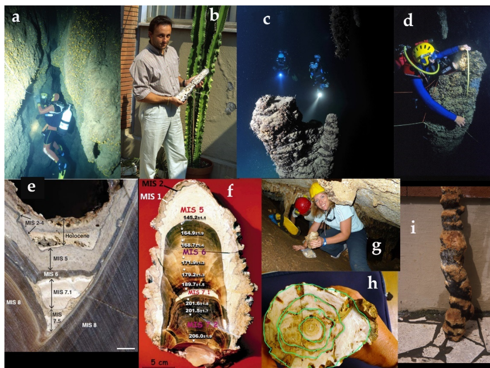
Figure 5. Coastal caves and submerged speleothems from Italy. (a): Sampling survey at -27 m in the Scaletta cave (Palinuro). (b) Prof. Marco Oliverio (Sapienza University) carrying the stalagmite collected at -48 m in the Scaletta cave (Palinuro). (c,d) Argentarola cave and a large stalagmite covered by serpulid overgrowth. (e) Stalagmite ASN collected at -18 m in the Argentarola cave. The 6 cm portion of the stalagmite covers the last 280 kyr, from MIS 8 to MIS 1 [18]. (f) Stalagmite ASL collected at -18.5 m in the Argentarola cave [2]. (g) View of the Custonaci cave. (h) Stalactite collected at +98 m in the Rumena cave, showing four marine highstands [6]. (i) Stalactite collected at -53 m in the Nettuno cave. Photo by F. Antonioli.
