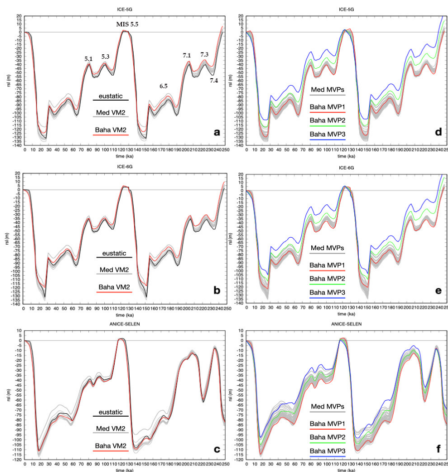
Figure 7. Cumulative predicted relative sea level (RSL) curves for ICE-5G (a,d), ICE-6G (b,e), and ANICE-SELEN (c,f) ice sheet models, in combination with different mantle viscosity profiles. The gray curves are for each site within the Mediterranean Sea, the red curves are for the Bahamas, and the black curves represent the eustatic signal (with respect to the present-day ocean function) for each ice sheet model.
