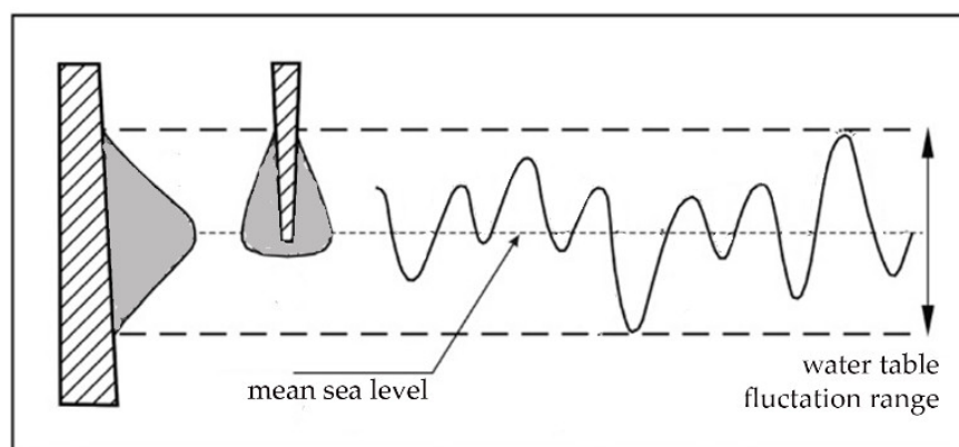
Figure A1. Tide amplitude and POS accretion, redrawn from [29].
