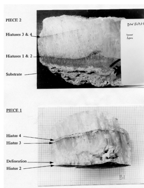
Figure 10. The DWBAH flowstone, sampled at −15 m on the Grand Bahama Island (courtesy of Joyce Lundberg).
