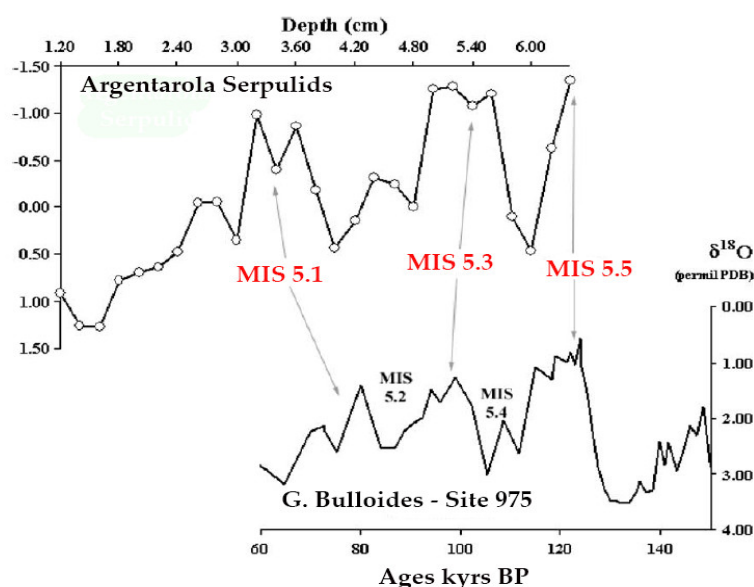
Figure 9. \delta^{18}\text{O} series of the marine layer of ASI (~18.5, MIS 5.5), compared with ODP 975 (Central Mediterranean sea) (redrawn from [21]).
