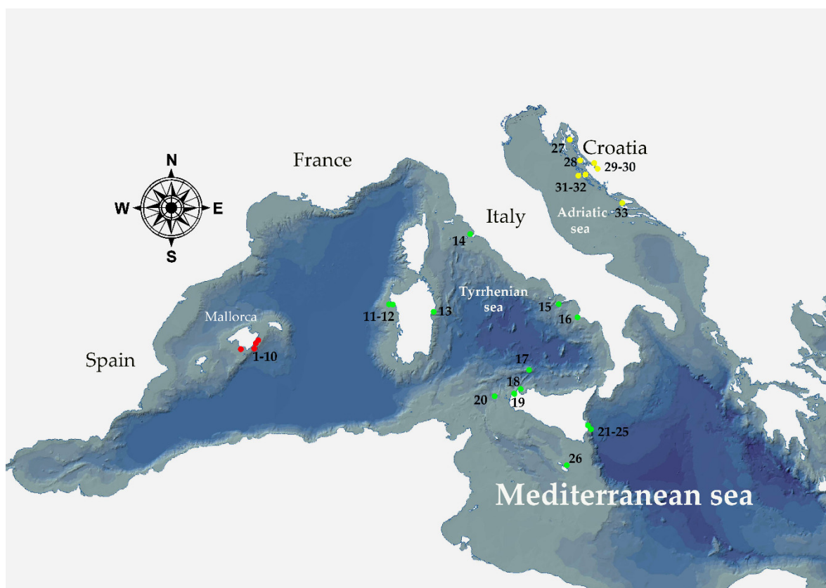
Figure 1. Overview map of the Mediterranean region showing the locations of the coastal caves discussed in this study. Specific information (latitude, longitude, sampling depths, dating method, and ages) is reported in Table 3 and 4.
