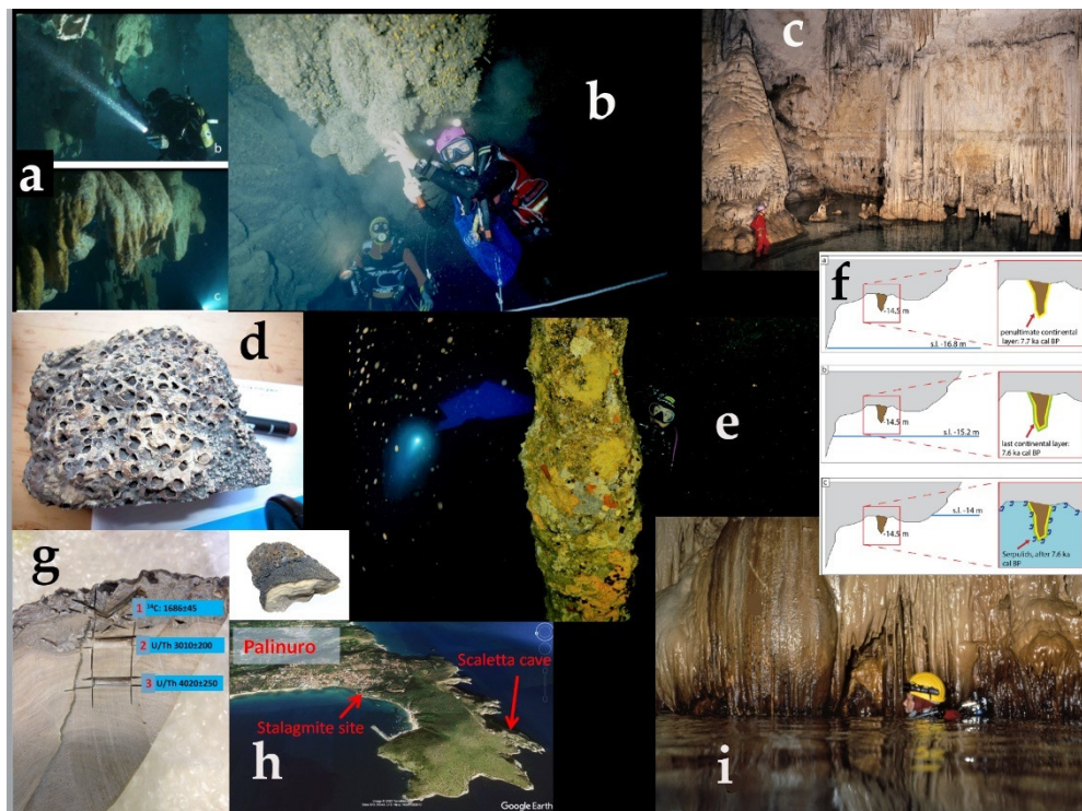
Figure 2. Coastal caves and submerged speleothems in Italy and Malta. (a) Stalactites sampled at −14 m in Malta. (b) Sampling survey conducted at −41 m in the Scaletta cave (Palinuro) by F. Antonioli, L. Ferranti, and M. Oliverio. (c) Oxidation bands observed at +4 m in the Nettuno cave and phreatic speleothems (photo by Mauro Mucedda). (d) and (e) Stalagmite collected in Palinuro encrusted by specimens of the barnacle Chthamalus . Cross section of the sample showing the portions collected for ^{14}\text{C} and U-series disequilibrium dating. (f) Cattedrale cave (Marettimo Island). (g) Growth model of the stalactite sampled in the Gebel Ciantar cave in Malta [65]. (h) Photo of the Palinuro promontory with the sampling sites of Scaletta cave and the stalagmite with barnacle overgrowth. (i) Risorgenza di Cala Luna cave. Photo by F. Antonioli.
