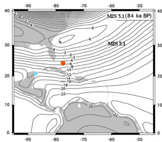
Figure A2. GIA for Caribbean Islands and Florida (redrawn from [39]).
