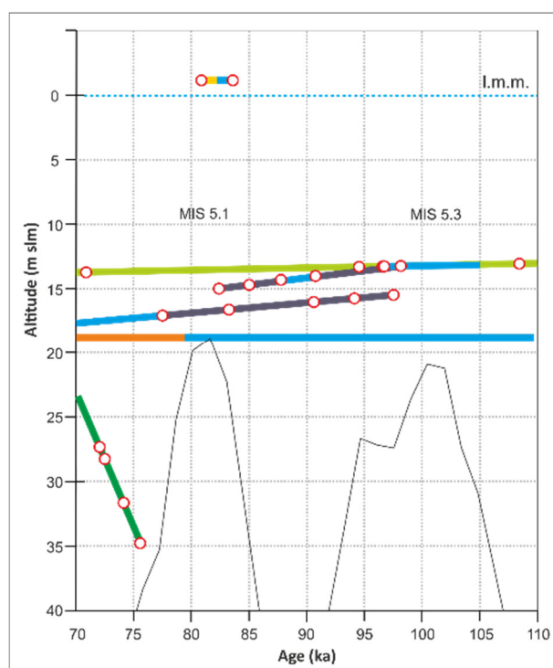
Figure 14. Zoom 1 of Figure 15. Light green line: DWBAH flowstone [11]; orange line: Stalagmite ASI (−18.5) from Argentarola cave, −18.5 m [2]; black line: Speleothems K14 and K18; yellow and blue line: Mallorca POS; green line: Plemmirio [64]; fine black line: global sea level curve reconstructed by [88].
