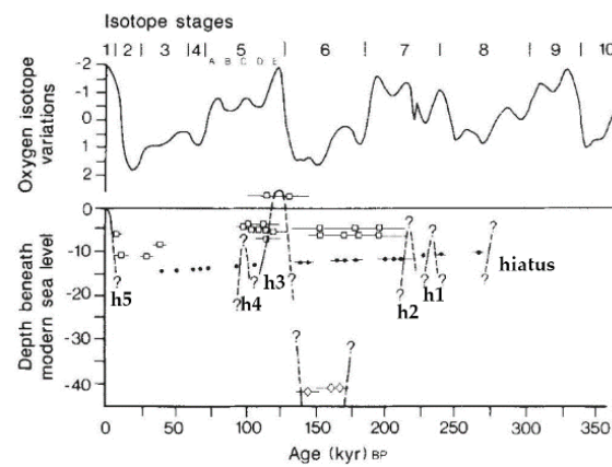
Figure A3. U-Th ages vs. the sampling depth of the flowstone DWBAH (redrawn from [1]).
