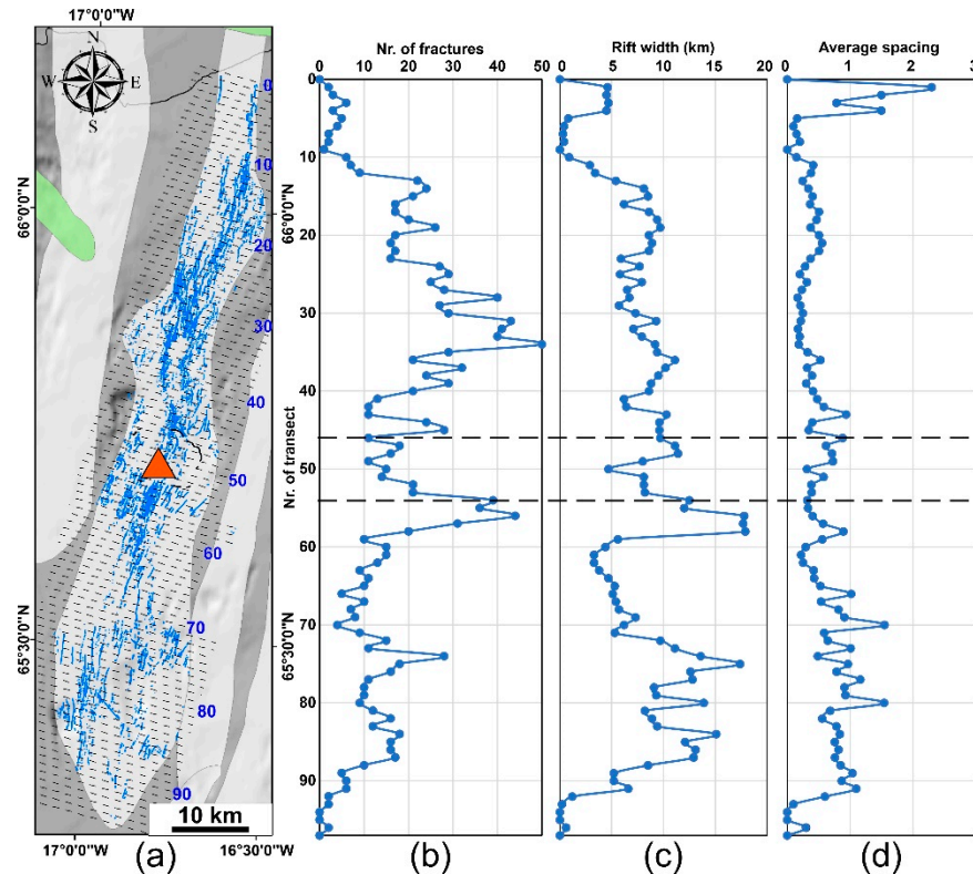
Figure 9. (a) Map representing all the structures of the KFS and the location of the central volcano. Black dashed lines show the N106°E-striking transects. Graphs showing (b) the number of total structures, (c) rift width and (d) the average spacing measured along the transects considering the whole structures. Black dashed lines in the graphs show the location of the Krafla caldera.
