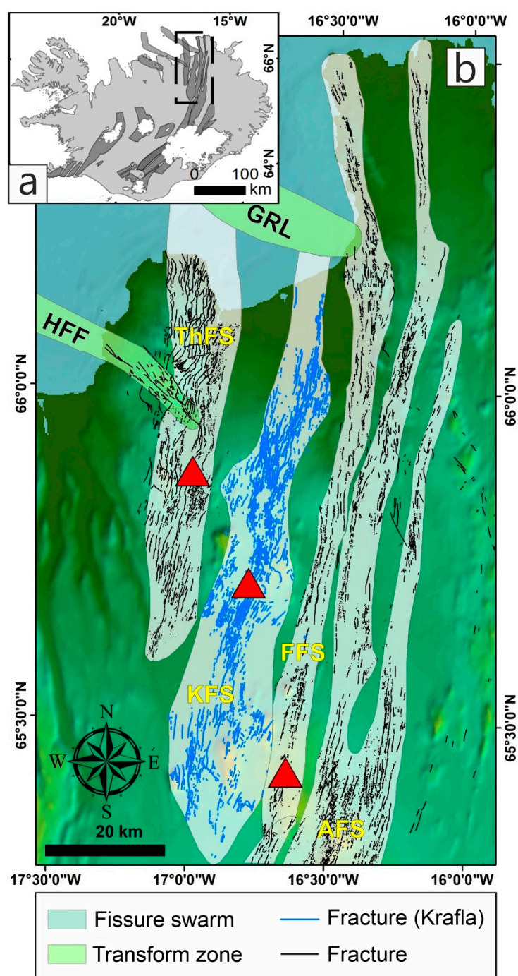
Figure 1. (a) Volcanic systems of Iceland, with the main volcano-tectonic rift zones of Iceland (darker grey areas, after Einarsson and Saemundsson [11]; Hjartardóttir et al. [1]): the black rectangle indicates the Northern Volcanic Zone (NVZ); (b) Map of the NVZ with all the structures and central volcanoes. Light green areas represent the transform zones, whereas light blue areas represent the fissure swarms of the region, where all the structures are shown (after Magnúsdóttir and Brandsdóttir [12]; Hjartardóttir et al. [1,13]); the KFS structures are highlighted in blue. AFS: Askja Fissure Swarm; FFS: Fremrinamar Fissure Swarm; HFF: Husavik Flatey Fault; GRL: Grimsey Lineament; KFS: Krafla Fissure Swarm; ThFS: Theistareykir Fissure Swarm.
