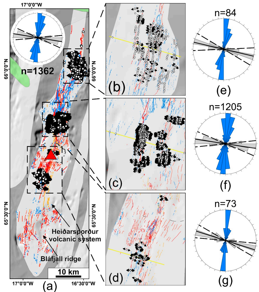
Figure 13. (a) Map of the KFS, same scale and north of Figure 9a, showing as white dots the location of all the structural measurements collected in the field. Rose diagram shows the 1362 opening directions (grey) and the local azimuth values (blue) of the extension fractures. The opening directions are represented by black diverging arrows. The three areas are shown more in detail in (b,c,d), with their respective rose diagrams in (e,f,g). Yellow lines in (b,c,d) represent the three N106°E- oriented transects; the continuous black lines in the rose diagrams represent the average values; dashed lines represent the standard deviation.
