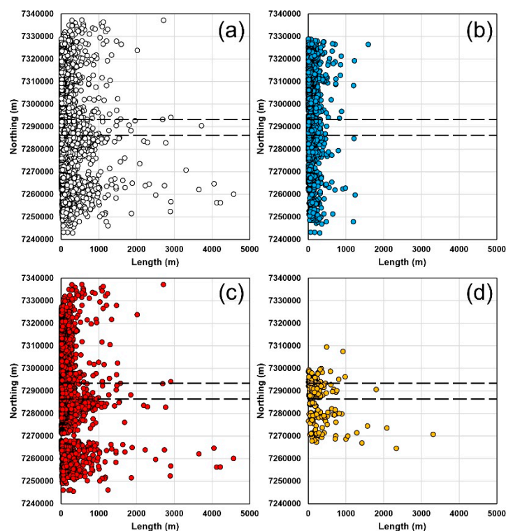
Figure 5. Graphs showing length values for the whole fractures set (a), extension fractures (b), normal faults (c) and eruptive fissures (d) subsets with respect to the north. The northing is re-reported in the WGS84-UTM Zone 28N reference system. Black dashed lines show the location of the Krafla caldera.
