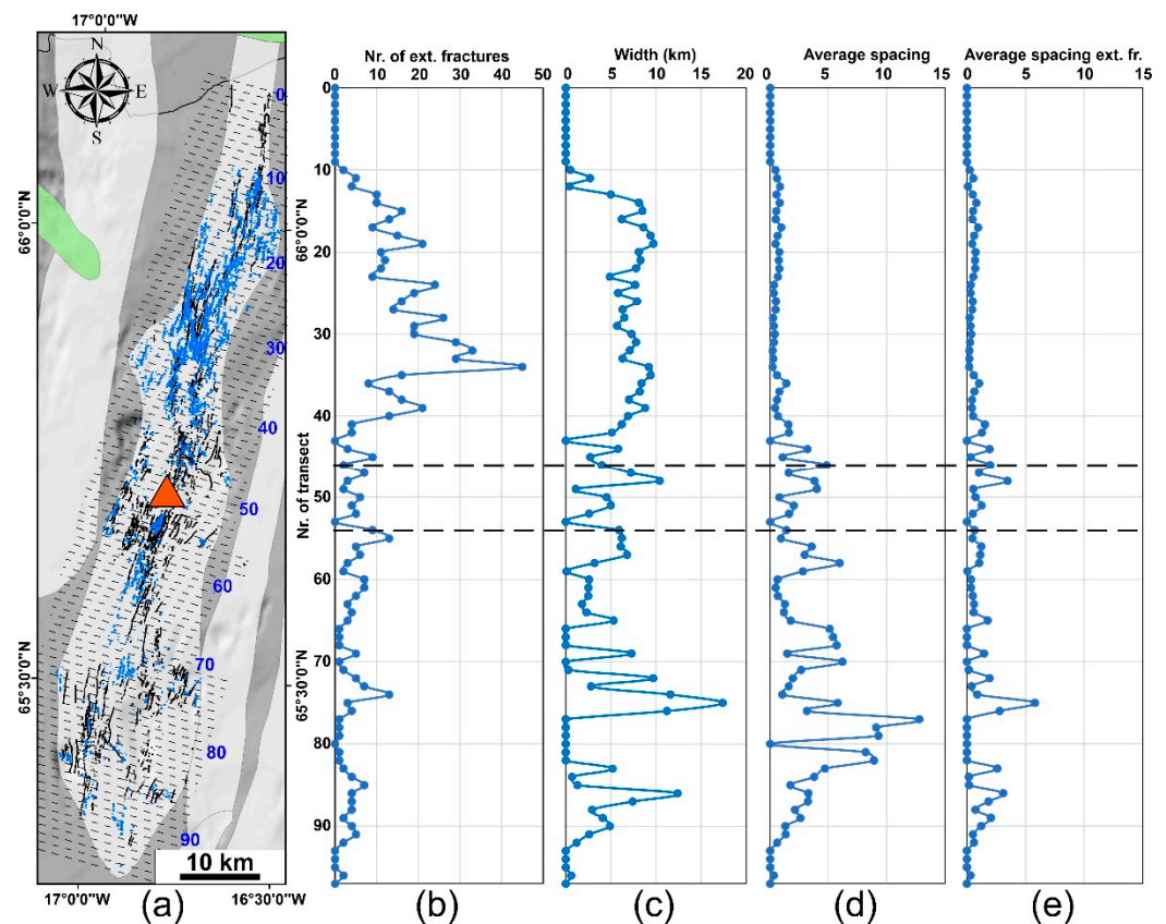
Figure 10. (a) Map representing extension fractures in the KFS, highlighted in blue. Black dashed lines show the N106°E-striking transects. Graphs showing (b) the number of extension fractures, (c) the rift width, (d) the average spacing considering the rift width shown in Figure 9c and (e) the average spacing considering the rift width shown in this figure, measured along the transects considering only extension fractures. Black dashed lines in the graphs show the location of the Krafla caldera.
