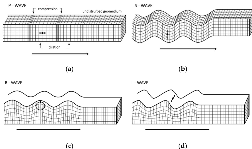
Figure 1. Seismic wave propagation: (a) longitudinal P-wave, (b) shear S-wave, (c) Rayleigh R-wave and (d) Love L-wave, modified from [24].
