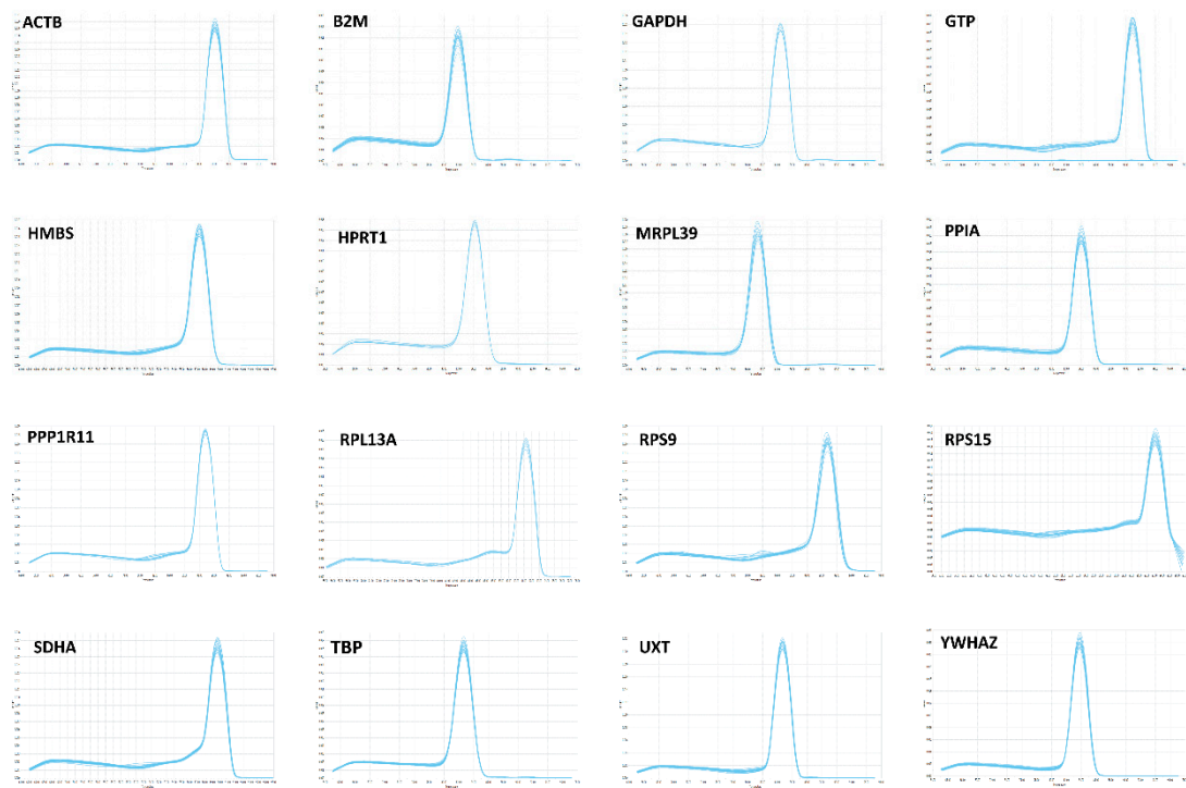
Figure S1. Melting curves of 16 candidate reference genes showing single peaks.
