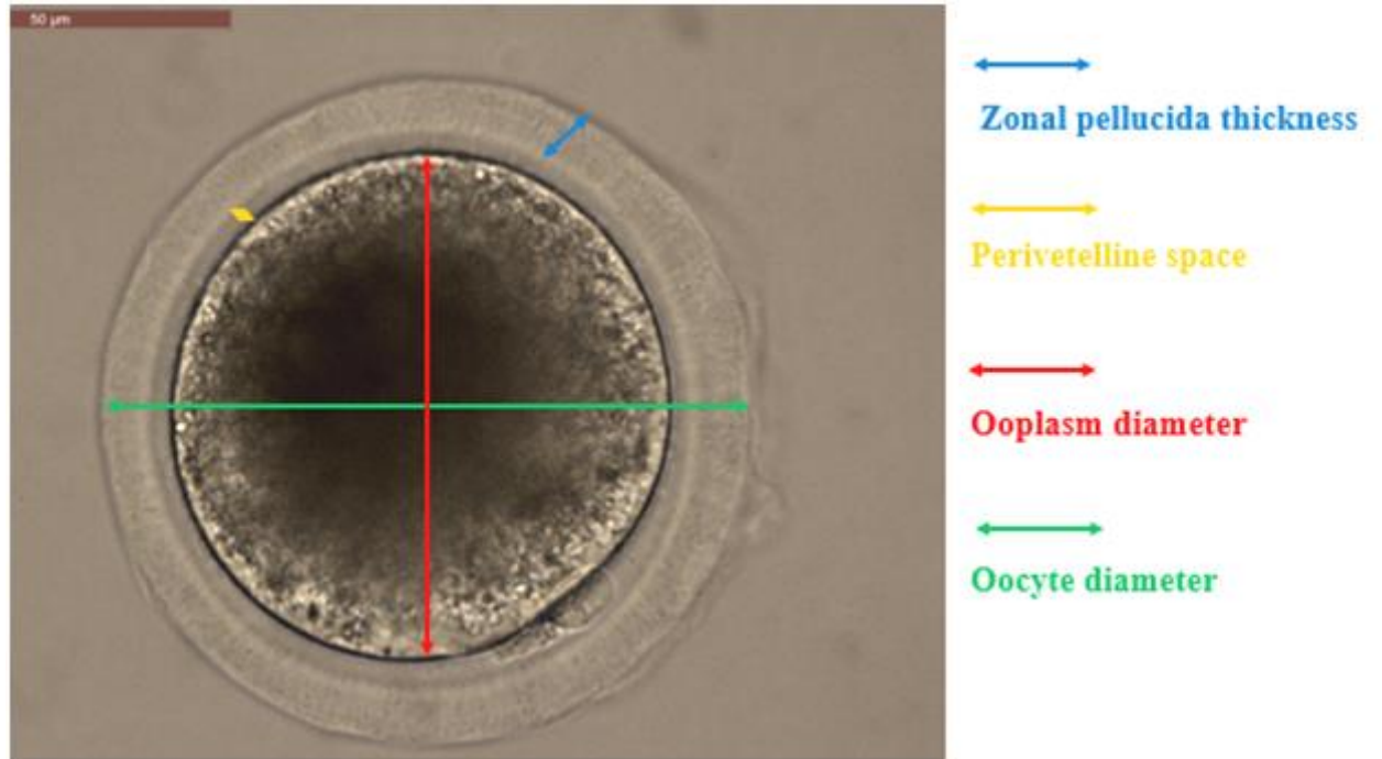
Figure S1: Camel oocyte morphometry parameters. Scale bar = 50 \mu\text{m} .
