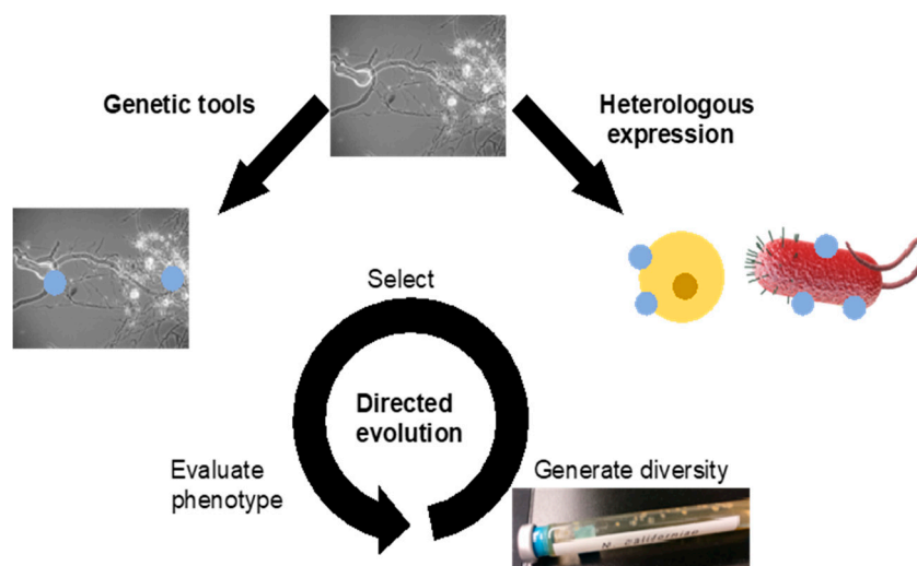
Figure 3. Anaerobic fungi show great potential for new genetic tool development and heterologous expression for biofuels production. Blue dots represent inserted or modified proteins, e.g., a
