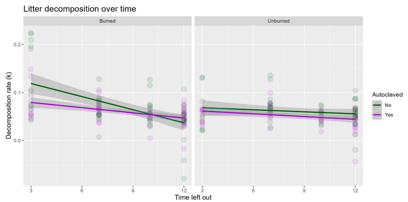
Figure 2. Litter decomposition rates over time. Litter decomposition rates generally declined over time ( p < 0.001 ) and were significantly lower in autoclave-treated litter ( p < 0.001 ). In the burned plots, decomposition rates were higher in the early sample collections (months out, p < 0.001 ), with no significant interaction between burn and autoclave treatments.
