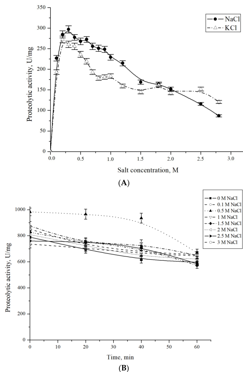
Figure 4. Effect of NaCl and KCl on the Cobetia amphilecti KMM 296 protease CamClpP (A) and salt stability (B).
