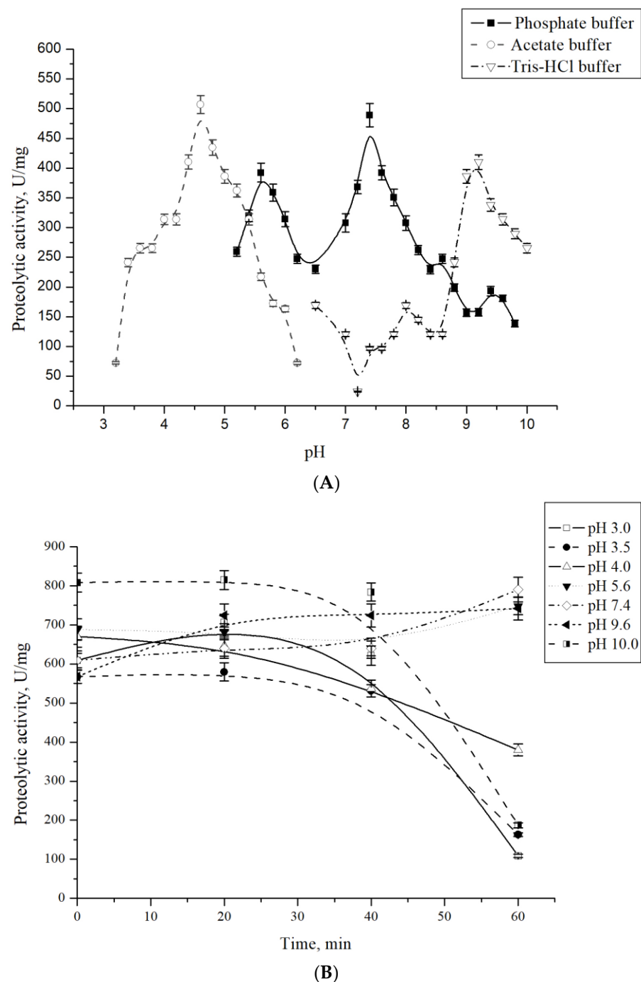
Figure 3. Effect of pH and buffer on the proteolytic activity of C. amphilecti KMM 296 protease CamClpP (A) and pH stability (B).
