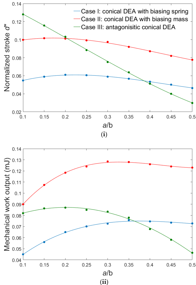
Figure 8. Maximal normalized stroke (i) and work output (ii) for three cases at pre-stretch \lambda_p = 1 \times 1 .
