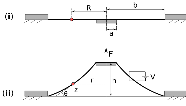
Figure 3. The cross-sectional illustrations of a conical DEA: (i) Pre-stretched membrane is bonded to a rigid ring and a central disk; (ii) out-of-plane deformation of the membrane caused by a force F and a voltage V .
