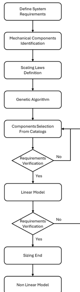
Figure 1. EMA preliminary design workflow.
