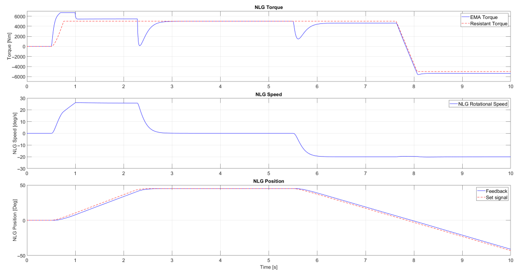
Figure 18. Preliminary non-linear model time response for a taxiing operation: the input corresponds to the maximum rotational speed, until the maximum permitted angle is reached; the reverse maneuver is then performed.
