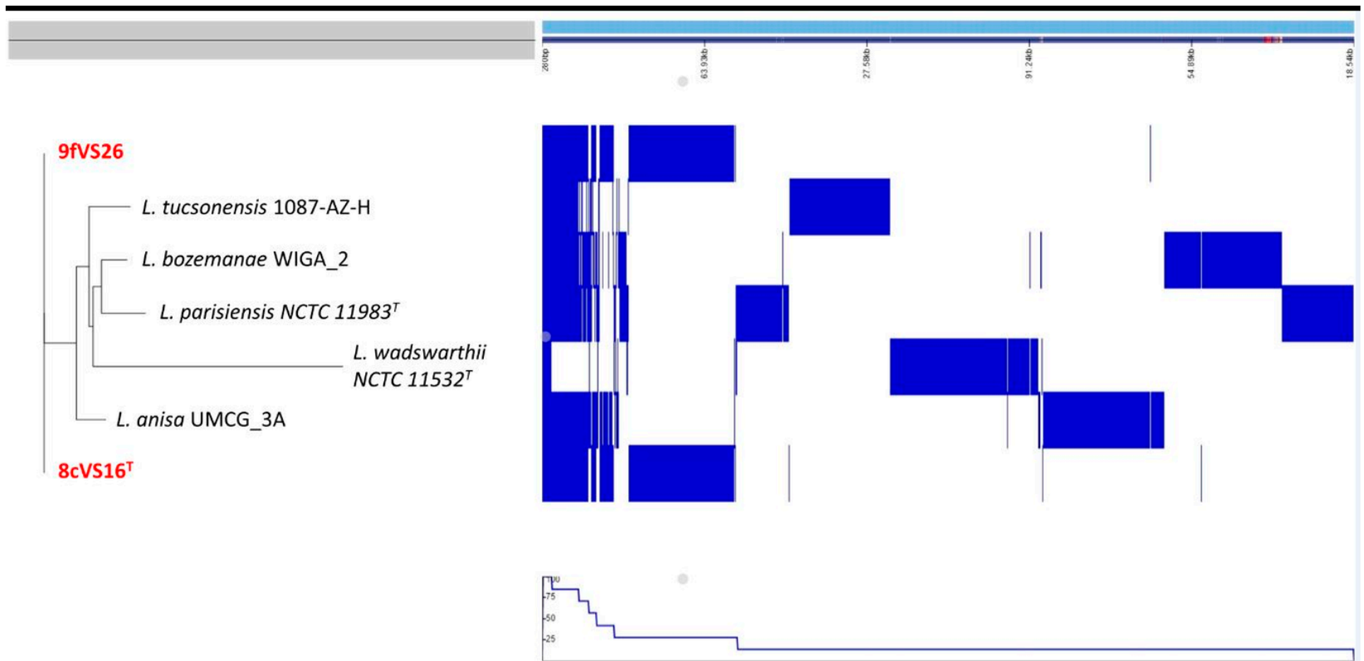
Figure 6. Visualization of the pangenome analysis of the strains 8cVS16 T and 9fVS26 obtained with Roary software (v. 3.13.0) and the close phylogenetic relative strains ( L. anisa , L. bozemanii , L. parisiensis , and L. tucsonensis ). Using the presence or absence of core genes, the whole genomes of the strains were clustered. The blue color indicated the presence of the gene, whereas the white color indicated the absence of the gene. The bottom part of the figure represents the genetic frequency of the pangenome.
