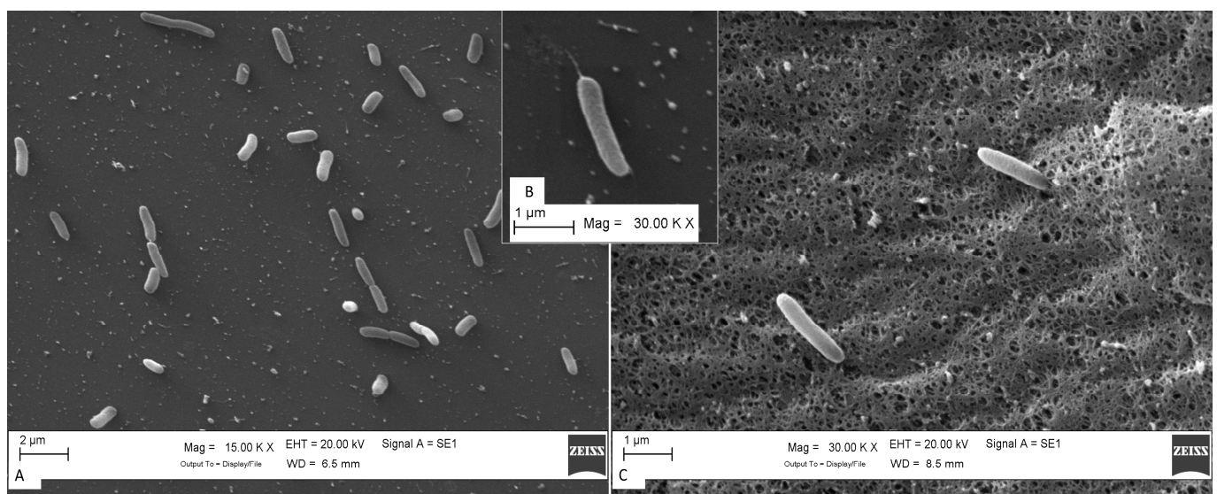
Figure 4. Scanning electron microscopy (SEM) images of strain 8cVS16T grown on BCYE Cys+ agar for 48 h at 35 °C with 2.5% CO 2 . View of (A) aflagellate form of strain grown on BCYE Cys+ (Bar 2 \mu\text{m} ), (B) flagellate form of strain grown on BCYE Cys+, and (C) fragment (5 \times 5 mm) of BCYE Cys+ medium on which the strain grew. Bar (A) 2 \mu\text{m} and (B,C) 1 \mu\text{m} . Magnification: (A) \times 15,000 and (B,C) \times 30,000 .
