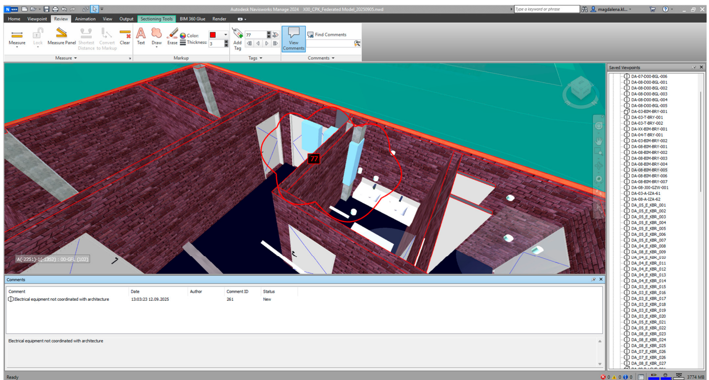
Figure 2. Autodesk Navisworks interface showing a viewpoint with proprietary issue attributes. Note the presence of timestamp, author, status, and camera position, which constitute partial reification, but the absence of standardized fields for priority, assigned person, and deadline, illustrating the limitations of vendor-specific approaches discussed in Section 5.3. Source: Own elaboration.
