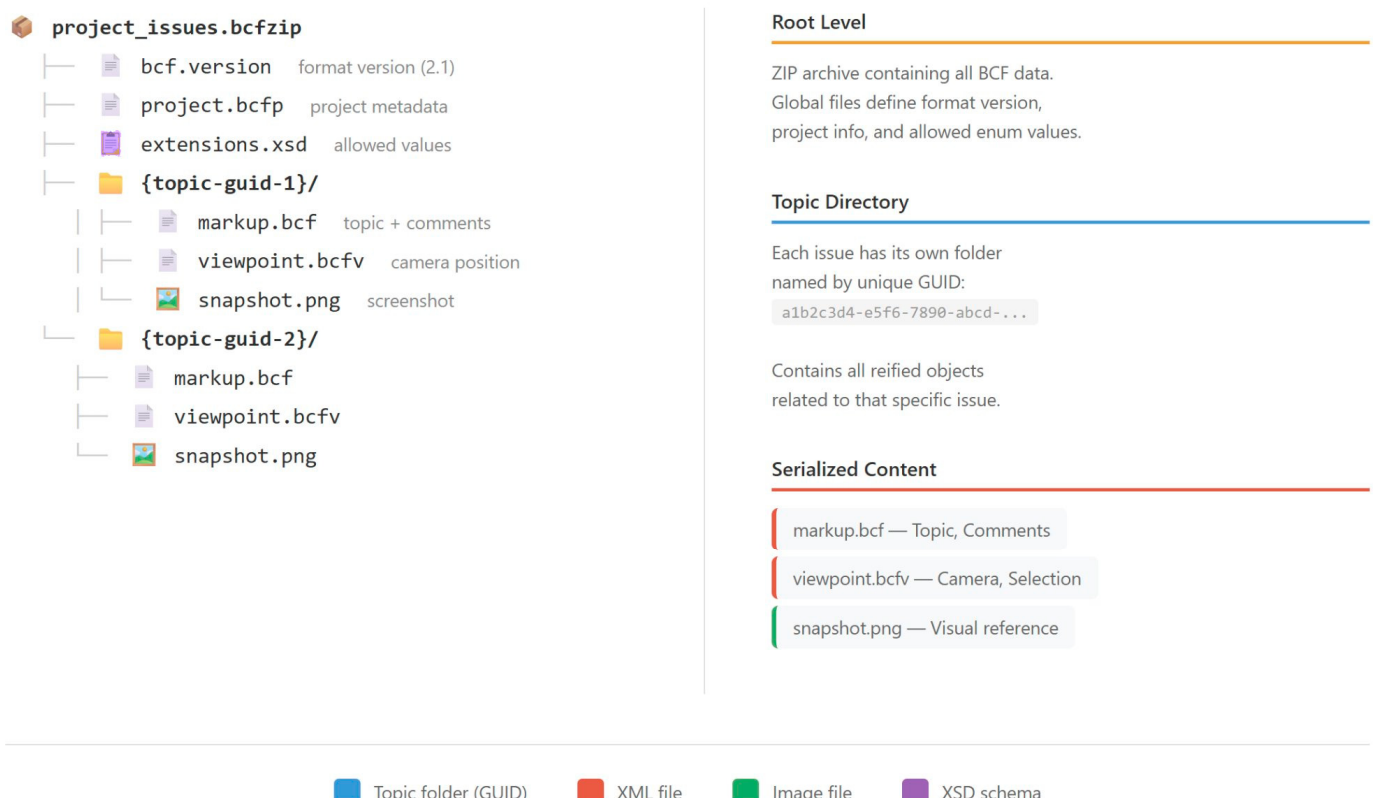
Figure 1. Diagram of the BCF file structure showing the hierarchy of directories and files along with the relationships between them. Source: Own elaboration.
