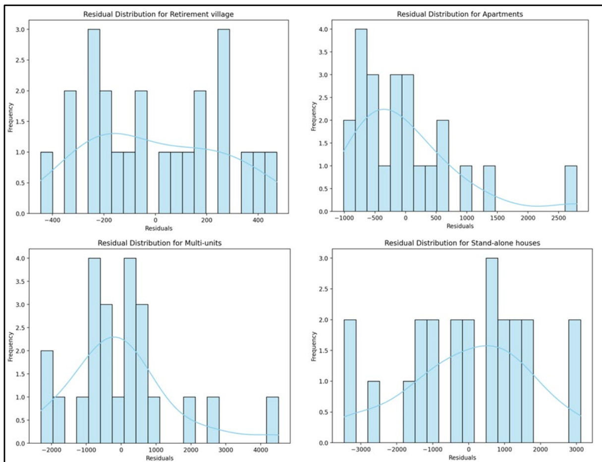
Figure 3. Residual analysis distribution for the four residential types.
