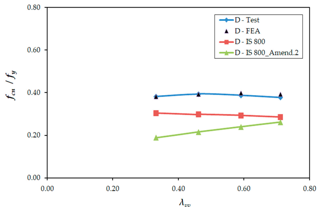
Figure 16. f_{cn}/f_y vs. \lambda_{vv} plot for single bolt—hinged case [22].
