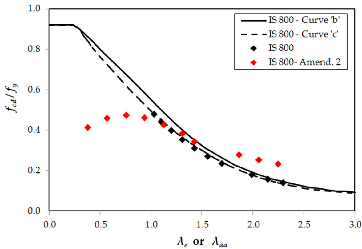
Figure 9. f_{cd}/f_y vs. \lambda plot for one bolt-fixed case.
