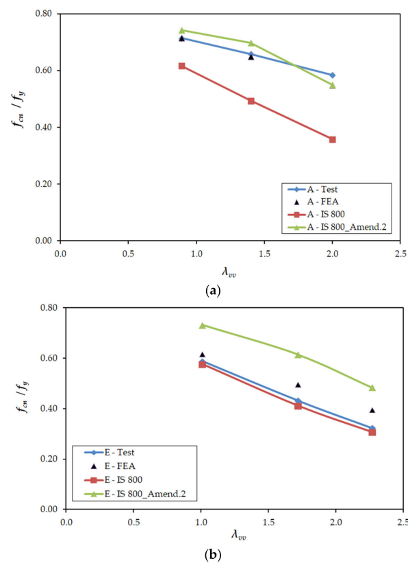
Figure 14. f_{cn}/f_y vs. \lambda_{vv} plot for two bolts—fixed case [22]: (a) series—A; (b) series—E.
