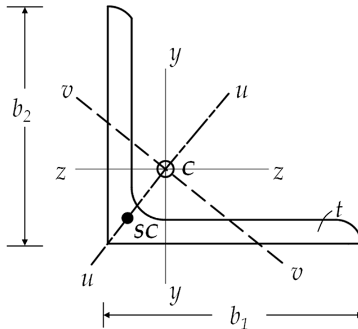
Figure 1. Angle section.
