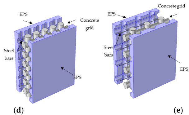
Figure 7. Constituents of Wall W 3 : (a) Steel bars; (b) Smaller concrete grid; (c) EPS sheet; (d) Whole assembly constituent of Wall W 2 ; (e) Whole assembly constituent of Wall W 3 .
