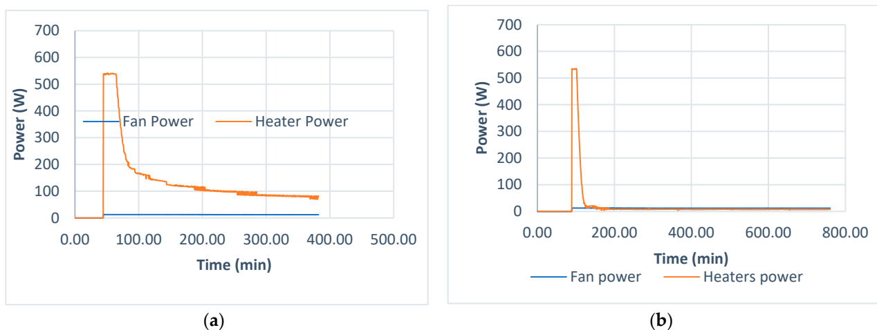
Figure 12. Variations of heater and fan power with time during Test 1: (a) Wall T_3 ; (b) Wall W_1 .
