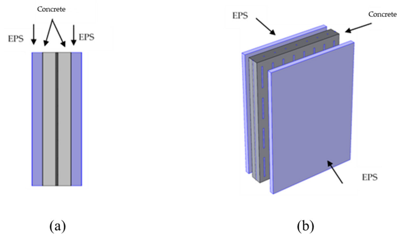
Figure 5. (a) Side view cross section of Wall W 1 ; (b) Whole assembly constituents of Wall W 1 .
