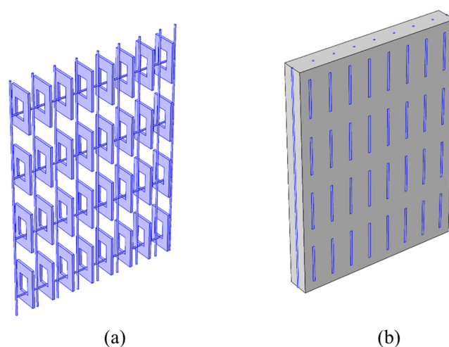
Figure 4. Constituents of Wall ( W_1 ): (a) Injected molded polypropylene crossties and steel bars; (b) Poured concrete and reinforced by the steel bars.
