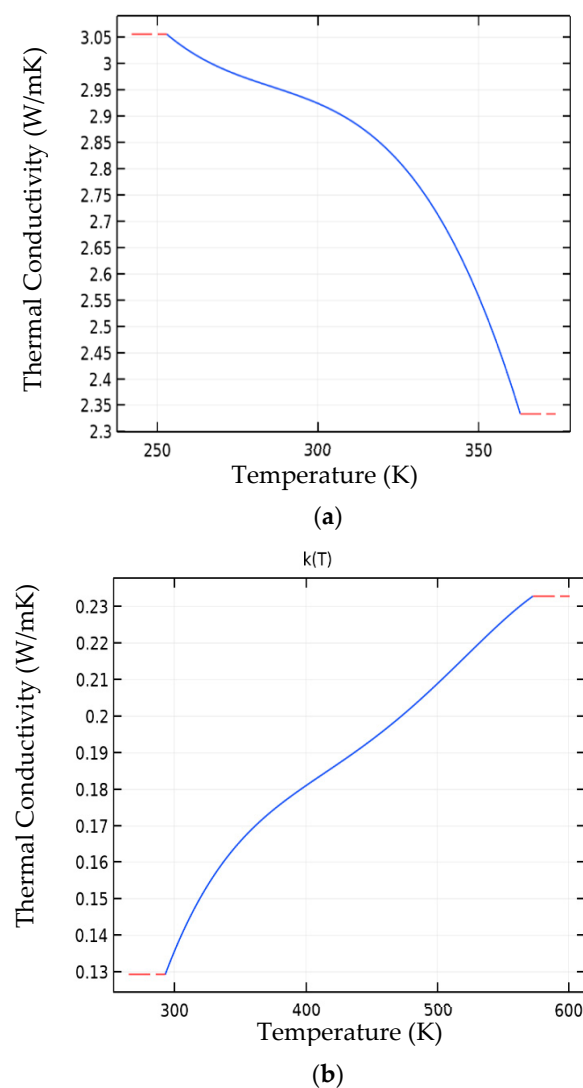
Figure 9. Thermal conductivity versus temperature (K): (a) Concrete; (b) Polypropylene.
