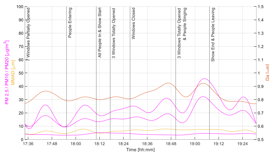
Figure 11. \text{PM}_{2.5} , \text{PM}_{10} and \text{PM}_{20} [ \mu\text{g}/\text{m}^3 ] with D_a [ \mu\text{m} ] and MMAD (median) [ \mu\text{m} ].
