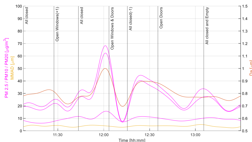
Figure 5. PM 2.5 , PM 10 and PM 20 [ \mu\text{g}/\text{m}^3 ] with D_a [ \mu\text{m} ] and MMAD (median) [ \mu\text{m} ].
