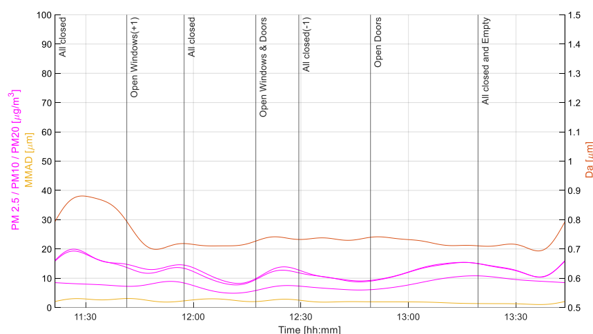
Figure 8. PM 2.5 , PM 10 and PM 20 [µg/m 3 ] with D a [µm] and MMAD (median) [µm].
