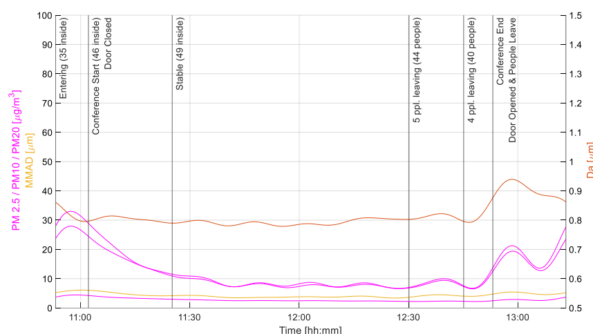
Figure 14. PM 2.5 , PM 10 and PM 20 [ \mu\text{g}/\text{m}^3 ] with D_a [ \mu\text{m} ] and MMAD (median) [ \mu\text{m} ].
