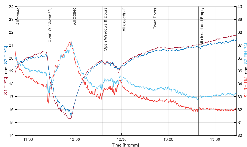
Figure 7. Temperature [°C] and relative humidity [%] for S1 and S2.
