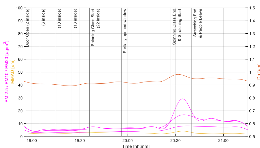
Figure 23. PM 2.5 , PM 10 and PM 20 [µg/m 3 ] with D a [µm] and MMAD (median) [µm].
