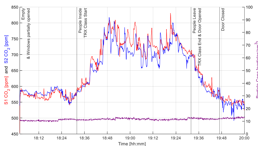
Figure 18. CO 2 concentration [ppm] for S1 and S2 and particle concentration [particles/cm 3 ].
