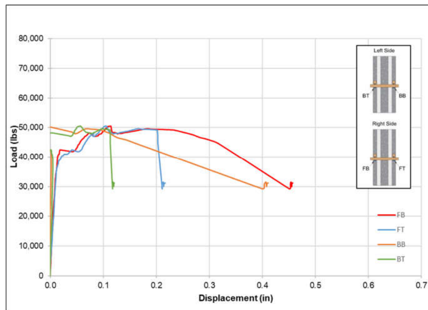
Figure 14. Load vs. displacement data from the four sensors for EPS.24.4.MMGRID.3.
