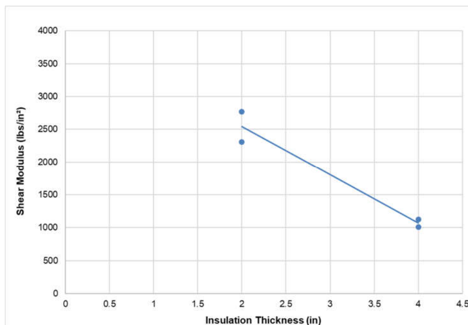
Figure 22. Shear modulus vs. insulation thickness graph of EPS.24.2.MMGRID and EPS.24.4.MMGRID specimens.
