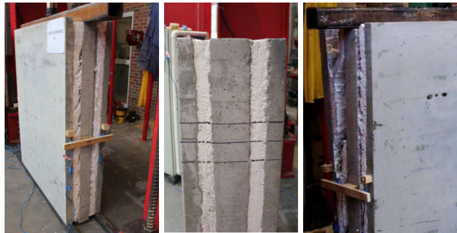
Figure 7. Panels EPS.24.2.MMGRID.1 (left), 2 (middle), and 3 (right) after testing.
