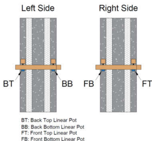
Figure 5. Locations of linear potentiometers for all tests.
