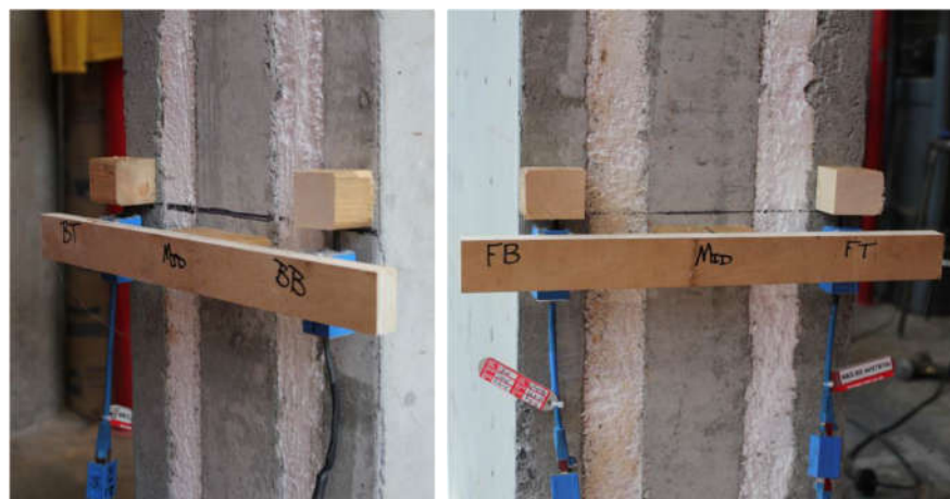
Figure 6. A typical panel with potentiometers installed.
