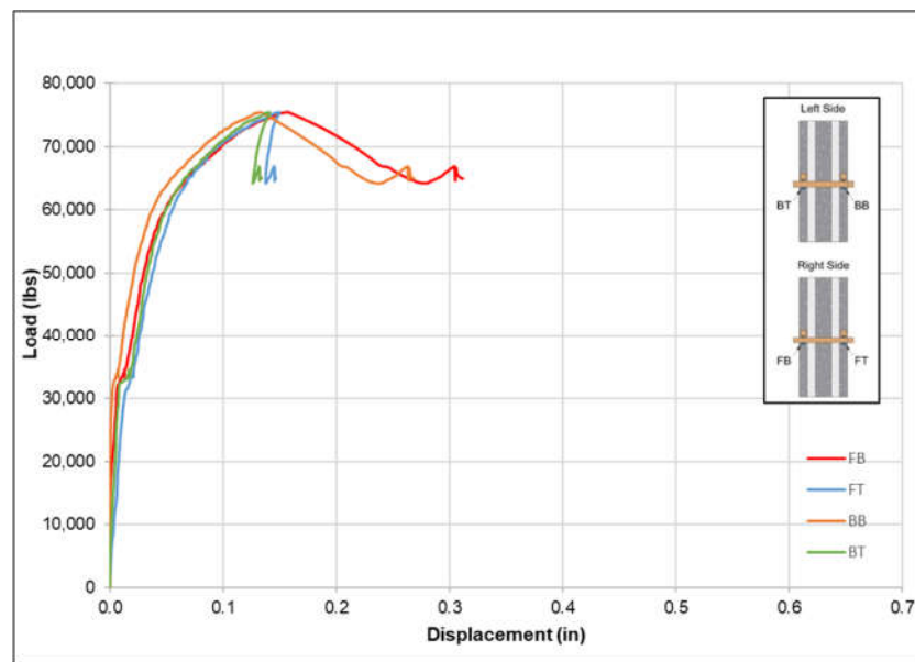
Figure 9. Load vs. displacement data from the four sensors for EPS.24.2.MMGRID.2.
