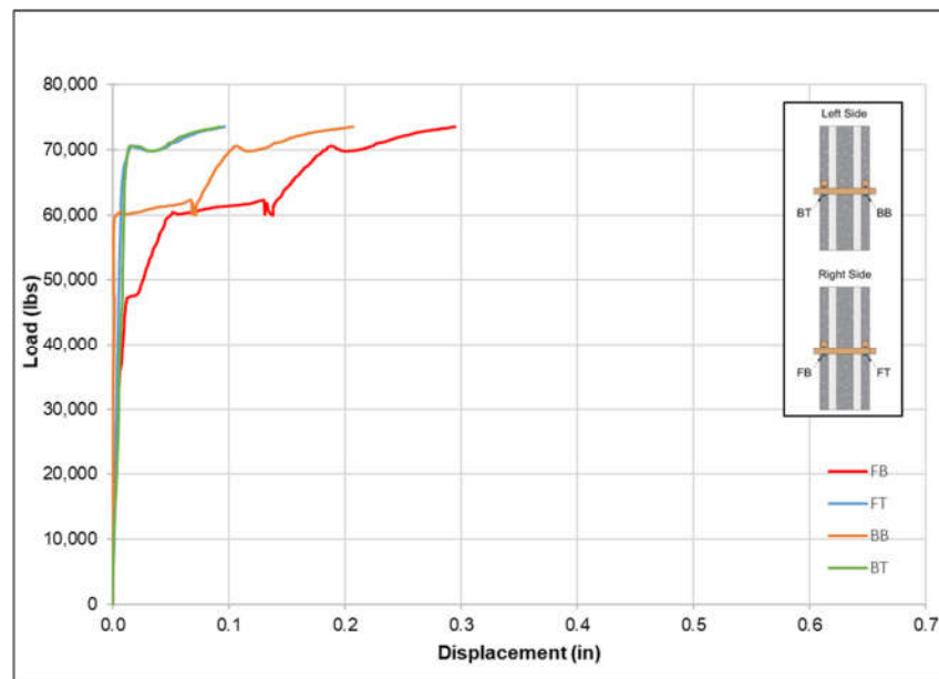
Figure 10. Load vs. displacement data from the four sensors for EPS.24.2.MMGRID.3.
