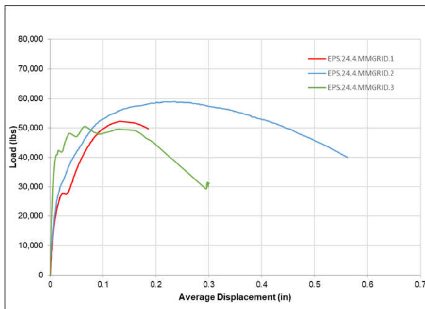
Figure 16. Average displacement behavior for each of the three specimens having 4 in (102 mm) EPS.
