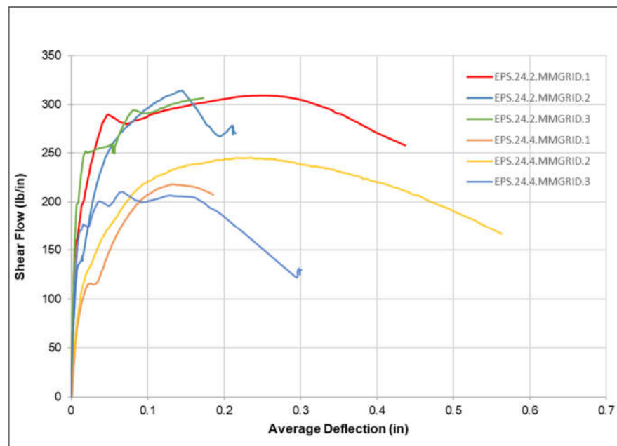
Figure 17. Effect of EPS insulation thickness: shear flow vs. average deflection graph of EPS.24.2.MMGRID and EPS.24.4.MMGRID specimens.
