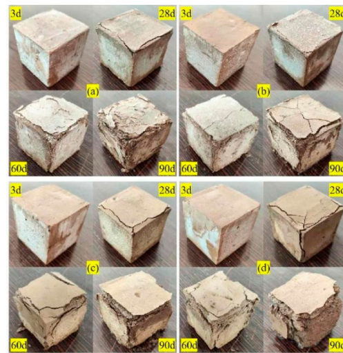
Figure 3. Visual appearance of SF-GSSS immersed in a \text{MgSO}_4 solution: (a) S10F0; (b) S9F1; (c) S8F2; and (d) S7F3.
