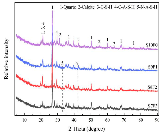
Figure 8. XRD analysis of SF-GSSS before sulfate attack.
