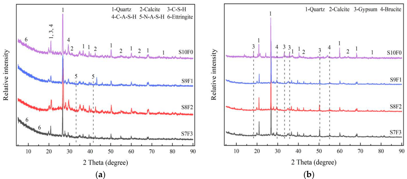
Figure 9. XRD analysis of SF-GSSS after 60 days immersion: (a) \text{Na}_2\text{SO}_4 solution and (b) \text{MgSO}_4 solution.
