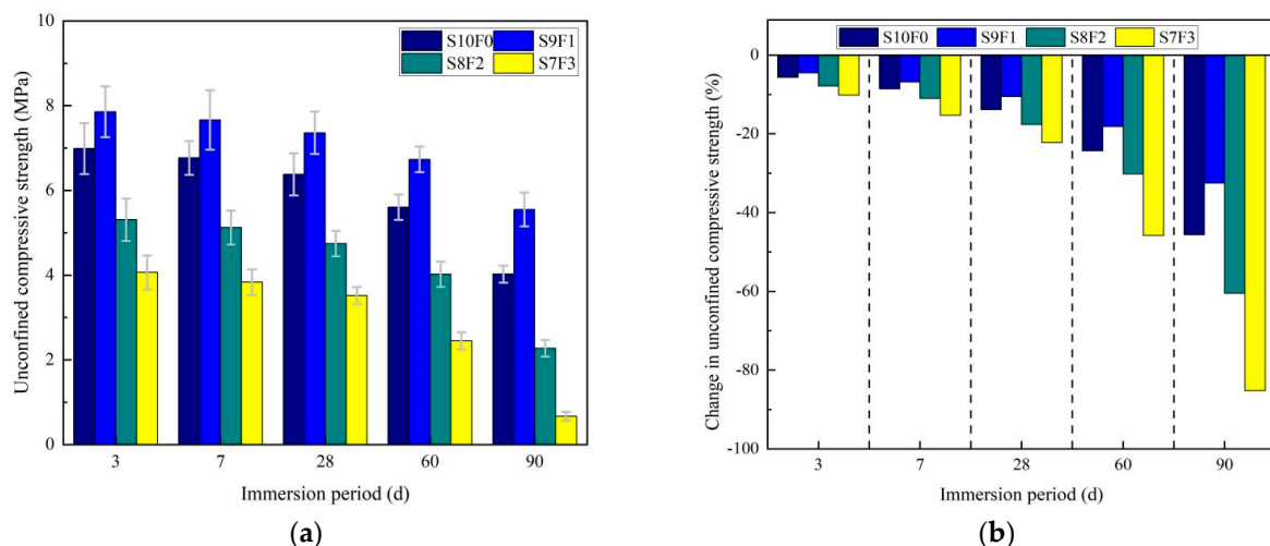
Figure 6. (a) The UCS of SF-GSSS immersed in \text{MgSO}_4 solution at various times. (b) Change in UCS.
