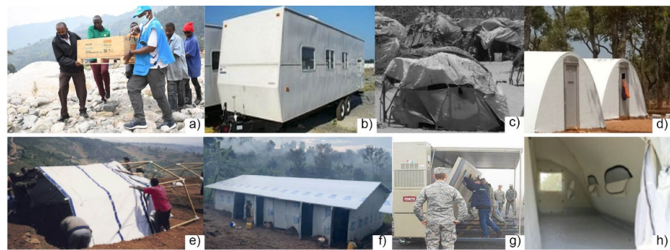
Figure 6. Selected temporary shelters. (a) High Performance Tent, UNICEF (© UNICEF/UN0588296/Wamala) [48]; (b) FEMA trailer, US agency [42,49]; (c) Makeshift Shelter2, refugees in Chad, 2017 [39,50]; (d) Lifeshelter, Jens O. Olsson [51,52]; (e) Bamboo tent, Shigeru Ban architect, Rwanda, 1999 (© Shigeru Ban architect) [53]; (f) Shelters for the Ituri crisis, ShelterCluster, Dem. Rep. Congo, 2017 and outward (©Anja Pirjevec) [39]; (g) Deployable truck, Forts [54]; (h) Self-standing family tent, ShelterCluster [55].
