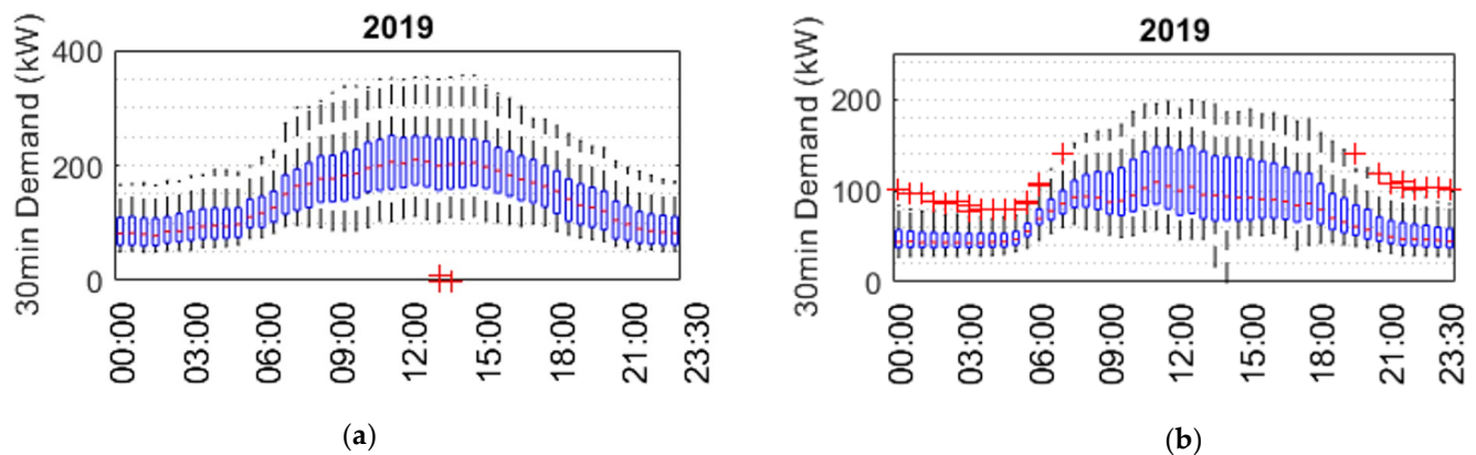
Figure 4. Annual demand profile expressed in boxplots from Community 1 (a) and Community 3 (b).
