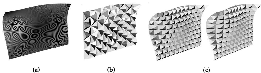
Figure 33. (a) Volumetrically influential zebra-striped surface; (b) Triangular pyramid panel generated by the increments of the zebra-striped surface; and (c) Rectangular pyramid panel generated by the increments of the zebra-striped surface.
