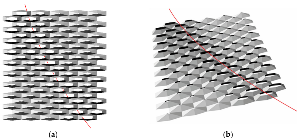
Figure 20. Proposed 3D parametric pyramidal geometry. (a) top view; and (b) perspective view of the adaptive surface resulting from the definition (the red line represent potential external stimuli).
