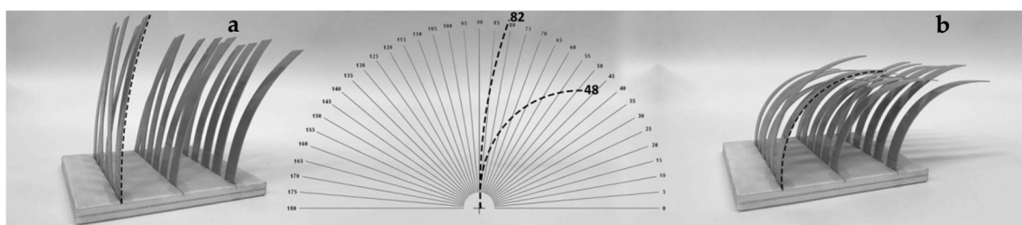
Figure 12. Tangential cut sycamore veneer and Kapton tape and their shape change influenced by temperature variations, 18 °C (a) versus 50 °C (b) with resulted angle changes.
