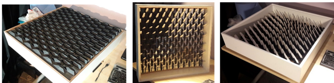
Figure 27. Assembled model consisting of the 3D-printed modules, lamellae, frame, and glass panel.
