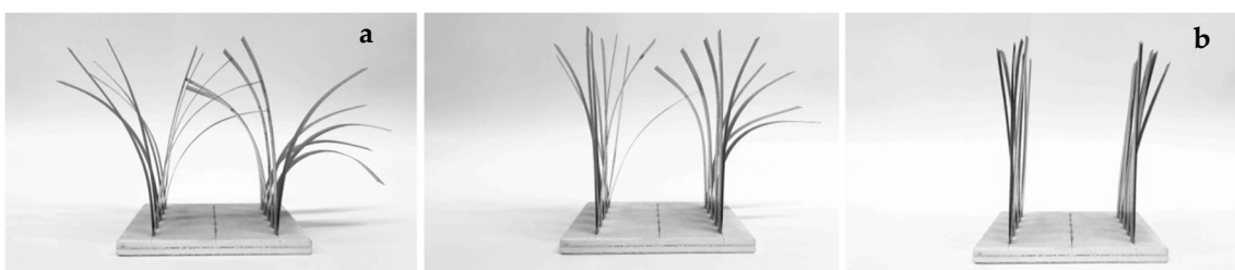
Figure 11. Recycled package paper and Kapton tape and their shape change influenced by temperature variations, 18 °C (a) up to 50 °C (b), front views, 2 parallel row arrangement of the lamellae.
