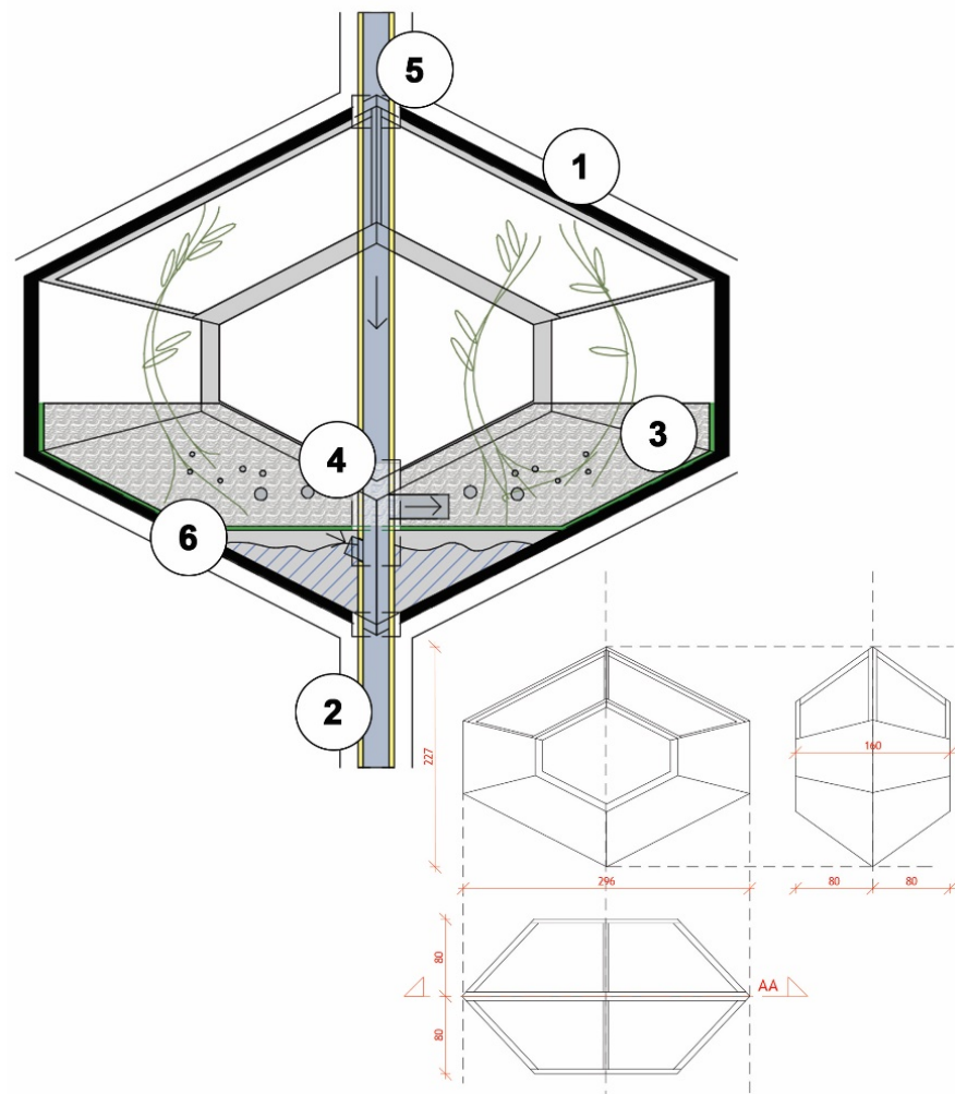
(C) MODGREW module components
