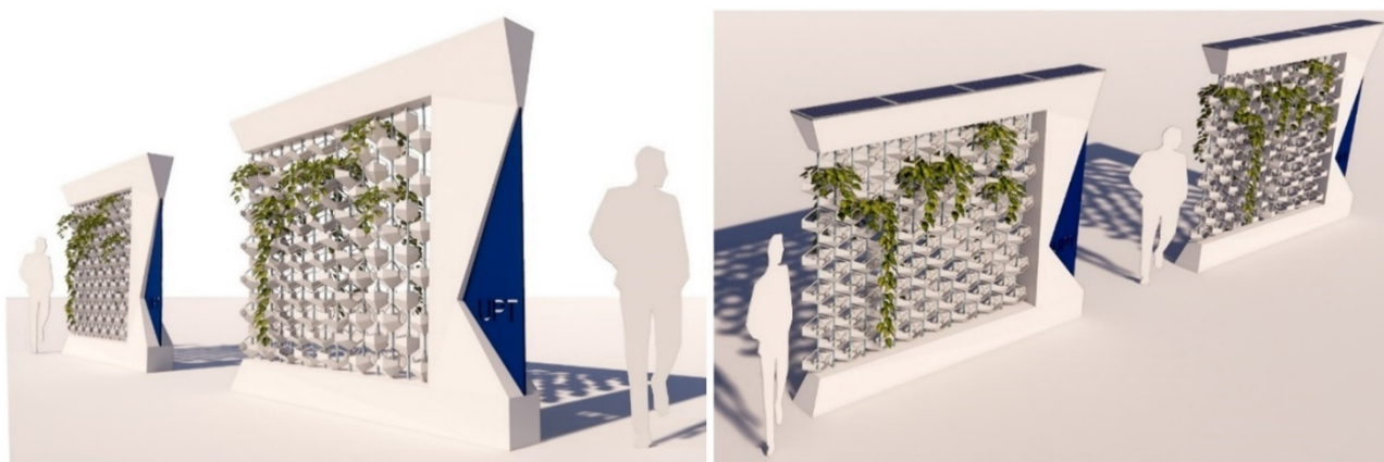
Figure 43. Final render—perspective views, initial position of the modules and rotated position as seen at a human scale.
