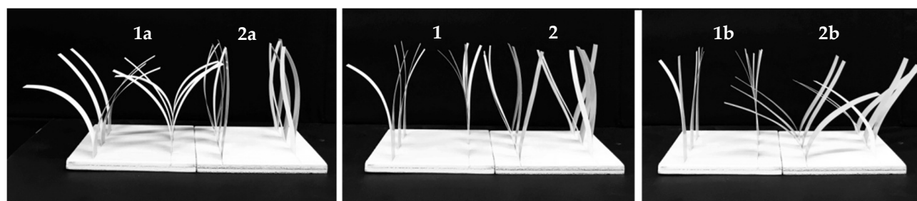
Figure 14. Drawing paper and Kapton tape—comparison between 2 different samples with tape on the exterior (1) and interior (2) and shape change influenced by temperature variations, 18 °C (1a and 1b) up to 50 °C (2a and 2b).
