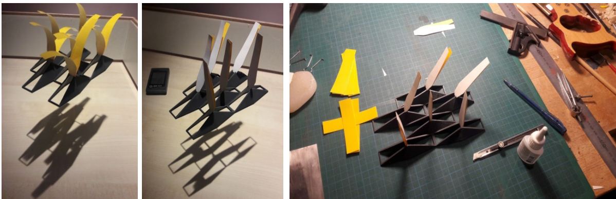
Figure 25. First successful samples of 3D printed modules with shape-changing lamellae.
