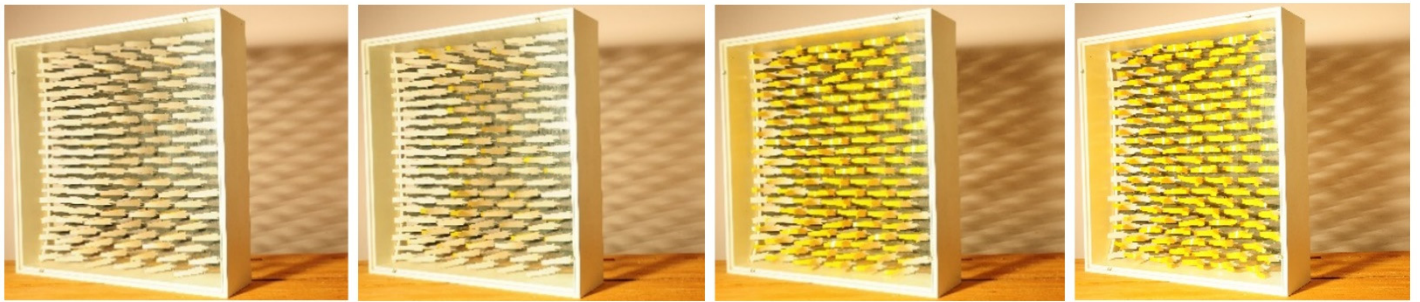
Figure 28. Assembled model and physical reaction and movement of the shape-changing lamellae, right view of the model.
