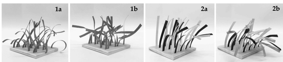
Figure 9. Kraft paper and Kapton tape (1a and 1b), respectively, Copier paper, black ink and Kapton tape (2a and 2b) and their shape change influenced by temperature variations, 18 °C (1a and 2a) versus 50 °C (1b and 2b)—conclusion: failure.
