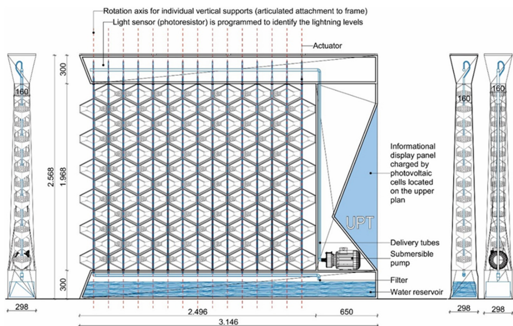
Figure 40. Final prototype technical drawings.
