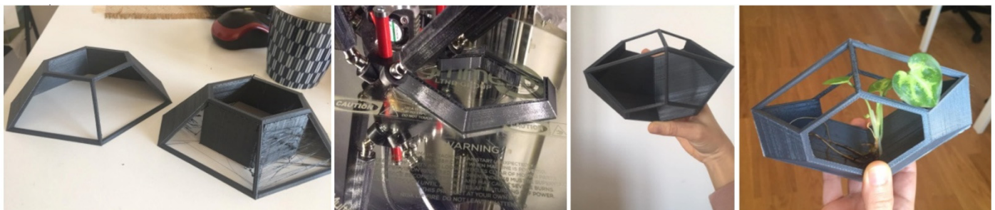
Figure 39. First successful samples of 3D printed modules with planter areas.
