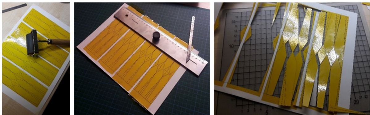
Figure 26. Printing, gluing, and cutting processes for the shape-changing lamella.
