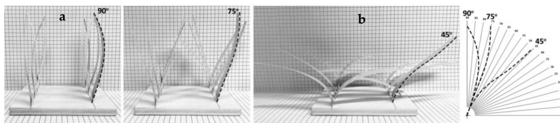
Figure 17. Final sample, drawing paper and Kapton tape on the interior—their shape change influenced by temperature variations, 18 °C (a) up to 50 °C (b).
