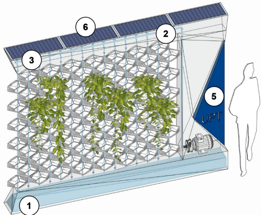
(B) MODGREW main automation features
