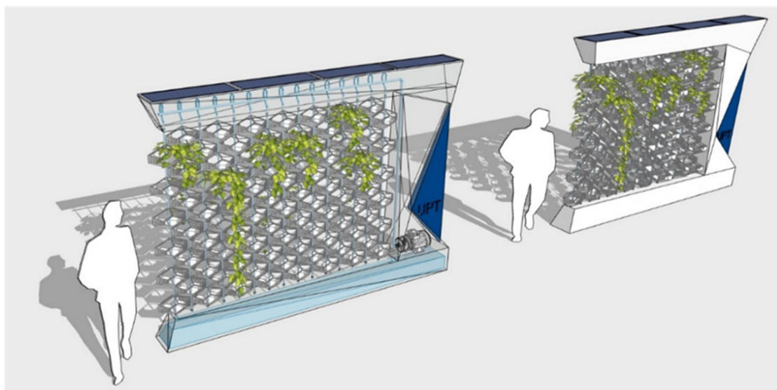
Figure 42. Final prototype technical drawings—perspective views, initial position of the modules and rotated position, including aerial views of the photovoltaic cells.
