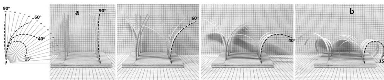
Figure 16. Final sample, drawing paper and Kapton tape on the exterior—their shape change influenced by temperature variations, 18 °C (a) up to 50 °C (b).
