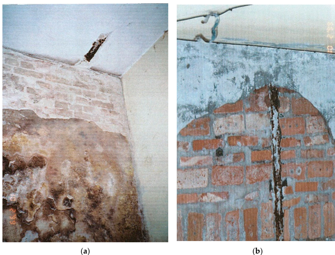
Figure 9. Willa Halina, view of degraded structural elements. (a) Mold on the outside wall; (b) moisture and corrosion of internal wall elements. Source: FORT Taraszkiewicz Architekci.
