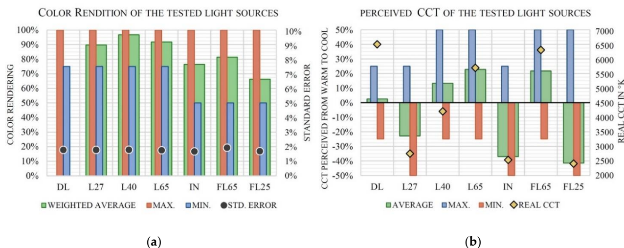
Figure 7. (a) Left: Subjective color rendition provided by the tested light sources of the set of color samples. (b) Right: Perceived correlated color temperature (CCT) produced by the tested light sources.
