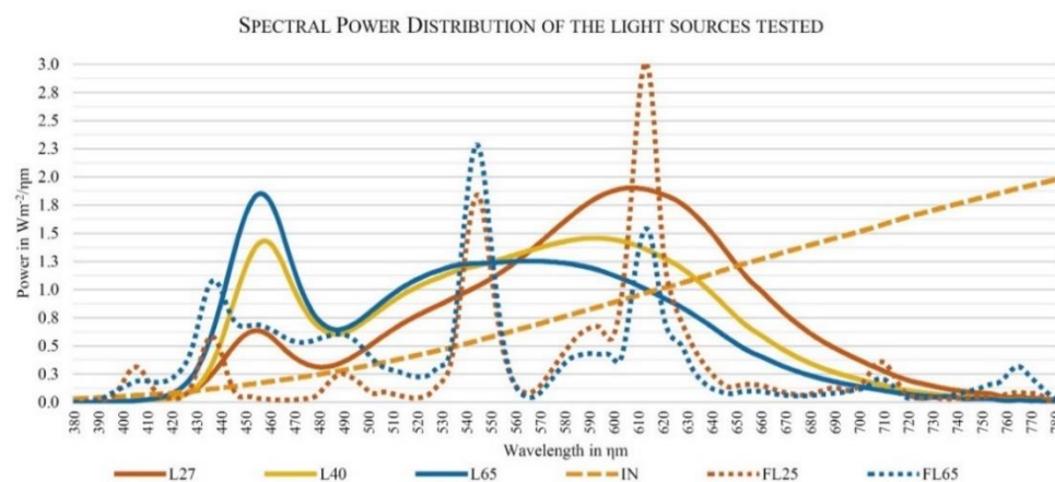
Figure 5. SPDs of the electric light sources tested.
