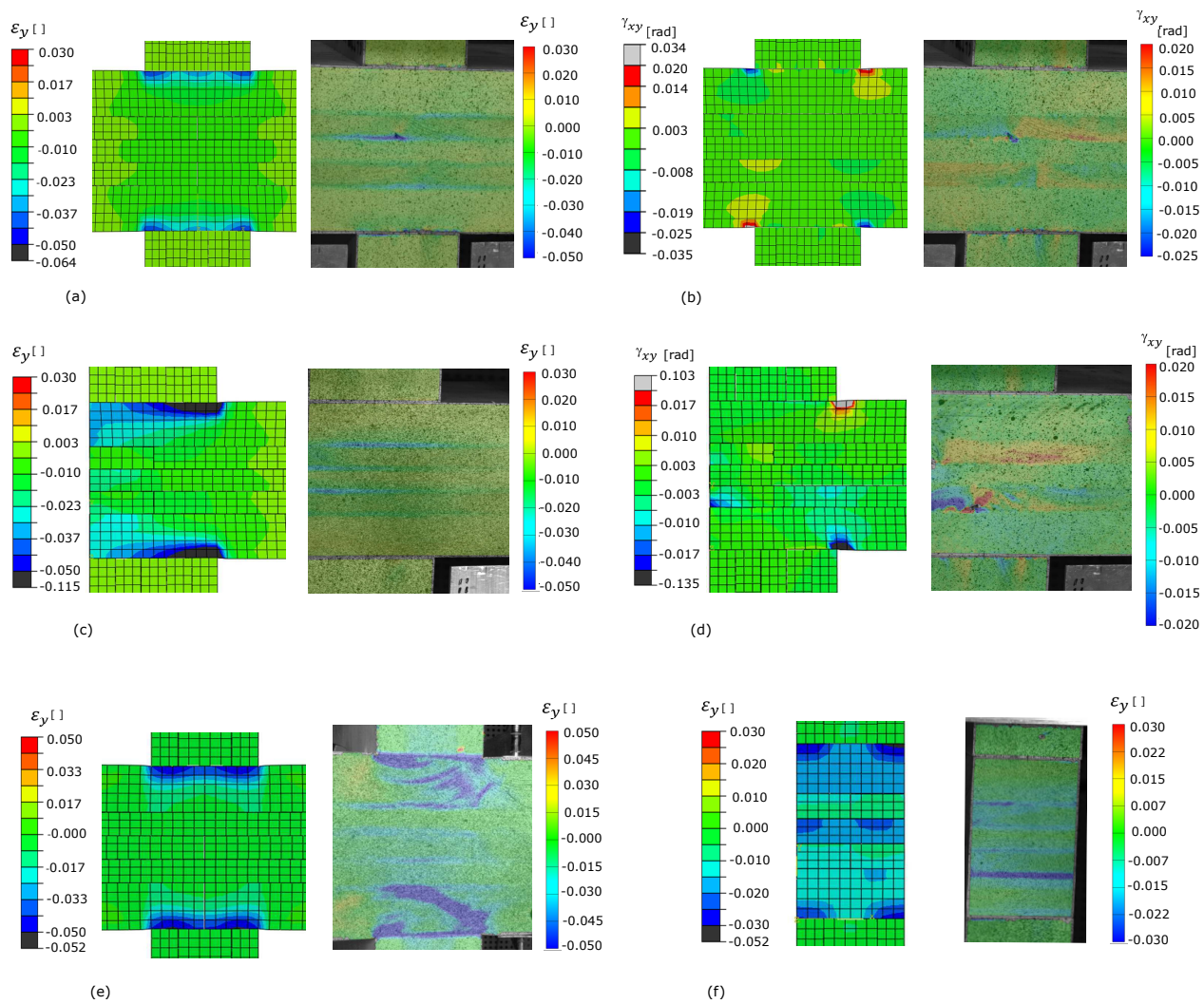
Figure 10. Strain distributions from numerical model (left) and experiments (right) for W100-F140-wv-cen setup: (a) compressive strain and (b) shear strain; for W100-F140-wv-edge setup: (c) compressive strain and (d) shear strain; (e) compressive strain for W80-F140-wv90-cen and (f) W80-F140-full comp. at about 2.5 mm global displacement.
