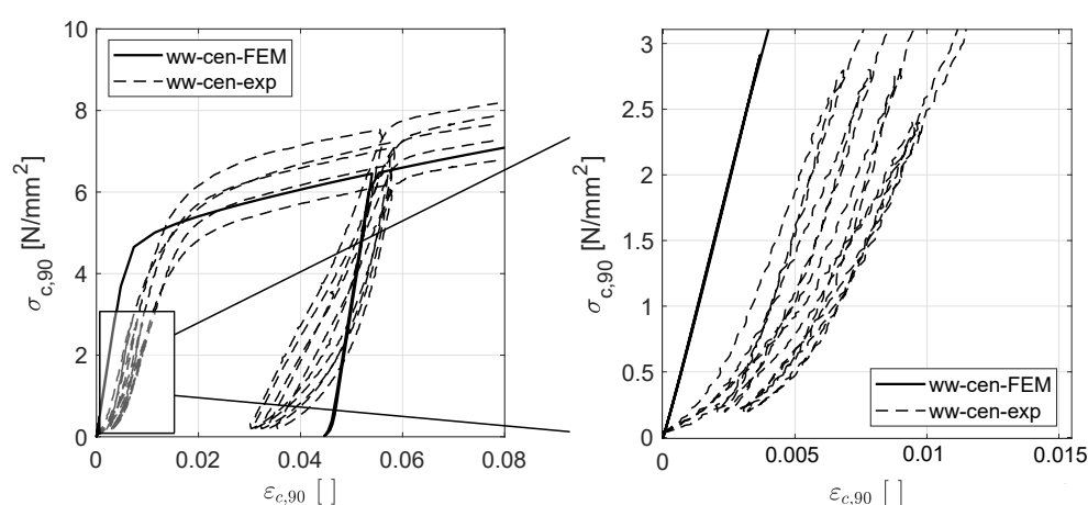
Figure 4. Compression stress vs. strain curves for W100-F140-cen-ww from FEM and experiment with unloading and reloading paths.
