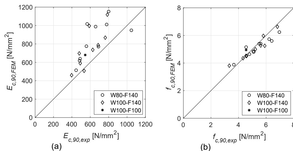
Figure 3. Correlation plot of (a) E_{c,90} and (b) f_{c,90} from FEM and experiment.
