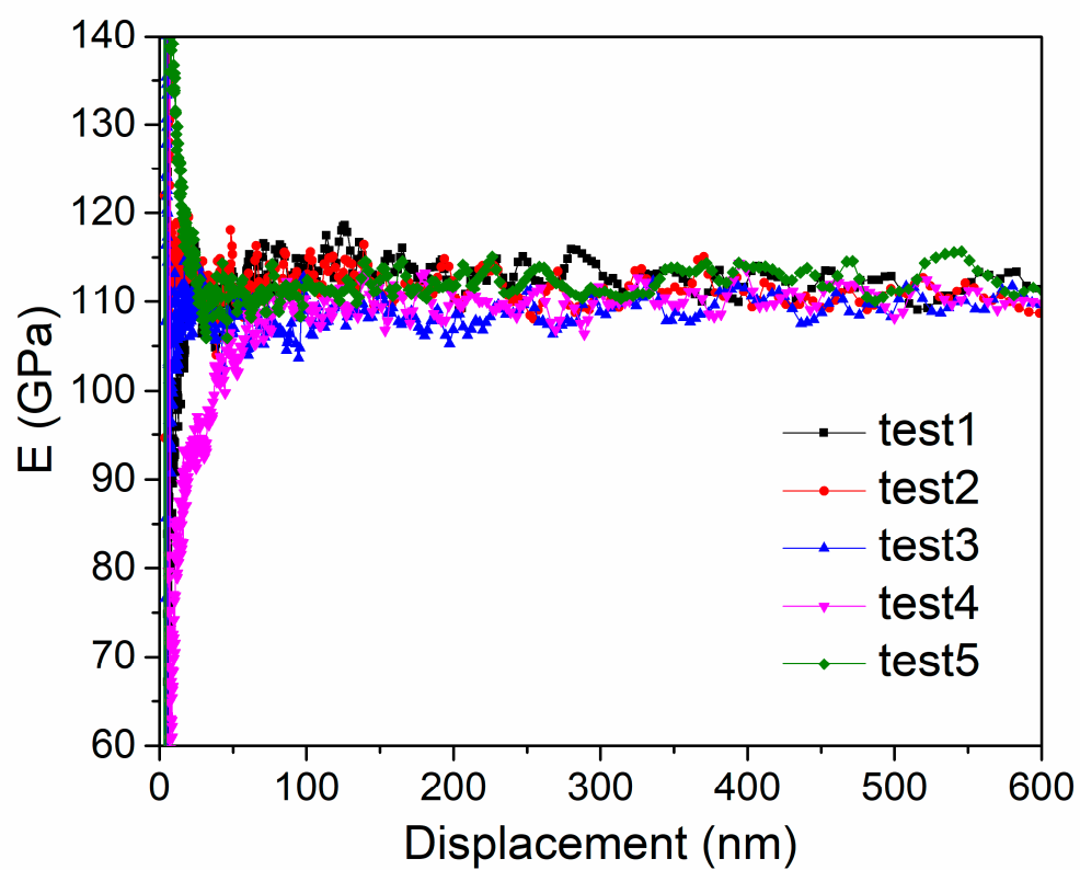
Figure 3. Elastic modulus was measured by continuous stiffness module (CSM) and was depicted as a function of displacement. The mean elastic modulus was 110 GPa.
