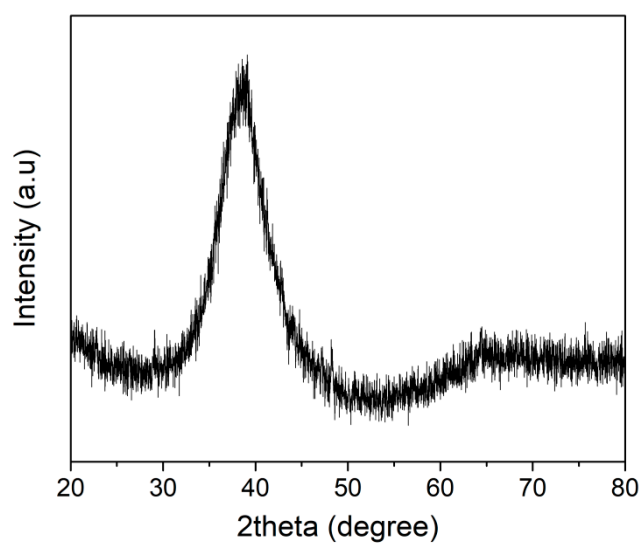
Figure 1. The typical XRD pattern of as-cast Zr-Cu-Ag-Al alloy.
