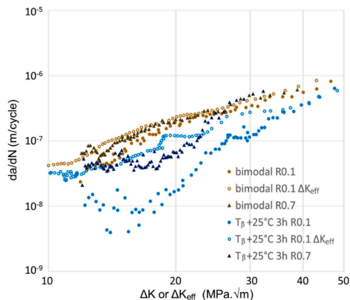
Figure 14. Fatigue crack propagation rates as a function of effective stress intensity range \Delta K_{\text{eff}} at R = 0.1 and R = 0.7 tests of the bimodal microstructure and one lamellar microstructure.
