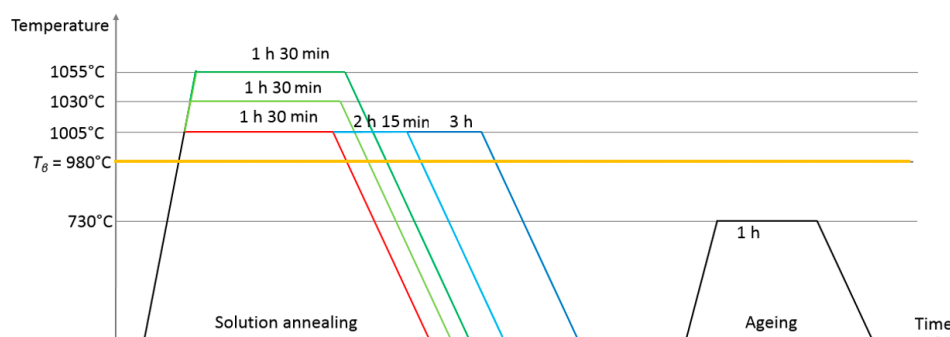
Figure 4. Heat treatments performed.
