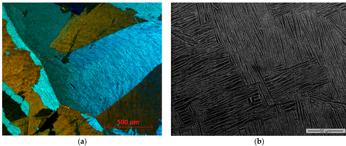
Figure 6. Lamellar microstructure obtained with annealing temperature T_{\beta} + 25^{\circ}\text{C} for 3 h, viewed with polarized optical microscopy (a) and SEM (b).
