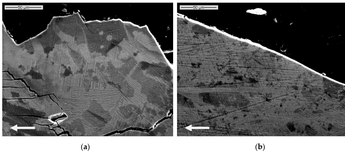
Figure 11. Crack path at mid-thickness before (a) and after (b) transition, respectively at \Delta K = 20 \text{ MPa}\sqrt{\text{m}} and at \Delta K = 40 \text{ MPa}\sqrt{\text{m}} , T_{\beta} + 75 \text{ }^{\circ}\text{C} for 1 h 30 min heat treatment, propagation according to the arrow.
