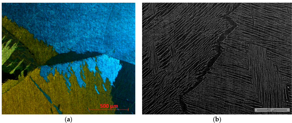
Figure 7. Lamellar microstructure obtained with annealing temperature T_{\beta} + 75^{\circ}\text{C} for 1 h 30 min, viewed with polarized optical microscopy (a) and SEM (b).
