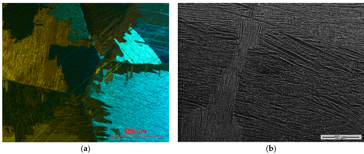
Figure 5. Lamellar microstructure obtained with annealing temperature T_{\beta} + 25^{\circ}\text{C} for 1 h 30 min, viewed with polarized optical microscopy (a) and SEM (b).
