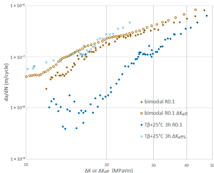
Figure 16. Fatigue crack propagation rates as a function of effective stress intensity range \Delta K_{eff} and \Delta K_{eff,S} at R = 0.1 for one lamellar microstructure, compared to the bimodal microstructure.
