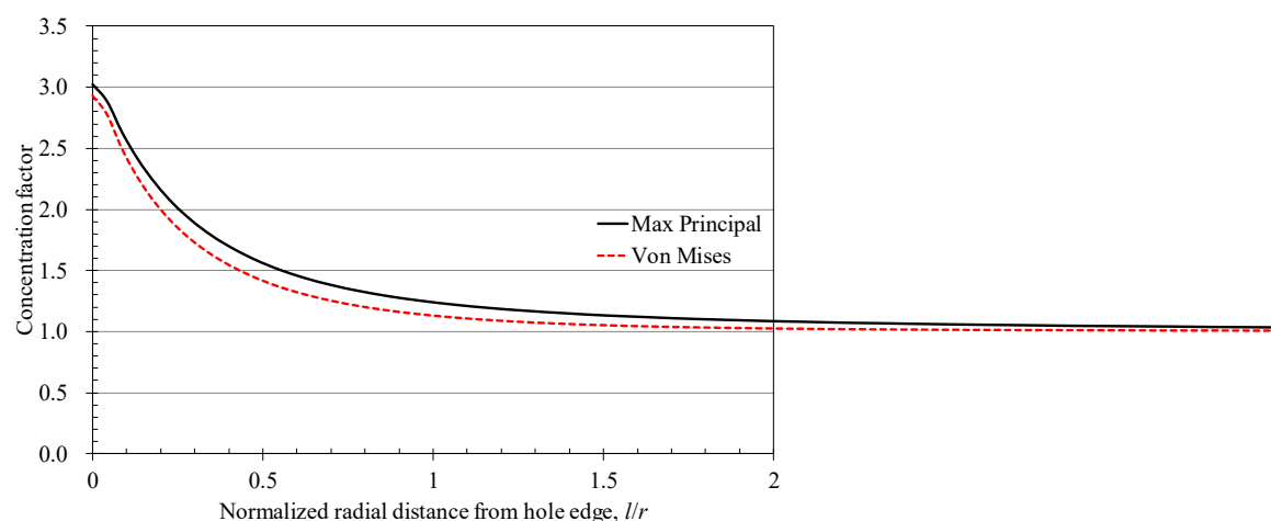
Figure 8. Distribution of Mises stress and max principal stress radially away from hole edge on specimen outer surface (path P3).
