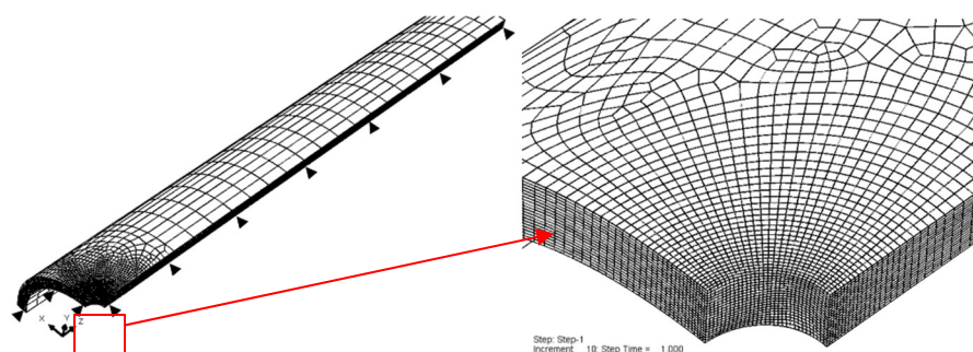
Figure 4. Finite element model.
