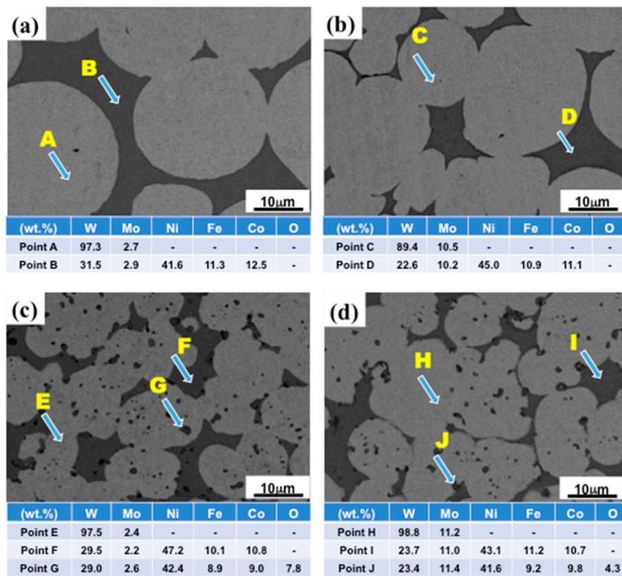
Figure 5. Energy-dispersive X-ray spectroscopy (EDS) analysis of the sintered (a) W3Mo, (b) W12Mo, (c) W3Mo-YO, and (d) W12Mo-YO model alloys milled for 24 h.
