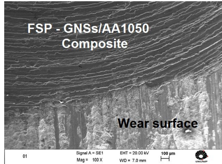
Figure S2. SEM images of samples surface before and after FSP
