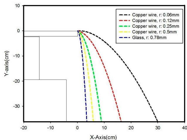
Figure 8. Trajectory simulation by particle size for copper wires and glass. (Applied voltage ( U ): 20 kV initial speed ( v_0 ): 0.13 \text{ m}\cdot\text{s}^{-1} , distance between two electrodes ( L ): 0.6 m).
