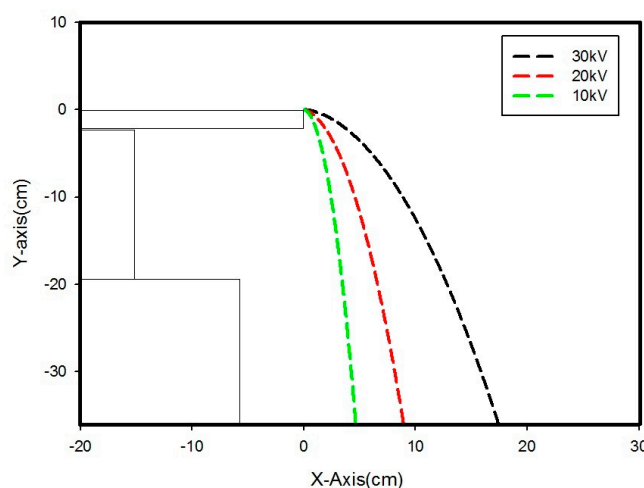
Figure 9. Trajectory simulations as applied voltage. (Radius of copper wire ( r_p ): 0.00025 m, length of copper wire ( l_p ): 0.01 m, initial speed ( v_0 ): 0.13 m·s -1 , distance between two electrodes (L): 0.6 m).
