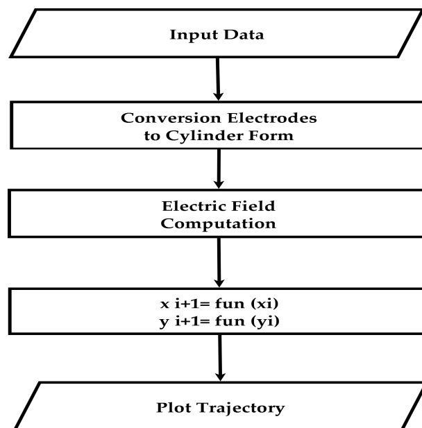
Figure 2. Flow chart of the particle trajectory computation.
