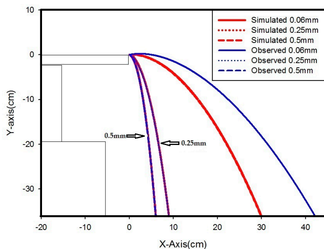
Figure 10. Comparison of conductive particle trajectory by observation vs. simulation. (Applied voltage ( U ): 20 kV, initial speed ( v_0 ): 0.13 \text{ m}\cdot\text{s}^{-1} , distance between two electrodes ( L ): 0.6 m).
