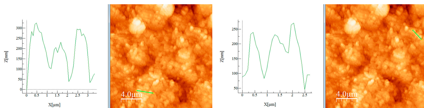
Figure 9. Surface profile of selected areas of sample S2.
