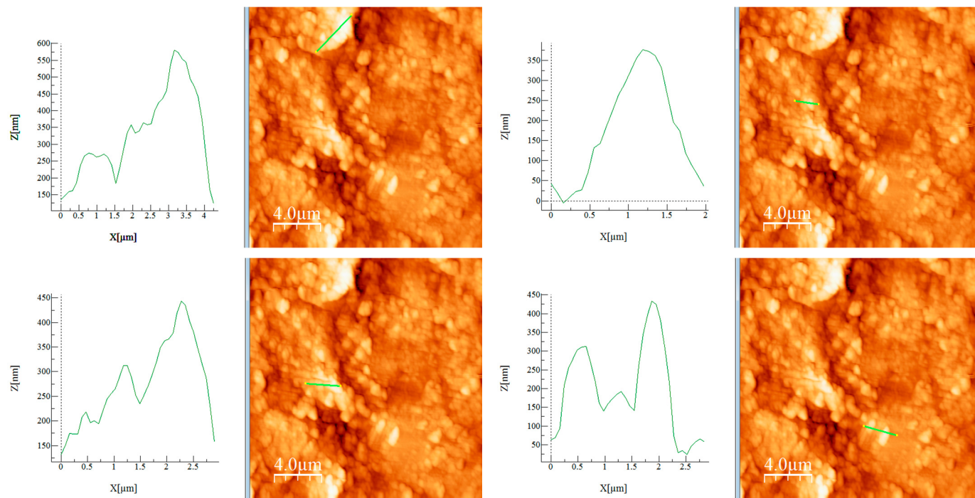
Figure 7. Surface profile of selected areas of sample S1.
