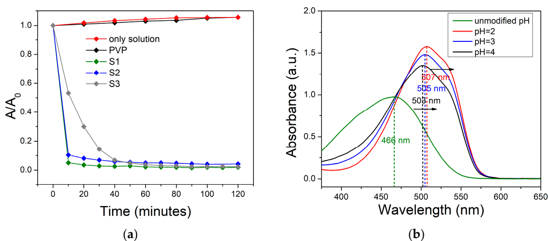
Figure 10. (a) Time-dependent degradation ratio ( A/A_0 ) illustrated at pH = 2 for reference test and for each test material (S1, S2, and S3); (b) representation of peak shape changes for absorbance of MO solution before pH adjustment and at pH = 2, pH = 3, and pH = 4.
