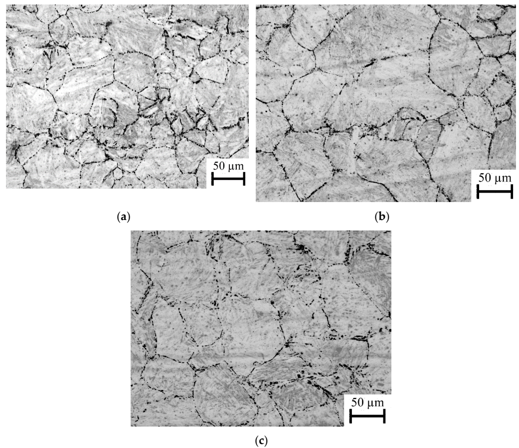
Figure 10. Optical investigated microstructures of SRX at a strain rate of 0.8 \text{ s}^{-1} , a deformation temperature of 1000^\circ\text{C} , and a prestrain of (a) 0.01, (b) 0.03, and (c) 0.05 after stress relaxation tests for 22MnB5 boron–manganese steel.
