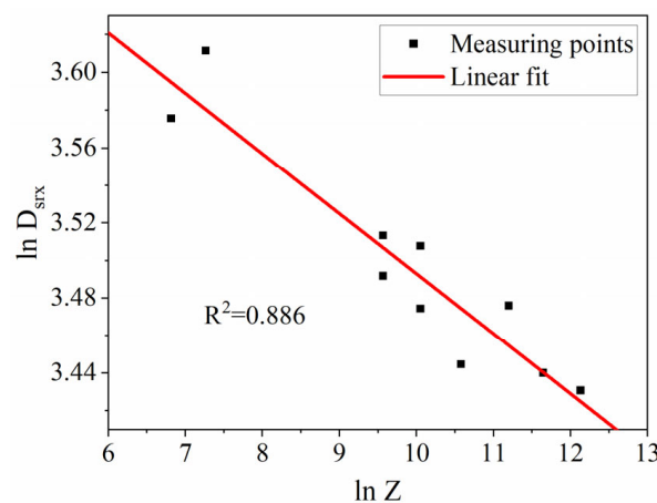
Figure 11. Relation of \ln Z and \ln D_{\text{srX}} for SRX of 22MnB5 steel.
