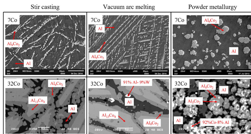
Figure 2. SEM images (backscattered electron mode) for Al-7 wt % Co (7Co) and Al-32 wt % Co (32Co) fabricated by stir casting, vacuum arc melting and powder metallurgy (Reprinted with permission from [34,72]. Copyright 2022, Elsevier).
