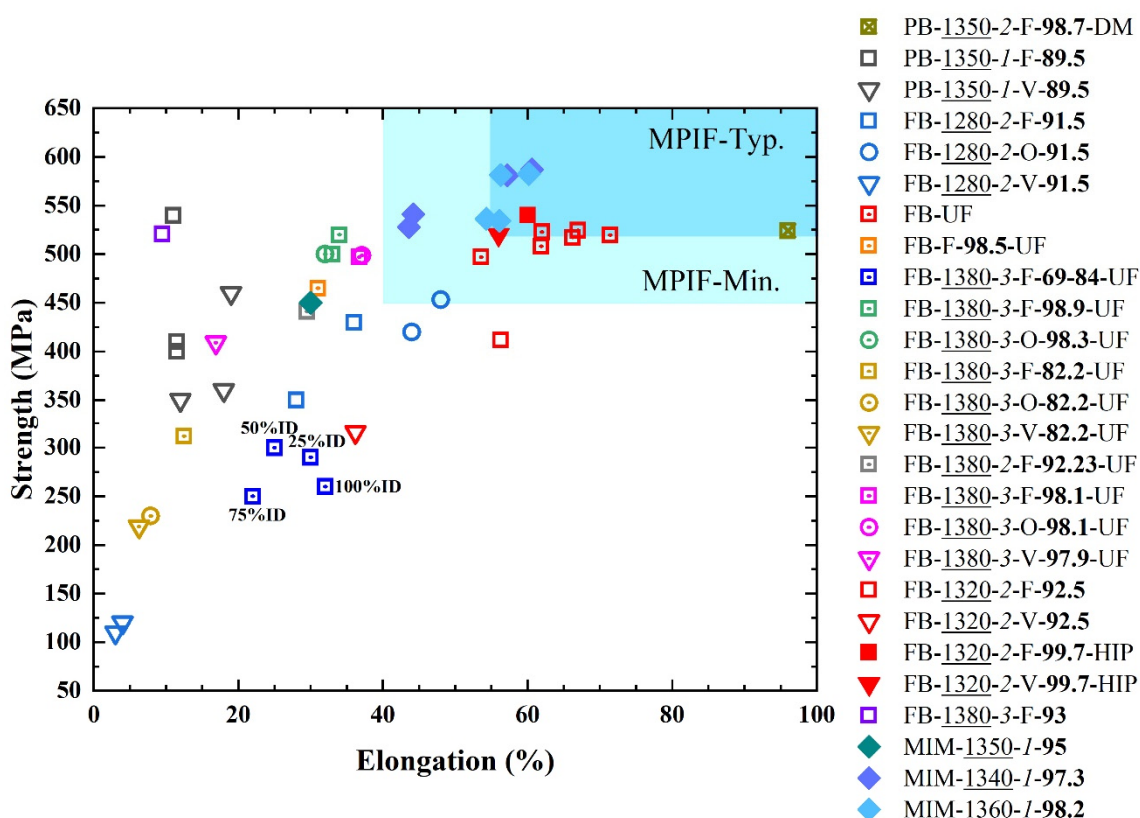
Figure 23. Stress vs. elongation map of 316L stainless steel fabricated by the metal MEX process with different conditions comparing with MPIF standard 35 for MIM materials. The underlined number represents sintering temperature (°C) and the italic number represents sintering time (h). F, O and V represent flat, on-edge and vertical printing orientations, respectively, and the bold number represents relative sintered density (%). ##% ID is the infill density. DM is utilising Desktop Metal system. Data from [9,45,53,56,57,66,68,75,81,93,98,108,160,161,169,171,172].
