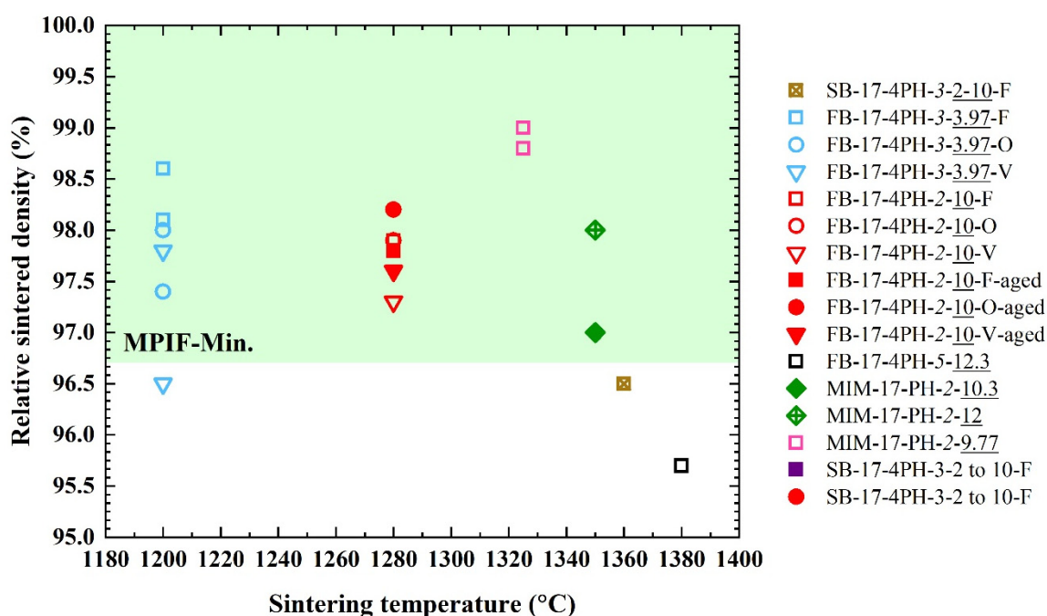
Figure 19. Sintering temperature vs. relative sintered density map of 17-4PH stainless steel fabricated by metal MEX process with different conditions comparing with MPIF standard 35 for MIM materials. The italic number represents sintering time (h) and the underlined number represents powder size ( \mu\text{m} ). F, O and V represent flat, on-edge and vertical printing orientations, respectively Data from [8,49,64,92,110,134,157,169].
