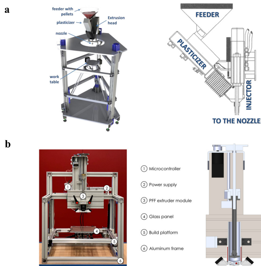
Figure 5. (a) In-house developed machine and their components with the extrusion unit combining a screw-based (plasticiser) to feed the feedstock and plunger system to inject the feedstock through the nozzle (adapted from [36]) and (b) in-house developed plunger-based printer and their components with the schematic of the extruder unit (Reprinted with permission from [61]. Copyright 2020, Additive Manufacturing, Elsevier).
