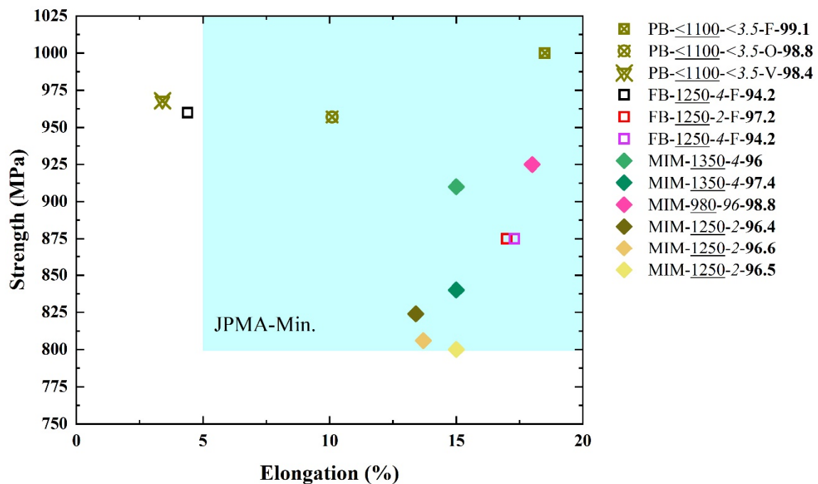
Figure 24. Stress vs. elongation map of Ti-6Al-4V alloy fabricated by the metal MEX process with different conditions comparing with JPMA standard for MIM materials. The underlined number is sintering temperature (°C), the italic number is sintering time (h) and the bold number is relative sintered density (%). Data from [78,79,109,163,164,170].
