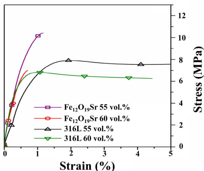
Figure 8. Tensile curves of and \text{Fe}_{12}\text{O}_{19}\text{Sr} and 316L filament with different solid loading, showing the reduction in strain with 5% increment of solid loading (adapted from [4]).
