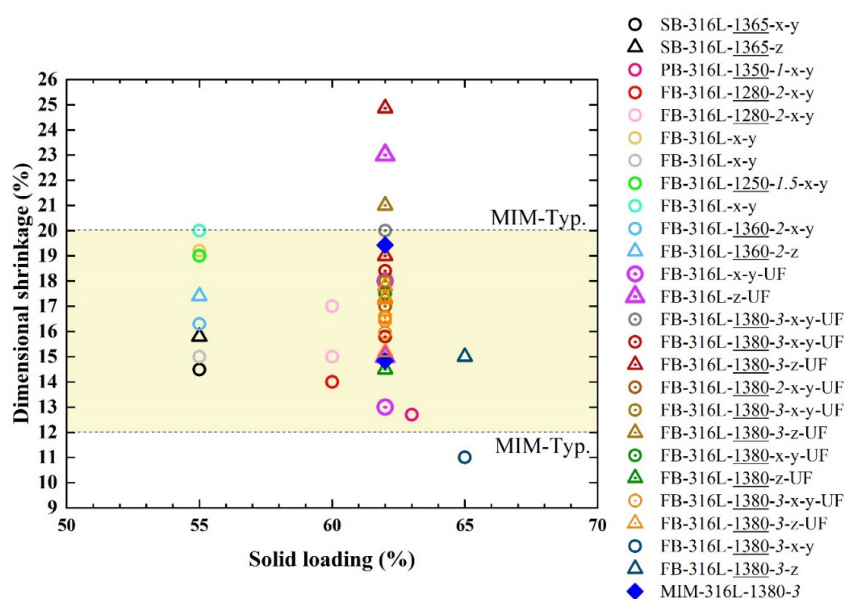
Figure 16. Solid loading vs. dimensional shrinkage map of 316L stainless steel fabricated by the metal MEX process with different conditions comparing with typical MIM. The underlined number
