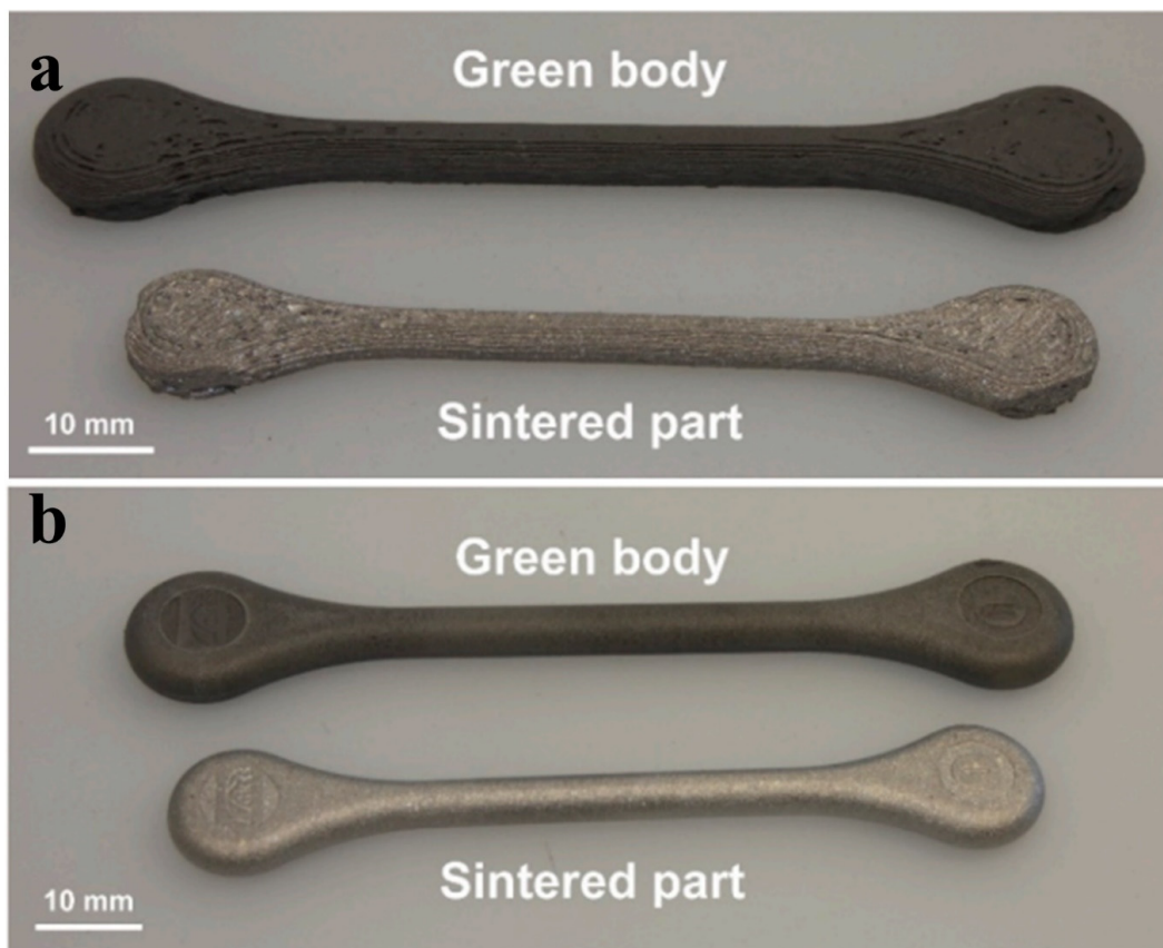
Figure 12. As-printed and as-sintered Ti-6Al-4V specimens fabricated by (a) metal MEX process and (b) MIM process, demonstrating the difference in sizes due to shrinkage upon sintering (adapted from [91]).
