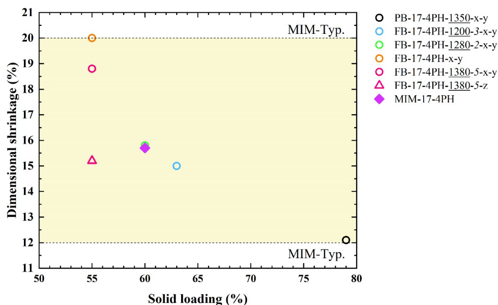
Figure 15. Solid loading vs. dimensional shrinkage map of 17-4PH stainless steel fabricated by metal MEX process with different conditions compared with typical MIM. The underlined number represents sintering temperature ( ^{\circ}\text{C} ); the italic number represents sintering time (h); and x-y (average from length and width) or z (thickness) indicate the direction of shrinkage measurement. Data from [8,36,44,49,64,127,158].
