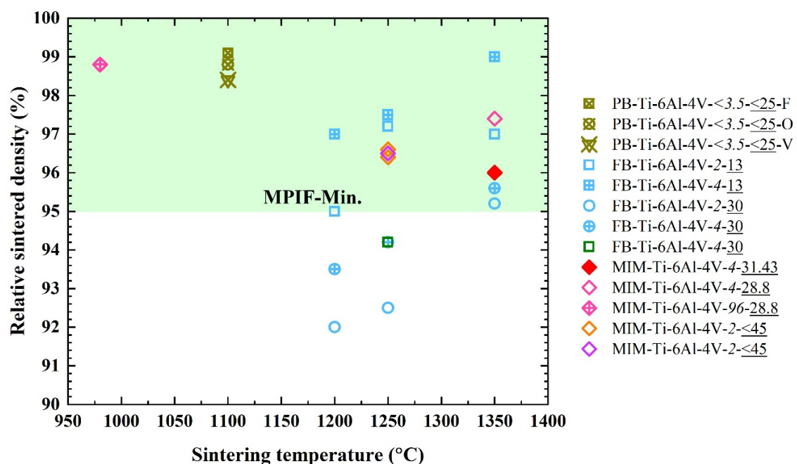
Figure 21. Sintering temperature vs. relative sintered density map of Ti-6Al-4V alloys fabricated by metal MEX process with different conditions comparing with MPIF standard 35 for MIM materials. The italic number represents sintering time (h) and the underlined number represents mean powder size ( \mu\text{m} ). Data from [78,79,109,163,164,170–172].
