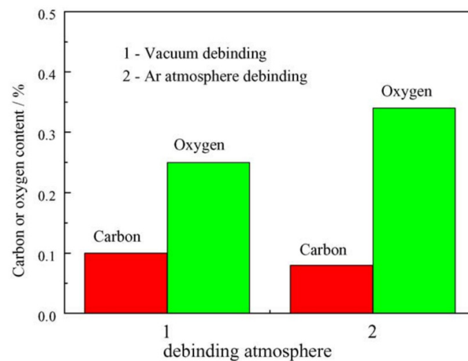
Figure 11. Effect of debinding atmosphere on the C and O uptake during debinding of Ti-6Al-4V MIM (Reprinted with permission from [179]. Copyright 2006, Journal of Materials Processing Technology, Elsevier).
