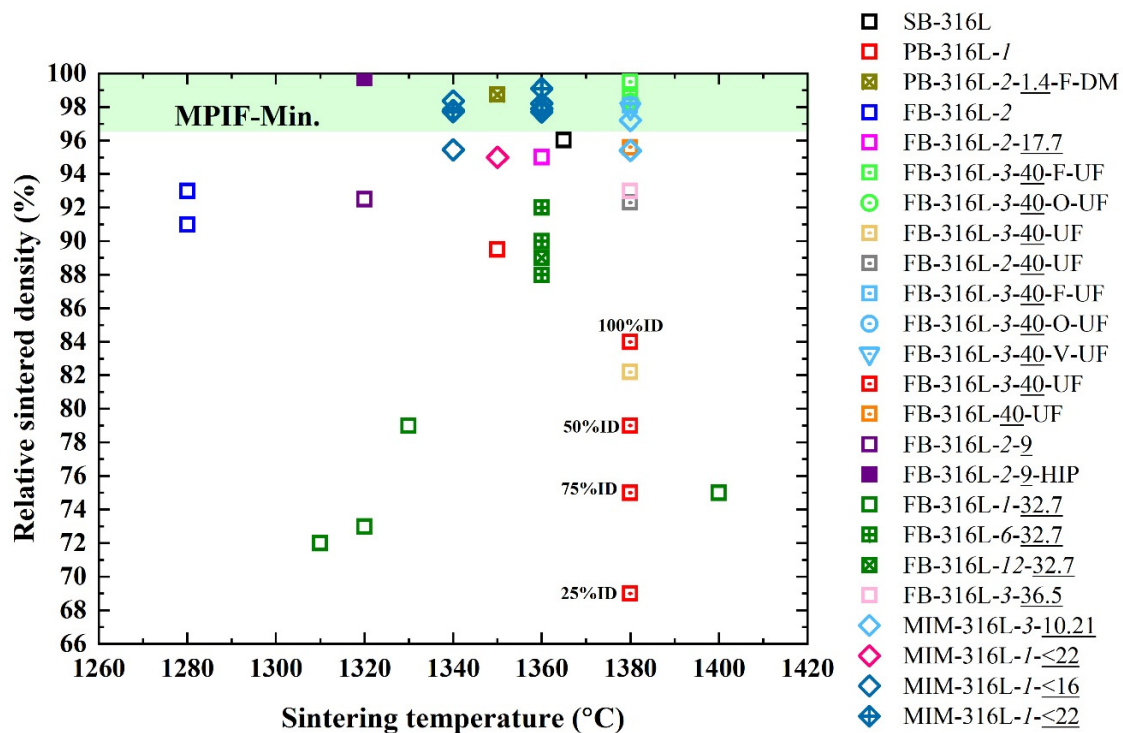
Figure 20. Sintering temperature vs. relative sintered density map of 316L stainless steel fabricated by metal MEX process with different conditions comparing with MPIF standard 35 for MIM materials. The Italic number represents sintering time (h) and the underlined number represents powder size ( \mu\text{m} ). F, O and V represent flat, on-edge and vertical printing orientations, respectively. ##%ID is the infill density. DM is utilising Desktop Metal system. Data from [9,41,45,52,53,56,57,66,68,70,72,75,81,98,108,159–161,169].
