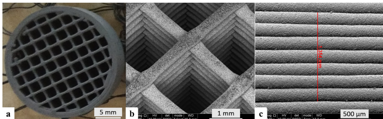
Figure 9. An as-printed part fabricated by metal MEX process, using an in-house developed 316L filament: (a) overview of the as-printed part, (b) top view and (c) side view (adapted from [83]).
