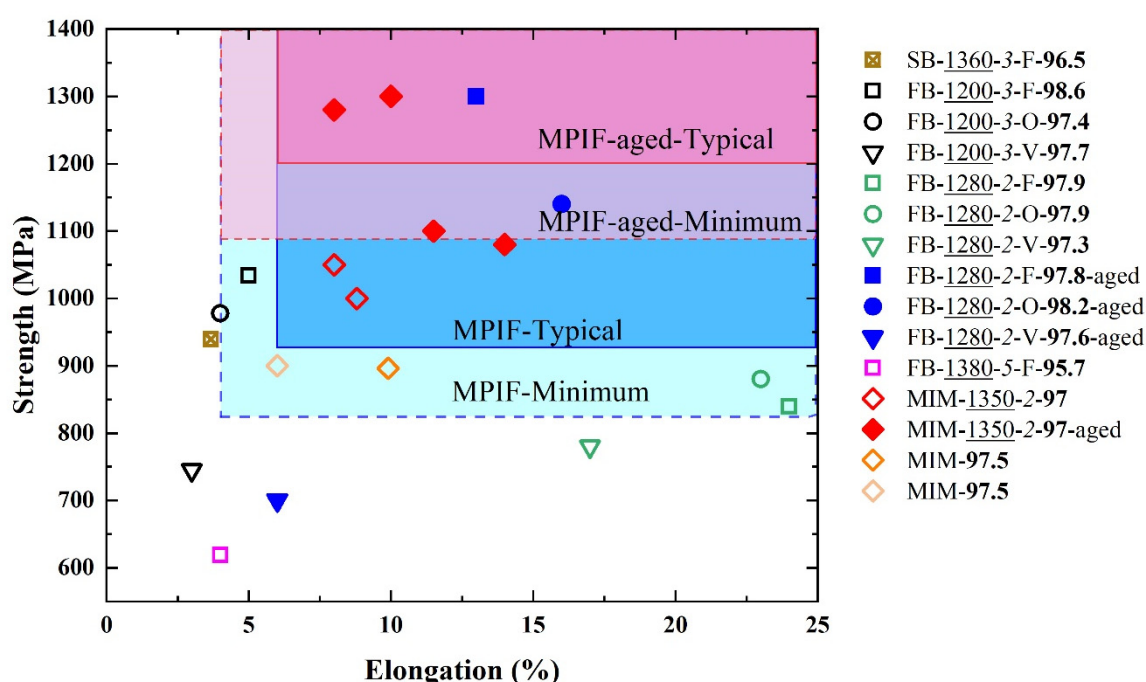
Figure 22. Stress vs. elongation map of 17-4PH stainless steel fabricated by the metal MEX process with different conditions comparing MPIF standard 35 for MIM materials. The underlined number represents sintering temperature (°C), the italic number represents sintering time (h), F, O and V represent flat, on-edge and vertical printing orientations, respectively, and the bold number represents relative sintered density (%). Data from [8,49,64,92,134,157,158,169].
