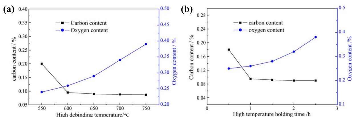
Figure 10. C and O uptake during debinding as a function of (a) debinding temperature and (b) sintering (holding) time during debinding of Ti-6Al-4V MIM (Reprinted with permission from [179]. Copyright 2006, Journal of Materials Processing Technology, Elsevier).
