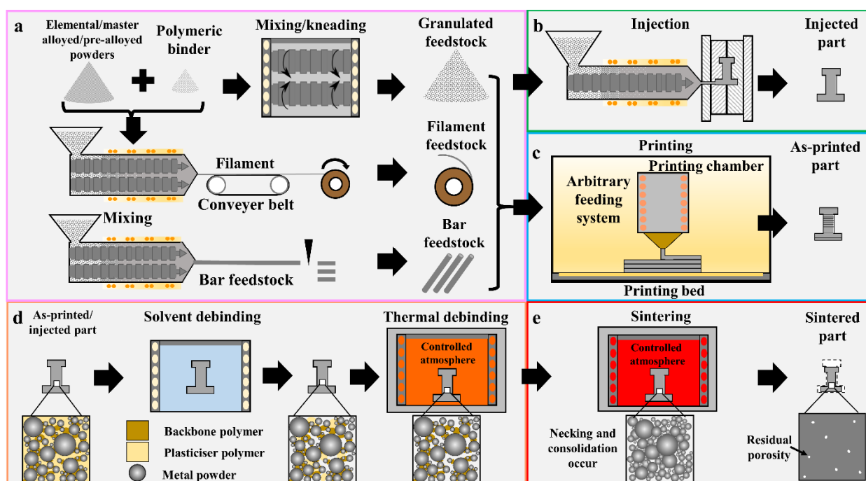
Figure 2. Comparison of material extrusion additive manufacturing of metal (a,c,d,e) and metal injection moulding (a,b,d,e).
