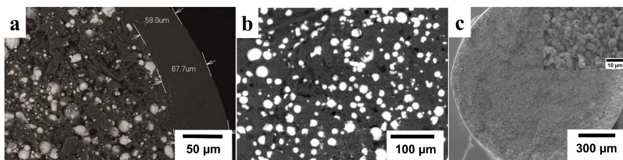
Figure 6. Cross-sectional view of the commercial filaments—(a) Ultrafuse by BASF (adapted from [4]), showing polymer skin surrounding mixing of polymer and metal powder, (b) 316L metal filament by Virtual foundry (adapted from [72]) and (c) 17-4PH stainless steel filament for MetalX system by Markforged, Inc. (Reprinted with permission from ref. [8]. Copyright 2021, Metallurgical and Materials Transactions A, Springer).
