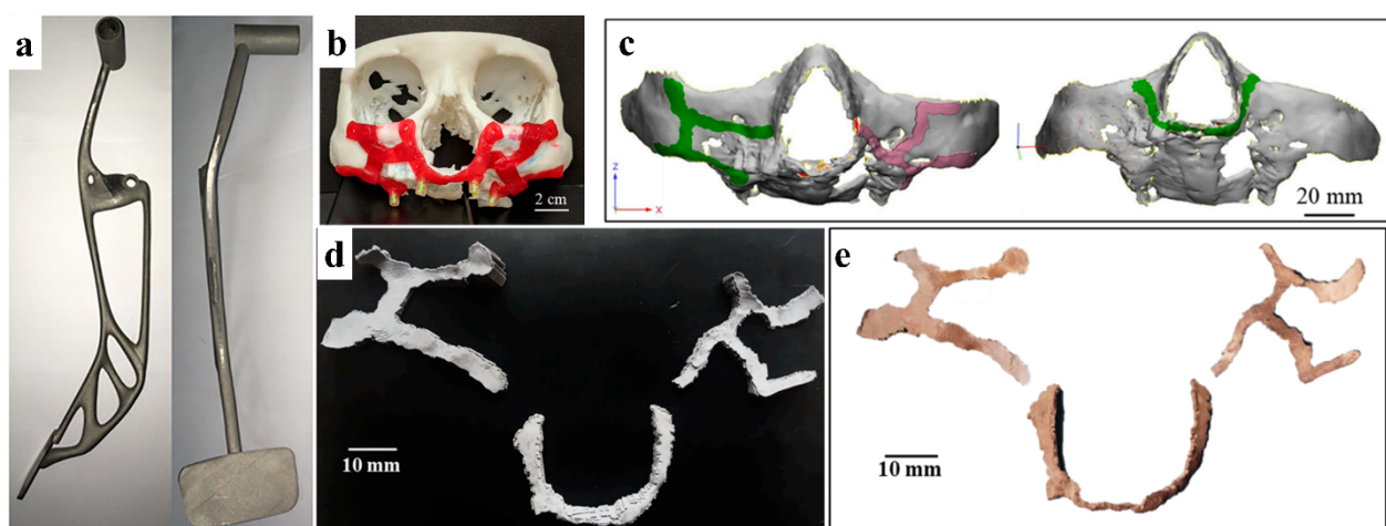
Figure 25. (a) 316L MEX brake pedal (Reprinted with permission from ref. [141]. Copyright 2021, Materials Today: Proceedings, Elsevier) and (b) maxillofacial implant design, (c) maxillofacial implants related to the design, (d) as-printed parts following the design and (e) as-sintered parts (adapted from [95]).
