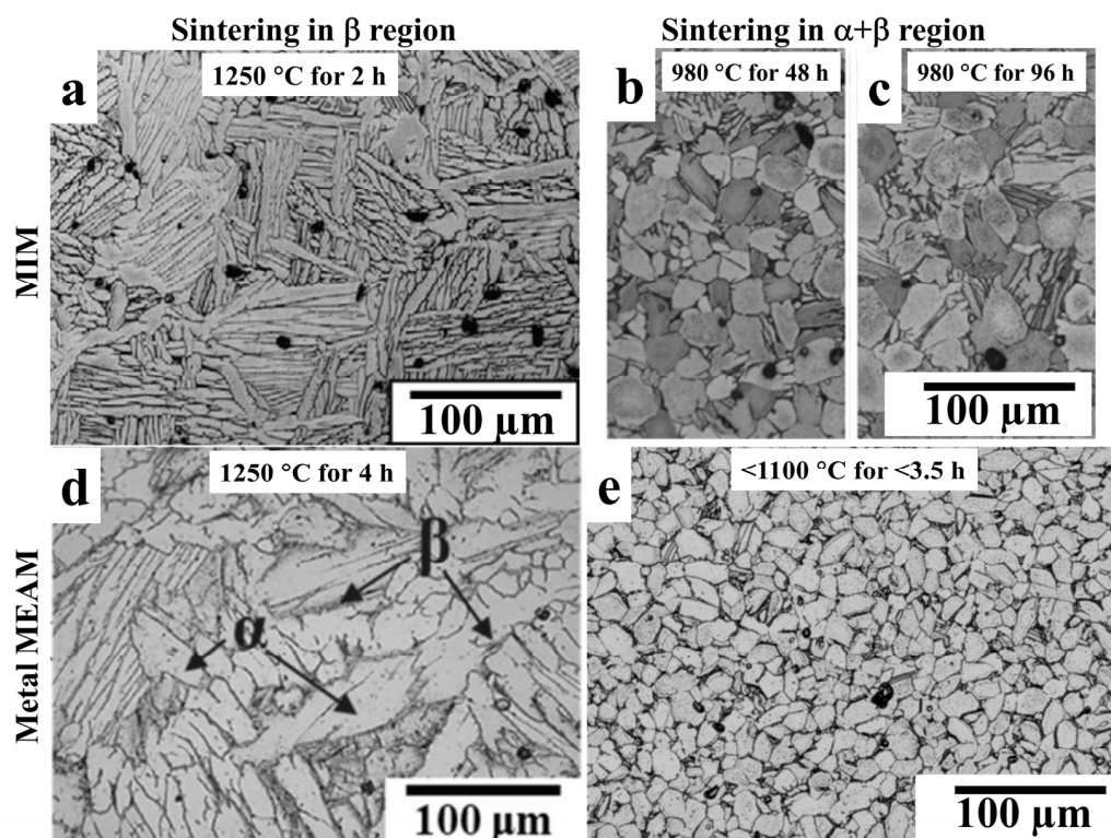
Figure 14. Microstructure comparison of Ti-6Al-4V parts (a) fabricated by MIM process sintered in the \beta region (Reprinted with permission from [171]. Copyright 2009, Materials Science and Engineering: A, Elsevier), (b,c) fabricated by MIM process sintered in the \alpha + \beta region (adapted from [163]), (d) fabricated by metal MEX process sintered in the \beta region (Reprinted with permission from [78]. Copyright 2021, Powder Technology, Elsevier). and (e) fabricated by metal MEX process sintered in the \alpha + \beta region for grain refinement (adapted from [109]).
