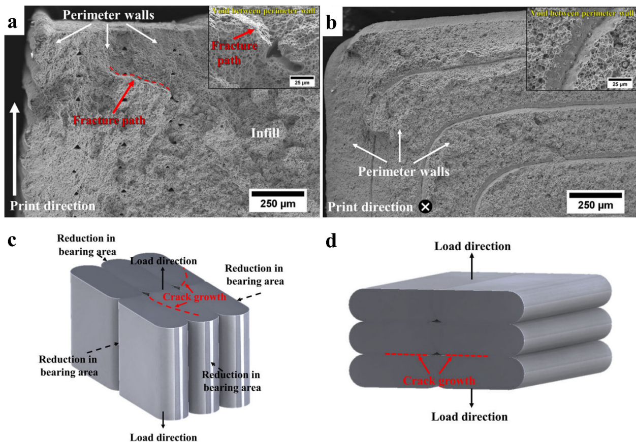
Figure 18. Fracture surface of metal MEX 17-4PH stainless steel specimens built with the (a) flat, (b) vertical orientations and schematics showing the failure mechanism of specimen built with the (c) flat and (d) vertical orientations (Reprinted with permission from [8]. Copyright 2021, Metallurgical and Materials Transactions A, Springer).
