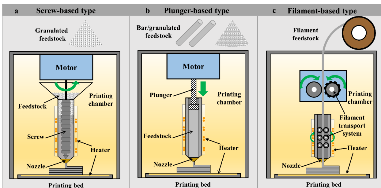
Figure 3. Types of material extrusion additive manufacturing classified by feeding system: (a) screw-based, (b) plunger-based and (c) filament-based types.
