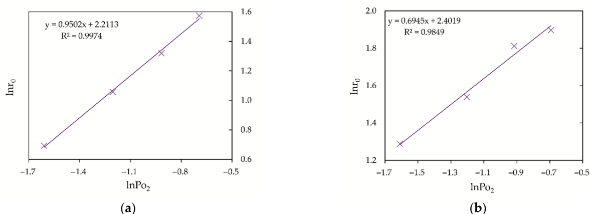
Figure 10. Dependence of \ln r_0 on \ln P_{O_2} without (a) and with (b) Cu (II).
