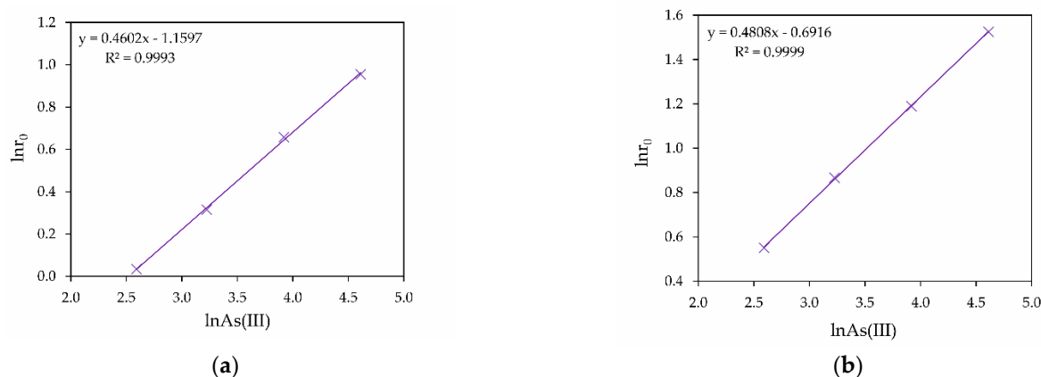
Figure 11. Dependences of \ln r_0 on \ln As(III) without (a) and with (b) Cu (II).
